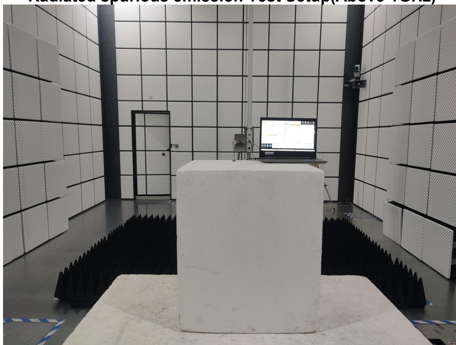
Radiated spurious emission Test Setup(Above 1GHz)
