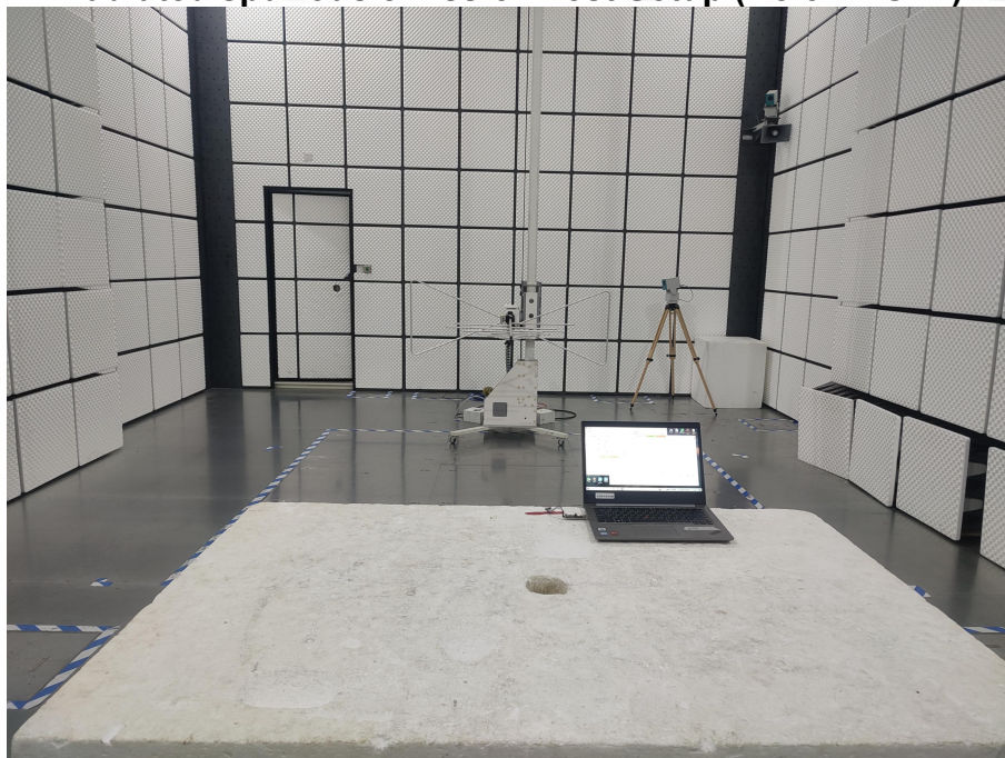
Radiated spurious emission Test Setup (Below 1GHz)
