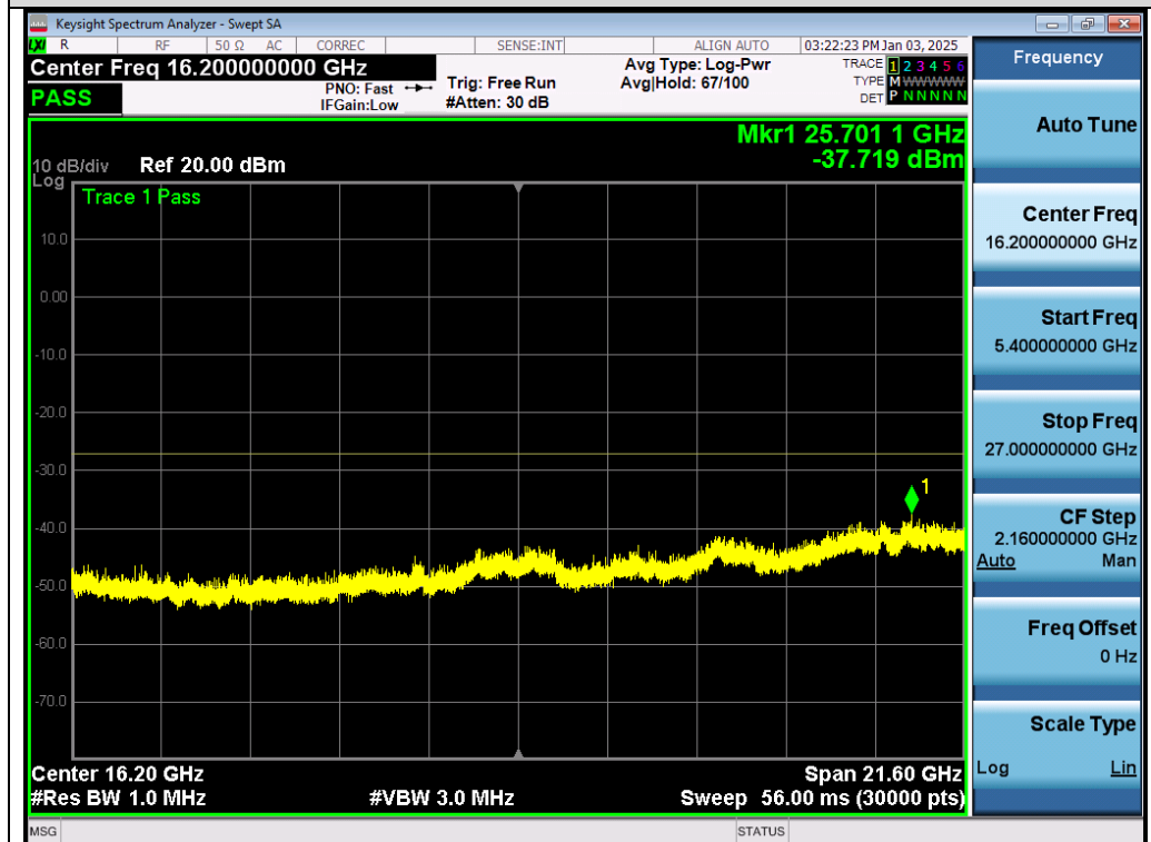
Test_Graph_802.11n40_ANT1_5190_MCS0_Frequency Band 4
