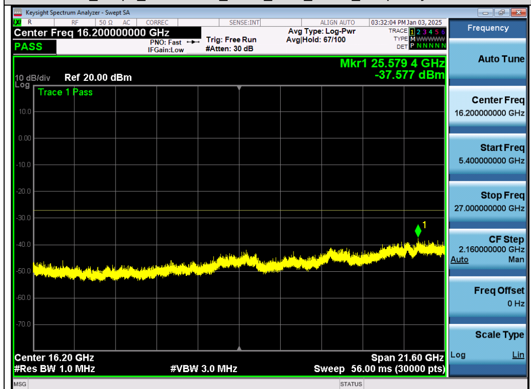
Test Graph 802.11ac80 ANT1 5210 MCS0 Frequency Band 4
