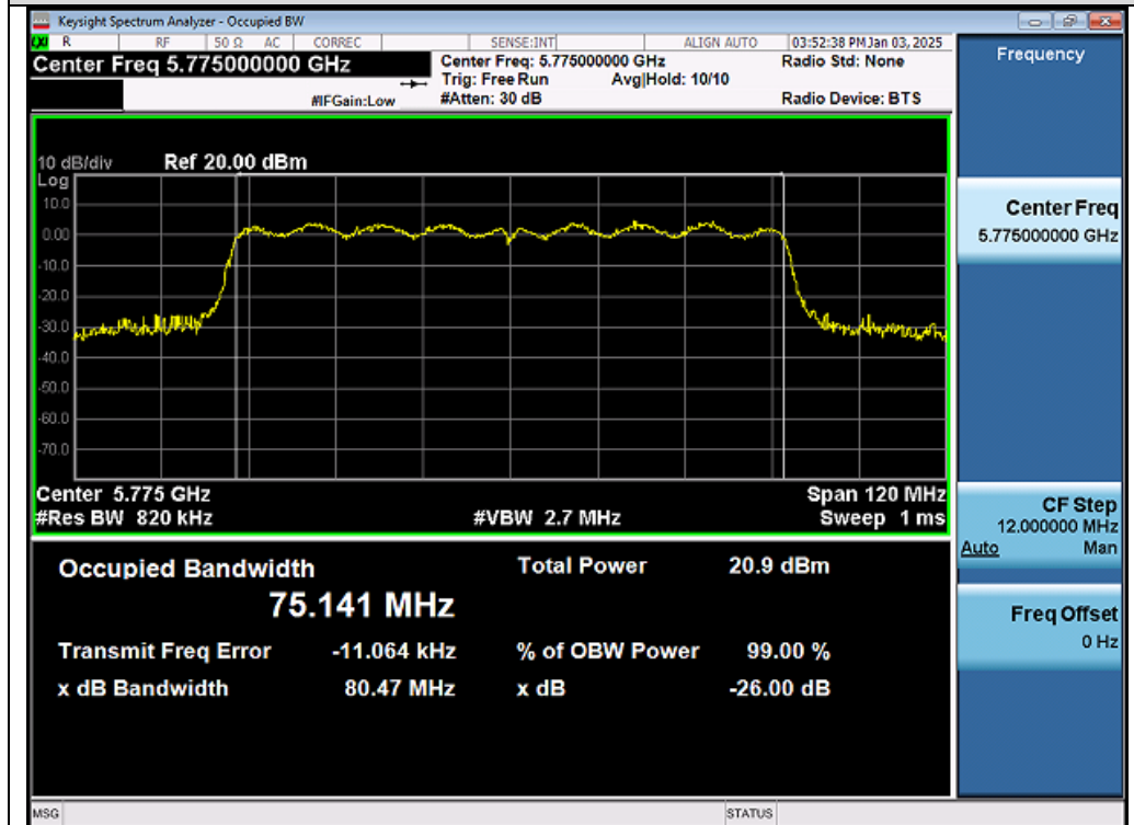
Test_Graph_802.11ac80_ANT1_5775_MCS0_OBW
