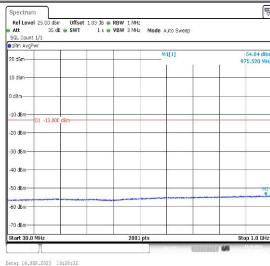
Band2-9262-2-30~1000MHz-PASS
