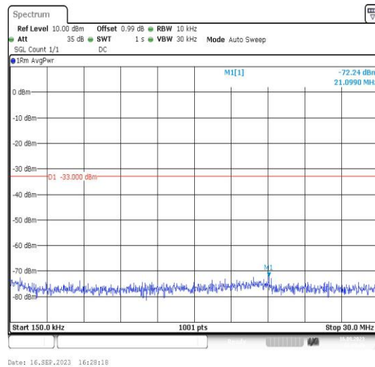
Band2-9262-2-0.15~30MHz-PASS
