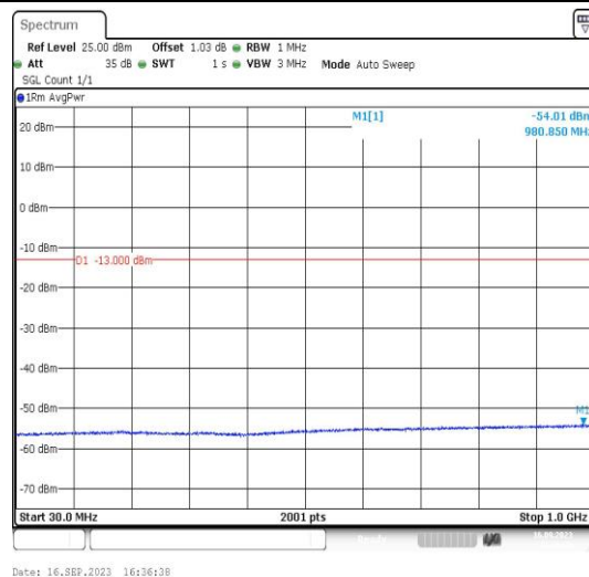
Band2-9538-4-30~1000MHz-PASS
