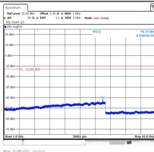
Band5-4233-4-1000~10000MHz-PASS
