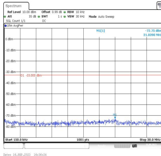
Band2-9538-4-0.15~30MHz-PASS
