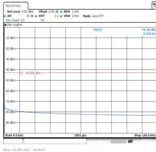
Band2-9262-2-0.009~0.15MHz-PASS
