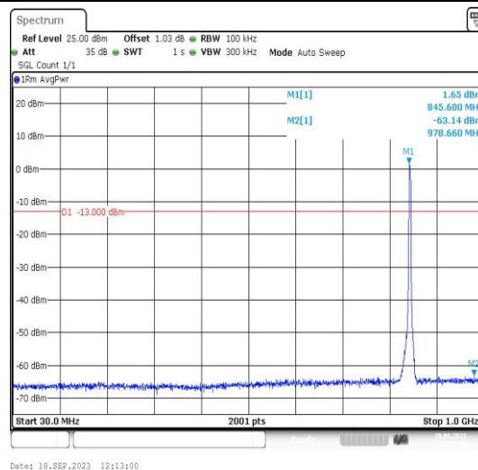
Band5-4233-4-30~1000MHz-PASS
