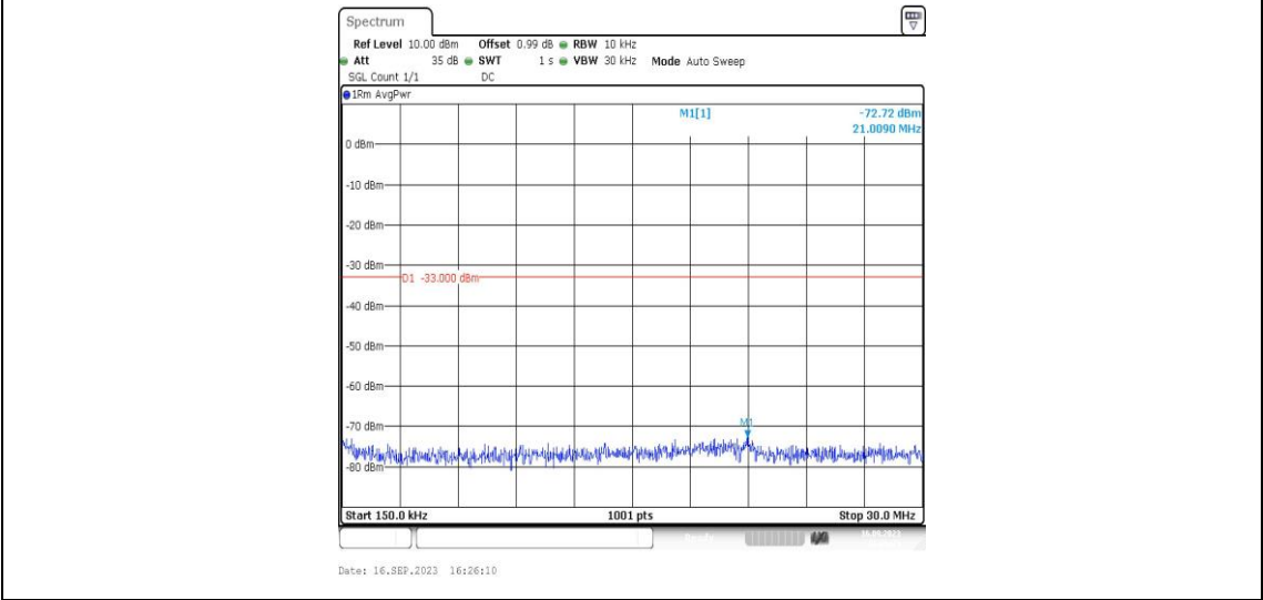
Band2-9400-1-0.15~30MHz-PASS
