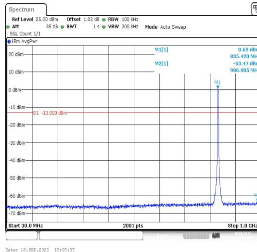
Band5-4182-2-30~1000MHz-PASS
