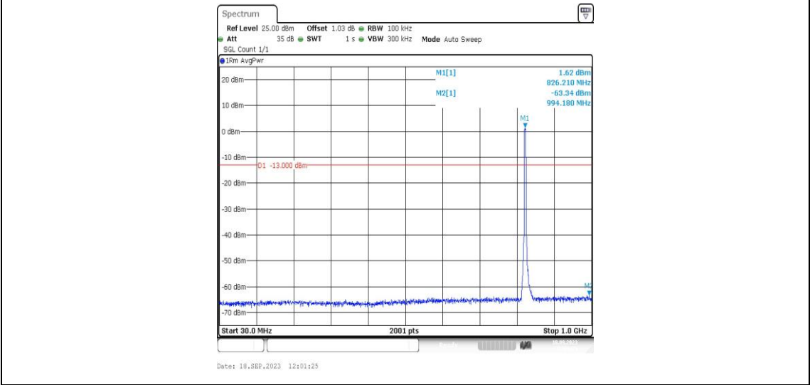
Band5-4132-1-30~1000MHz-PASS
