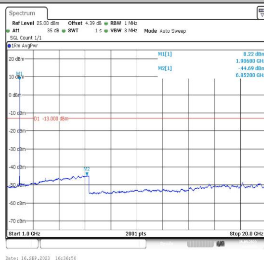
Band2-9538-4-1000~20000MHz-PASS
