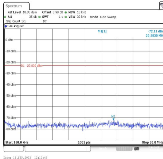
Band5-4233-4-0.15~30MHz-PASS
