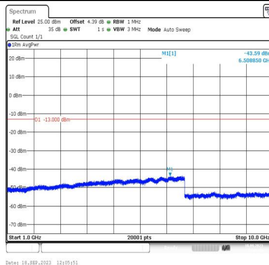
Band5-4182-2-1000~10000MHz-PASS
