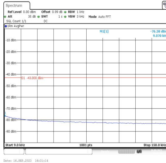
Band2-9262-3-0.009~0.15MHz-PASS
