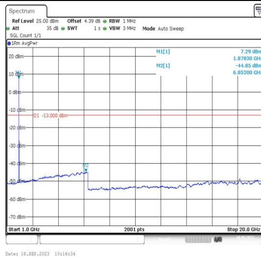
Band2-9400-2-1000~20000MHz-PASS
