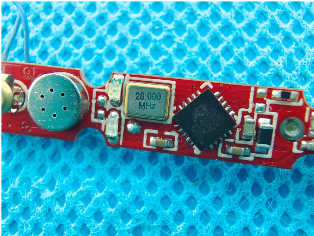
Right ear Chip
