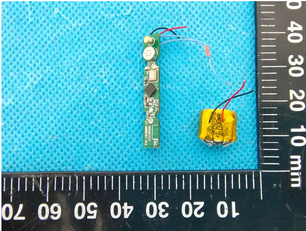
Left ear Battery
