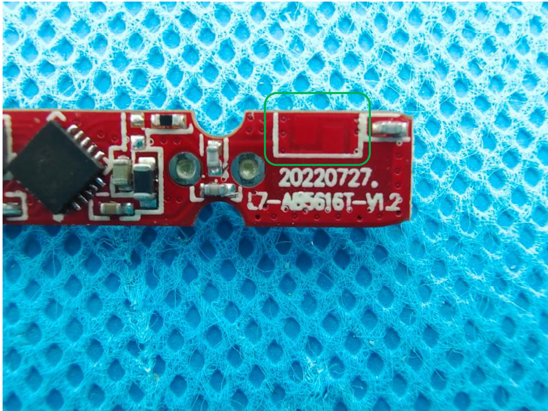
Right ear Antenna
