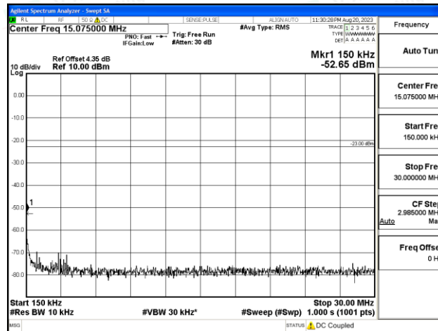
Band71_15MHz_16QAM_133297_1RB#0_0.15~30_0.15~30
