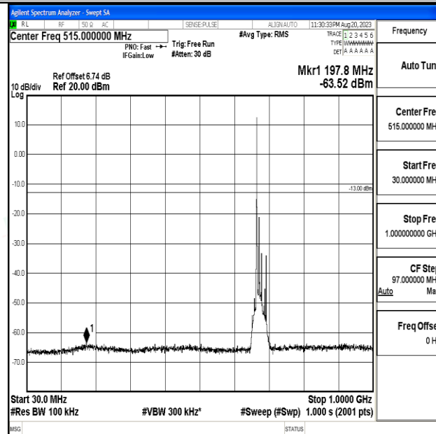
Band71_15MHz_16QAM_133297_1RB#0_30~1000_30~1000
