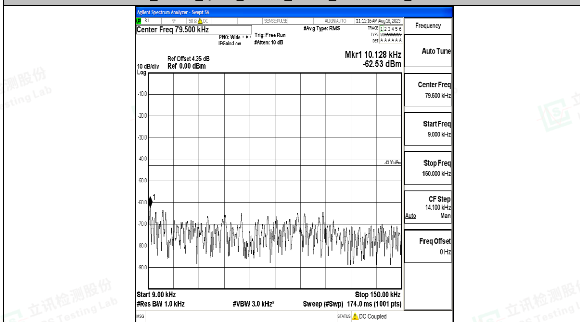
Band66_15MHz_16QAM_132597_1RB#0_0.009~0.15_0.009~0.15
