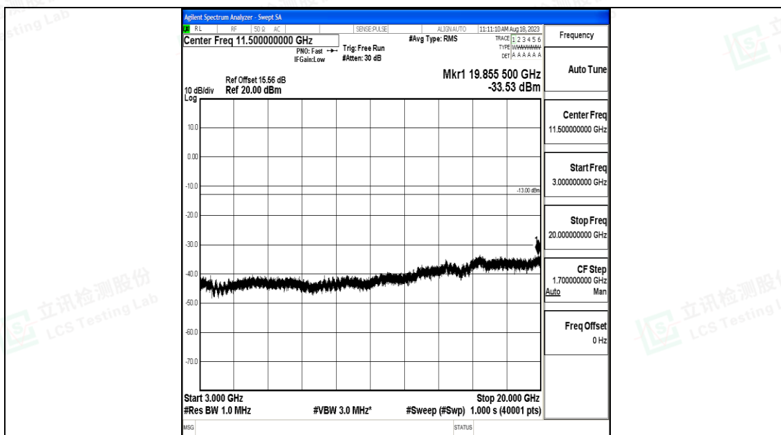
Band66_15MHz_QPSK_132597_1RB#0_3000~20000_3000~20000
