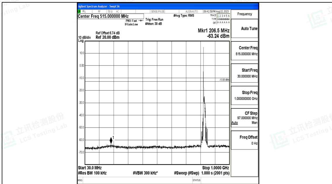
Band26_15MHz_QPSK_26865_1RB#0_30~1000_30~1000
