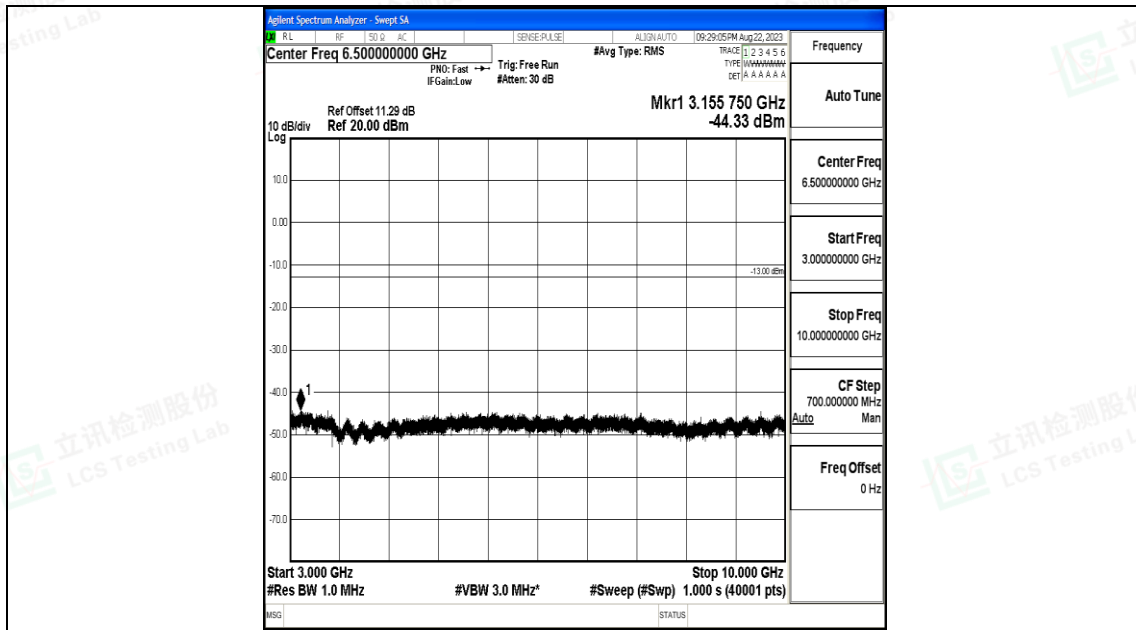
Band26_10MHz_QPSK_26840_1RB#0_3000~10000_3000~10000
