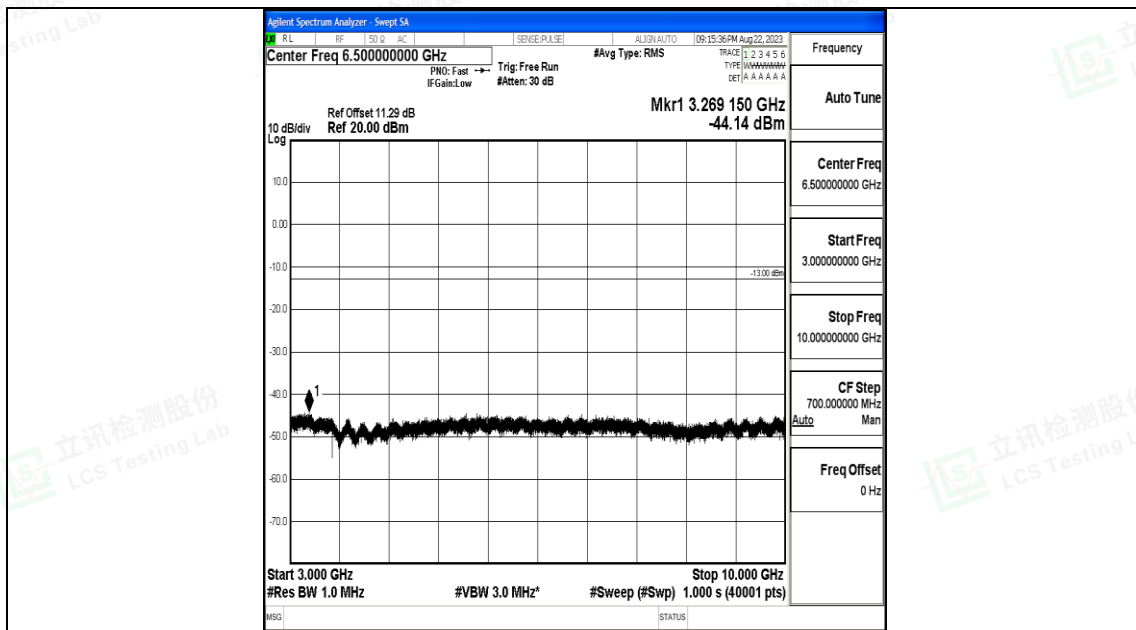
Band26_5MHz_QPSK_26815_1RB#0_3000~10000_3000~10000
