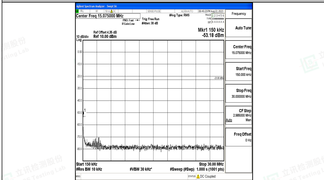
Band26_1.4MHz_QPSK_27033_1RB#0_0.15~30_0.15~30
