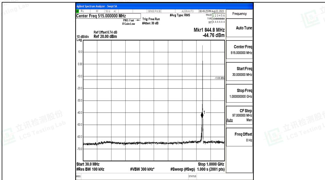
Band26_1.4MHz_QPSK_27033_1RB#0_30~1000_30~1000
