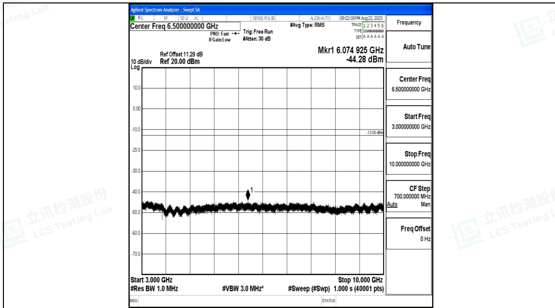
Band26_3MHz_QPSK_26915_1RB#0_3000~10000_3000~10000
