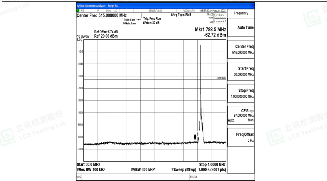
Band5_10MHz_16QAM_20450_1RB#0_30~1000_30~1000
