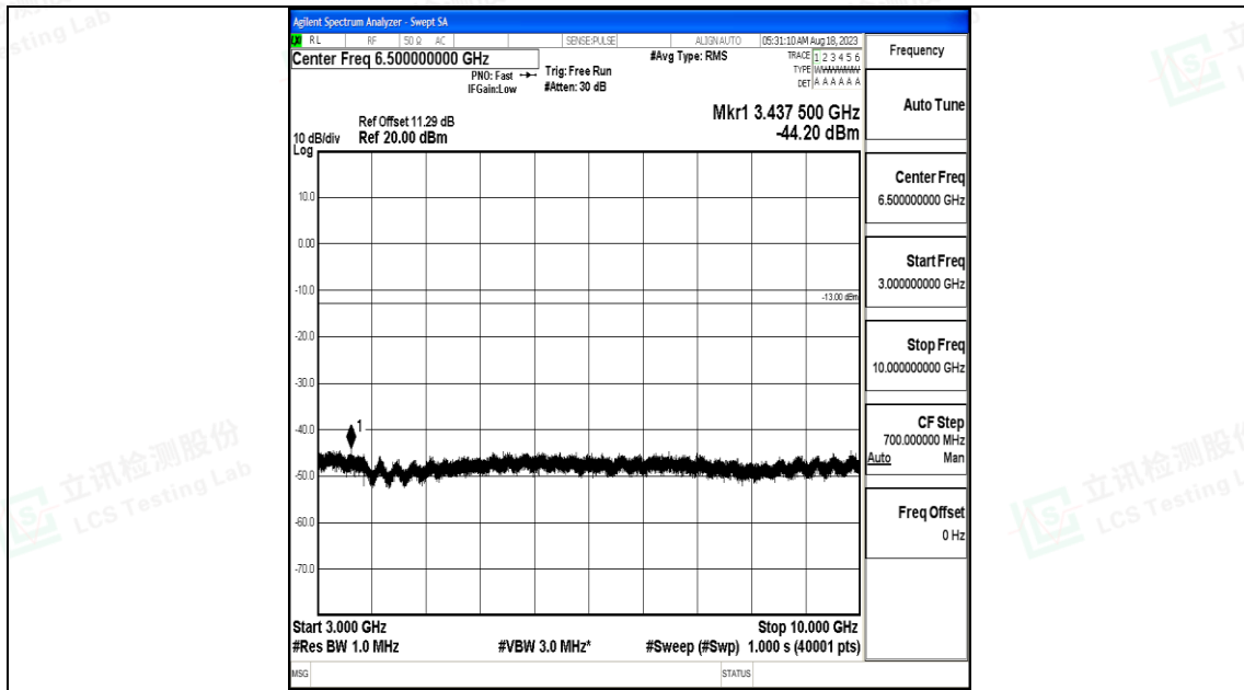
Band5_3MHz_16QAM_20525_1RB#0_3000~10000_3000~10000
