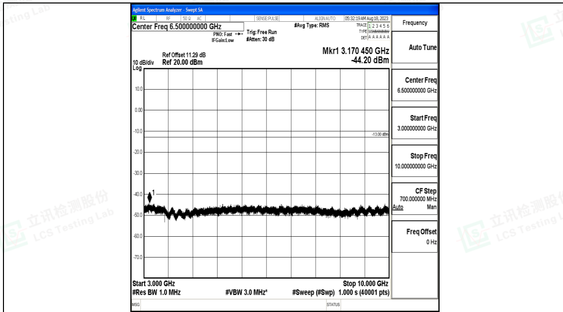
Band5_3MHz_16QAM_20635_1RB#0_3000~10000_3000~10000
