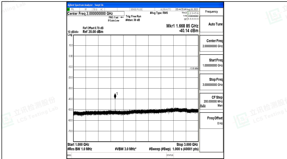
Band5_5MHz_QPSK_20525_1RB#0_1000~3000_1000~3000
