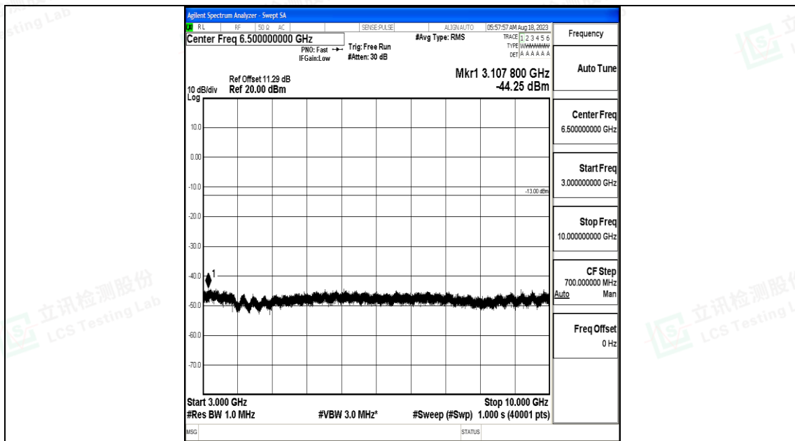
Band5_10MHz_16QAM_20450_1RB#0_3000~10000_3000~10000
