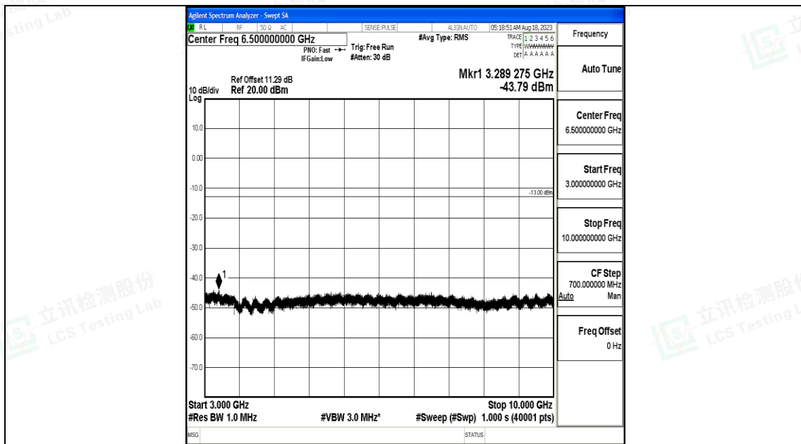
Band5_1.4MHz_16QAM_20643_1RB#0_3000~10000_3000~10000
