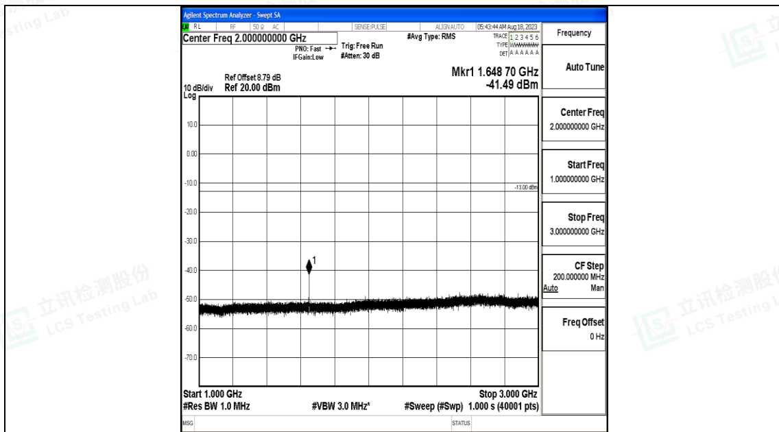
Band5_5MHz_QPSK_20425_1RB#0_1000~3000_1000~3000
