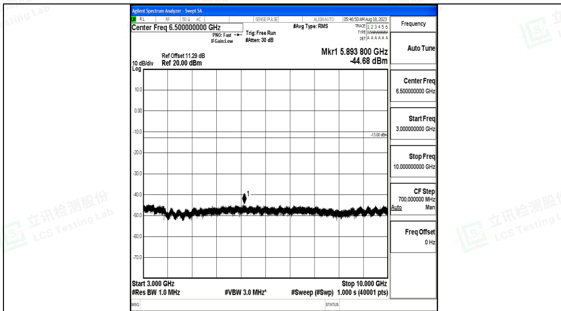
Band5_5MHz_16QAM_20625_1RB#0_3000~10000_3000~10000
