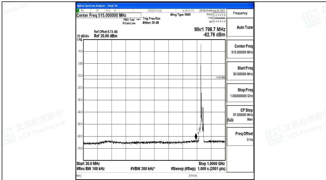
Band5_10MHz_16QAM_20525_1RB#0_30~1000_30~1000
