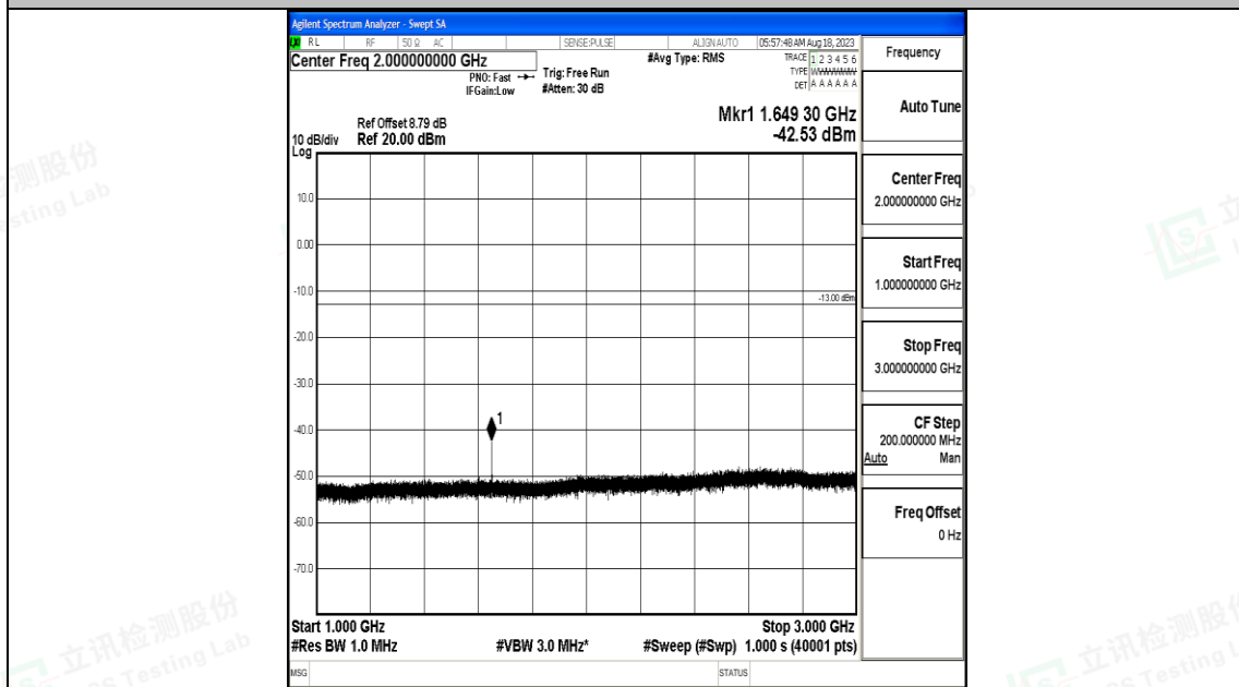
Band5_10MHz_16QAM_20450_1RB#0_1000~3000_1000~3000
