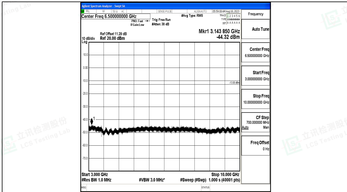
Band5_10MHz_16QAM_20525_1RB#0_3000~10000_3000~10000
