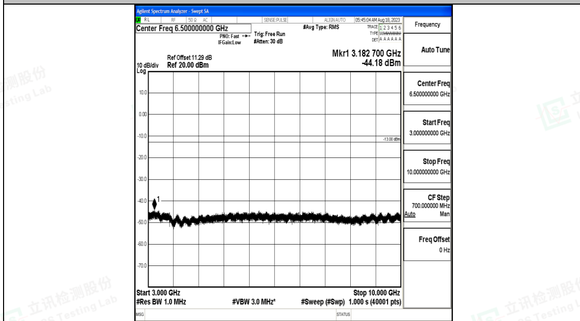
Band5_5MHz_QPSK_20525_1RB#0_3000~10000_3000~10000
