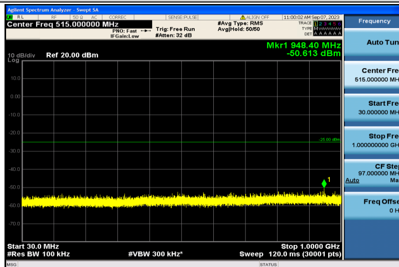
Band7-15MHz-16QAM-21375-1RB#0-30~1000MHz
