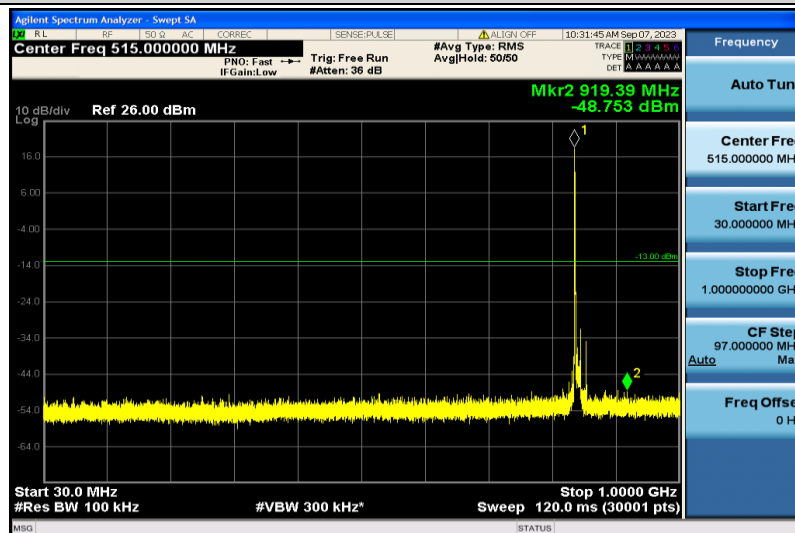
Band5-10MHz-16QAM-20600-1RB#0-30~1000MHz
