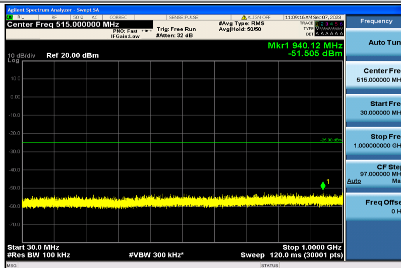
Band7-20MHz-16QAM-21350-1RB#0-30~1000MHz
