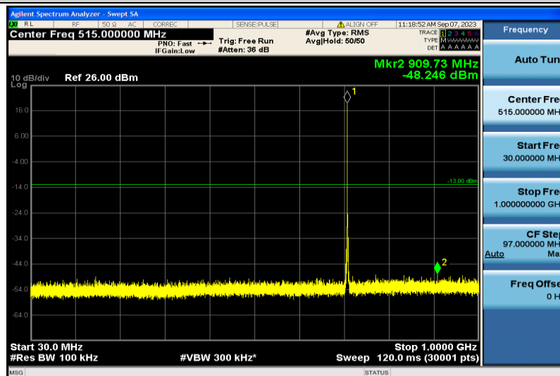
Band12-1.4MHz-QPSK-23173-1RB#0-30~1000MHz
