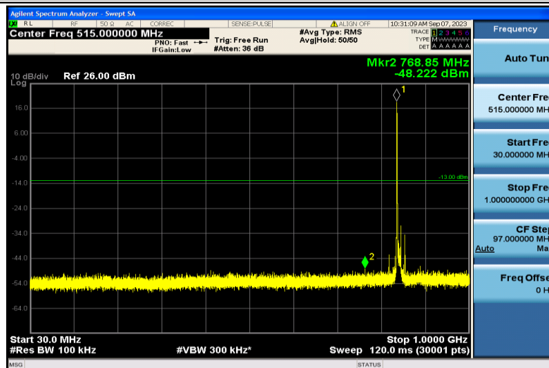
Band5-10MHz-QPSK-20600-1RB#0-30~1000MHz
