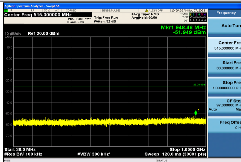
Band7-15MHz-QPSK-21375-1RB#0-30~1000MHz
