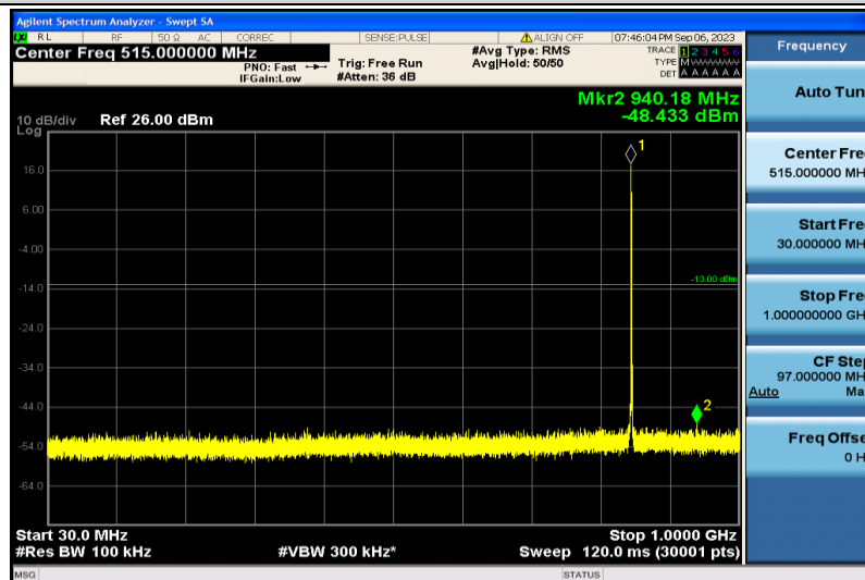
Band5-1.4MHz-16QAM-20643-1RB#0-30~1000MHz
