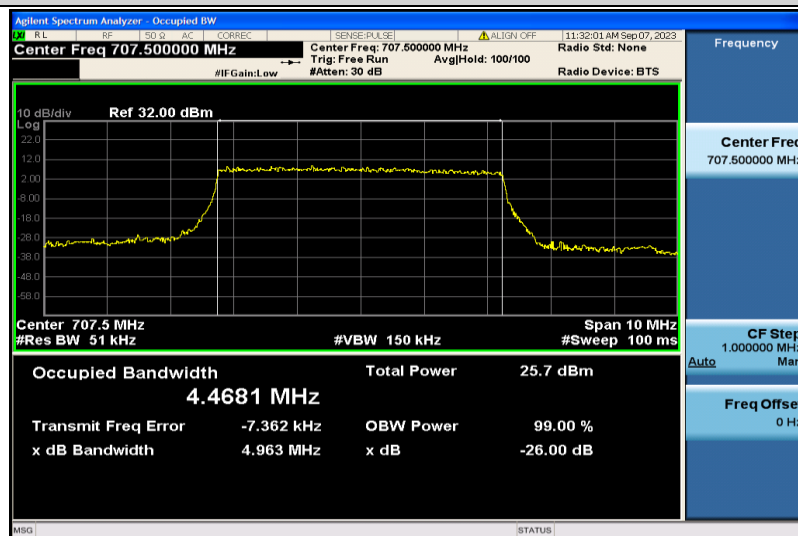
Band12-5MHz-QPSK-23095-25RB#0-4.4681
