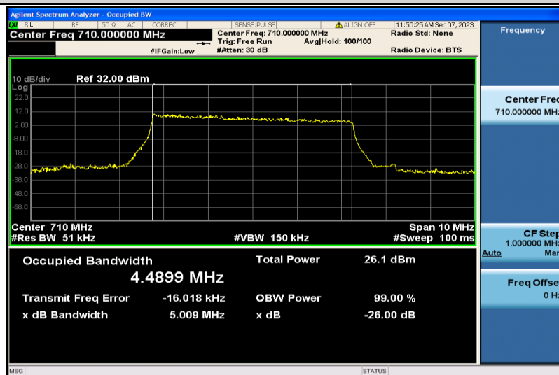
Band17-5MHz-QPSK-23790-25RB#0-4.4899
