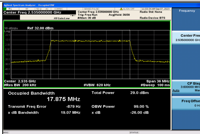
Band7-20MHz-QPSK-21100-100RB#0-17.875
