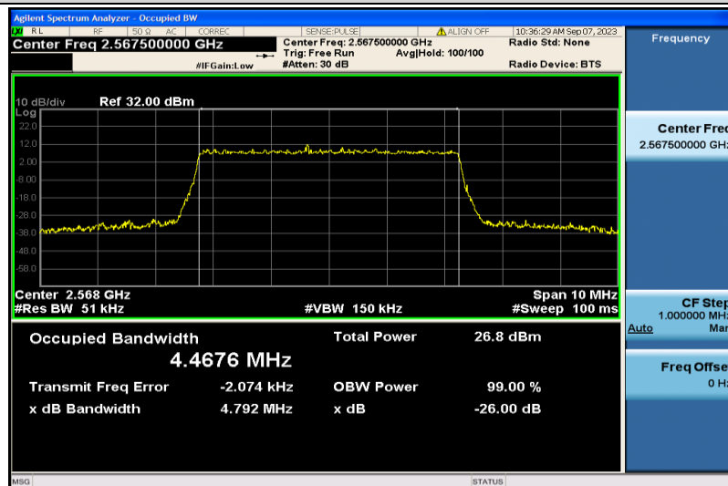
Band7-5MHz-16QAM-21425-25RB#0-4.4676
