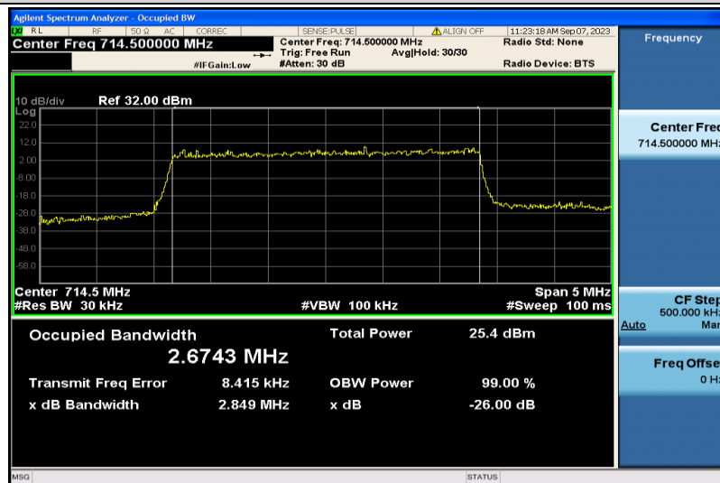
Band12-3MHz-QPSK-23165-15RB#0-2.6743
