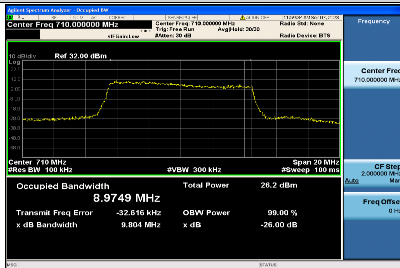
Band17-10MHz-QPSK-23790-50RB#0-8.9749
