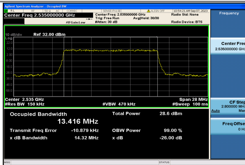
Band7-15MHz-QPSK-21100-75RB#0-13.416
