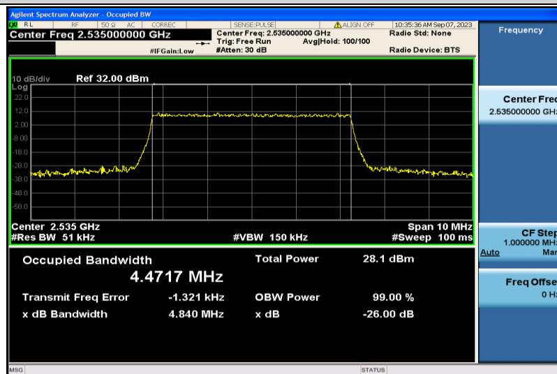
Band7-5MHz-QPSK-21100-25RB#0-4.4717
