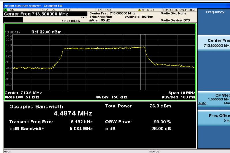
Band17-5MHz-QPSK-23825-25RB#0-4.4874
