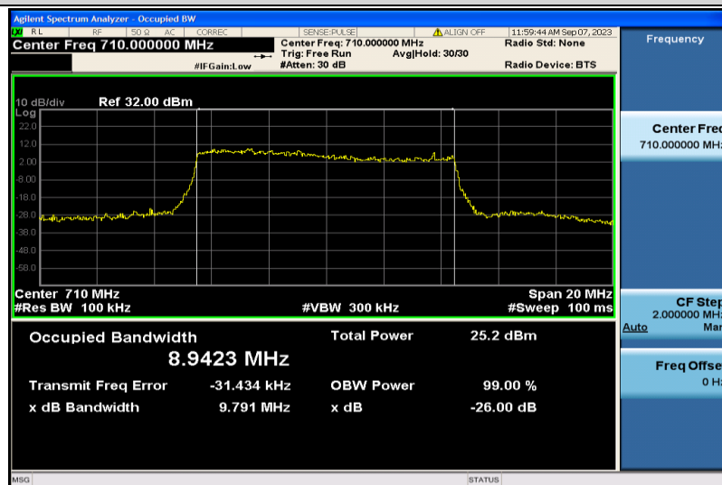
Band17-10MHz-16QAM-23790-50RB#0-8.9423
