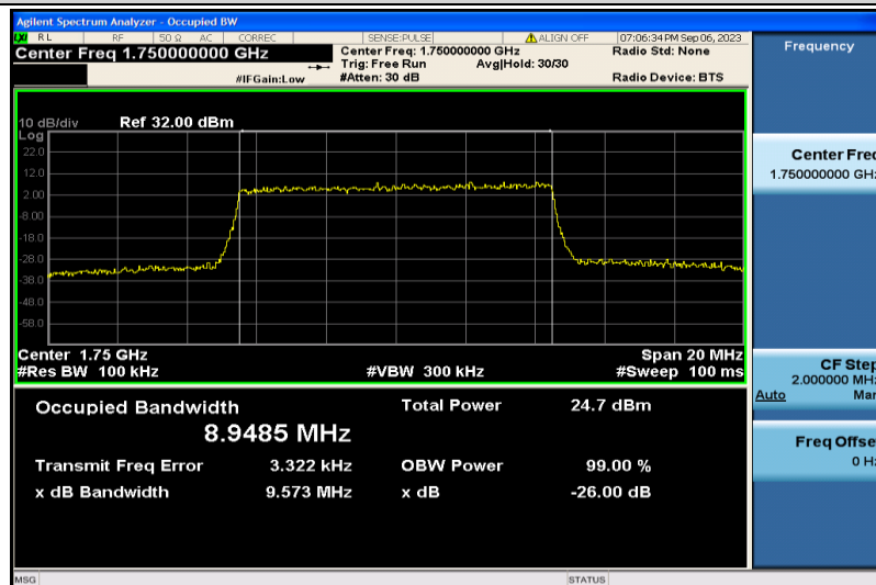
Band4-10MHz-16QAM-20350-50RB#0-8.9485
