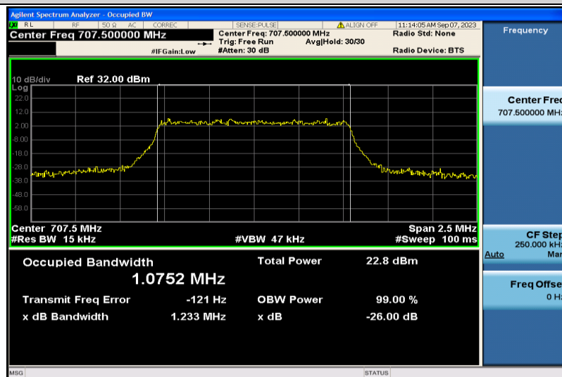
Band12-1.4MHz-16QAM-23095-6RB#0-1.0752
