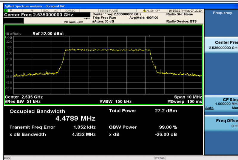
Band7-5MHz-16QAM-21100-25RB#0-4.4789
