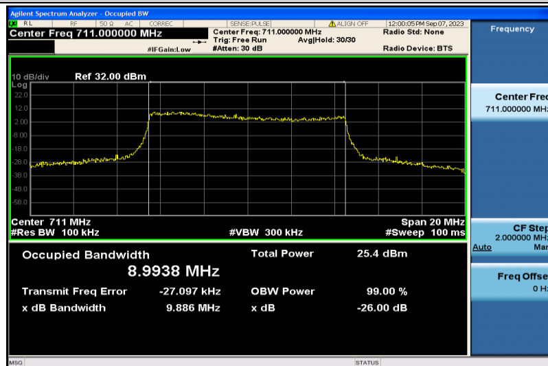
Band17-10MHz-16QAM-23800-50RB#0-8.9938
