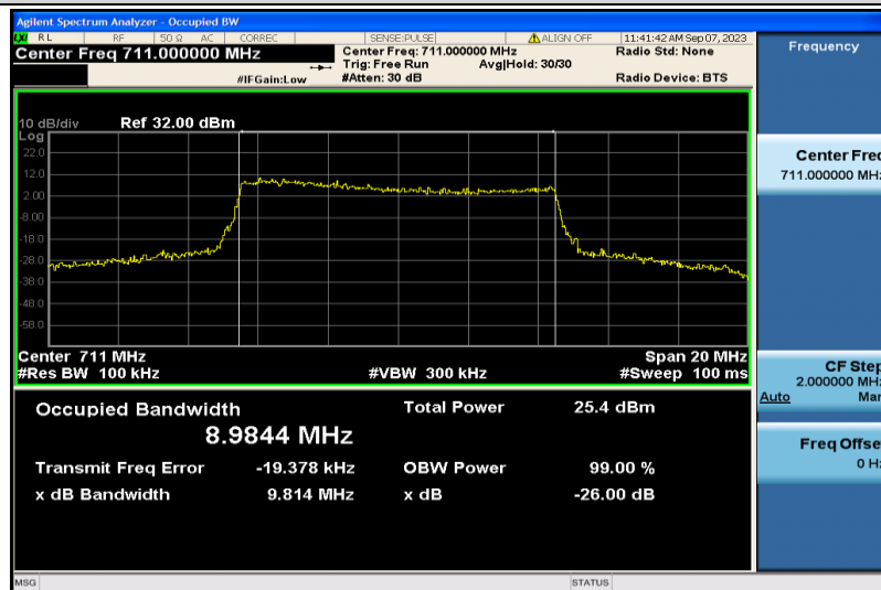
Band12-10MHz-16QAM-23130-50RB#0-8.9844
