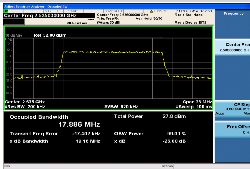
Band7-20MHz-16QAM-21100-100RB#0-17.886
