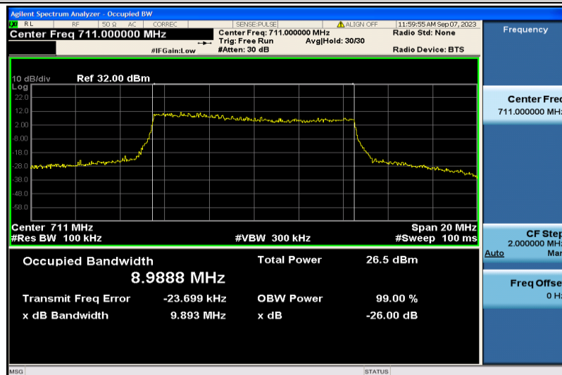
Band17-10MHz-QPSK-23800-50RB#0-8.9888
