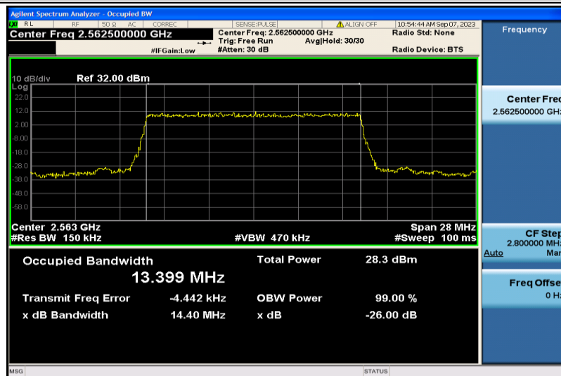
Band7-15MHz-QPSK-21375-75RB#0-13.399
