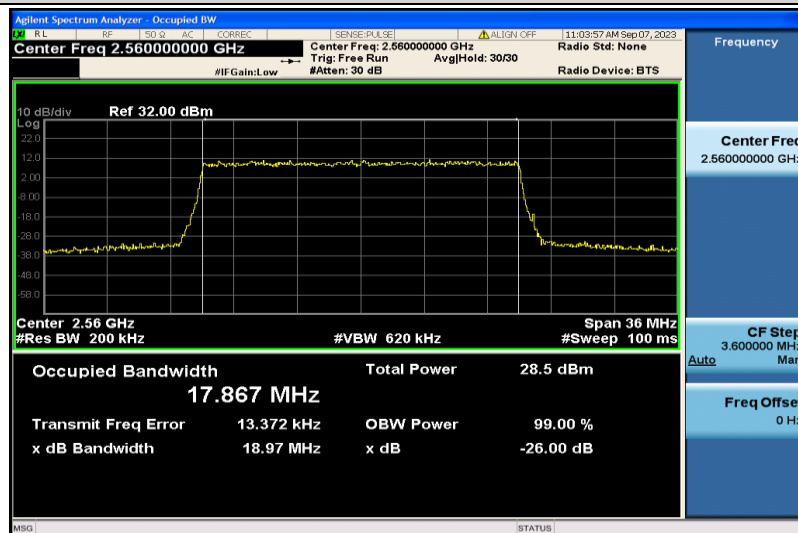
Band7-20MHz-QPSK-21350-100RB#0-17.867
