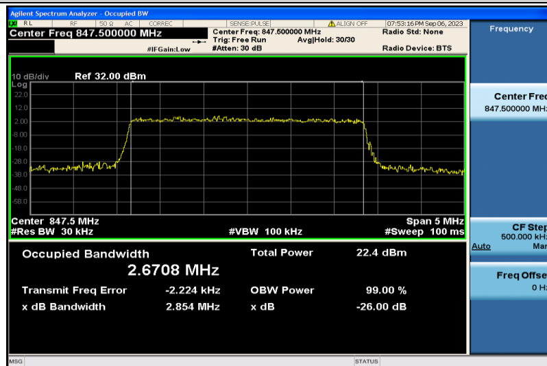
Band5-3MHz-16QAM-20635-15RB#0-2.6708
