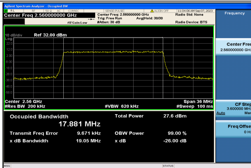
Band7-20MHz-16QAM-21350-100RB#0-17.881
