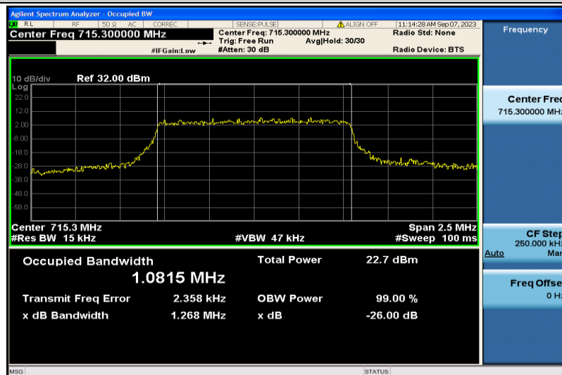
Band12-1.4MHz-16QAM-23173-6RB#0-1.0815
