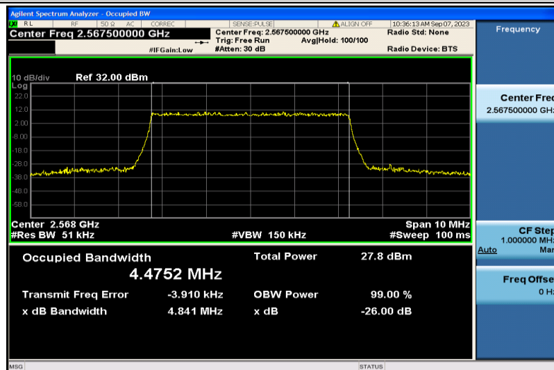
Band7-5MHz-QPSK-21425-25RB#0-4.4752
