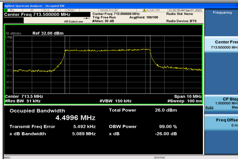
Band12-5MHz-QPSK-23155-25RB#0-4.4996
