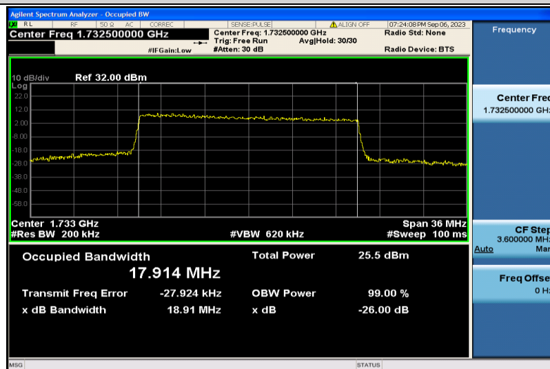
Band4-20MHz-16QAM-20175-100RB#0-17.914
