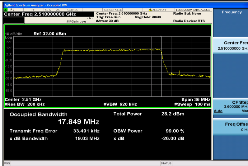
Band7-20MHz-16QAM-20850-100RB#0-17.849
