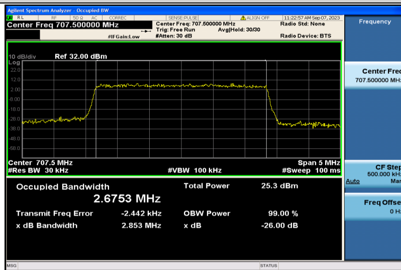
Band12-3MHz-QPSK-23095-15RB#0-2.6753
