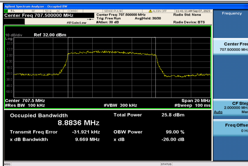
Band12-10MHz-QPSK-23095-50RB#0-8.8836
