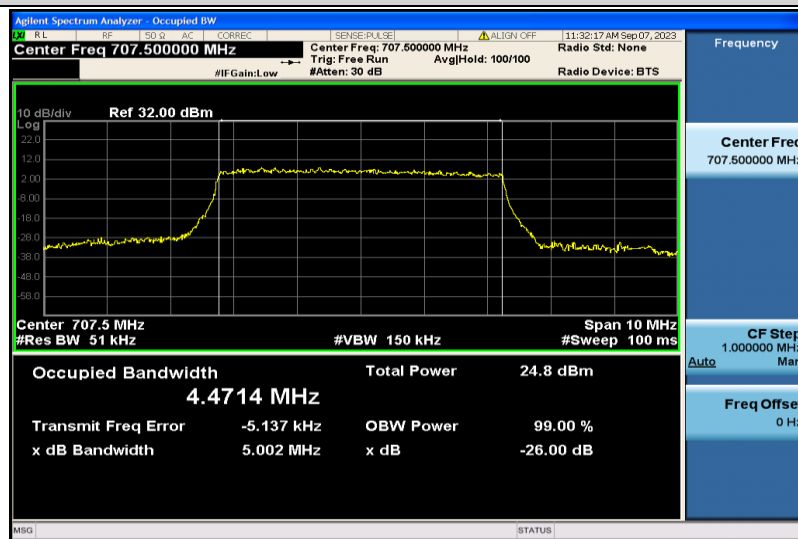
Band12-5MHz-16QAM-23095-25RB#0-4.4714
