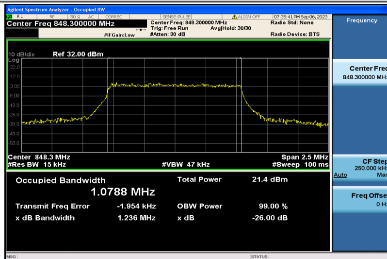
Band5-1.4MHz-16QAM-20643-6RB#0-1.0788
