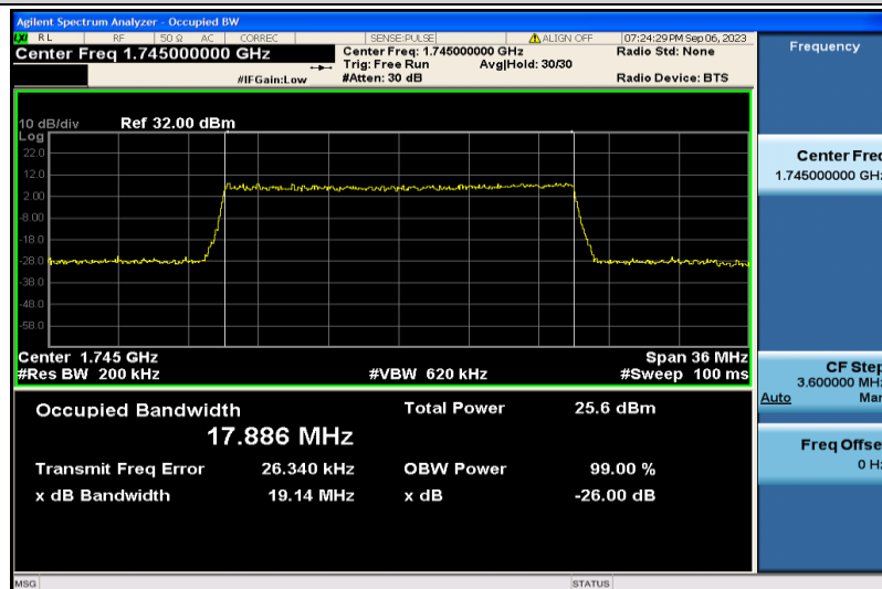
Band4-20MHz-16QAM-20300-100RB#0-17.886
