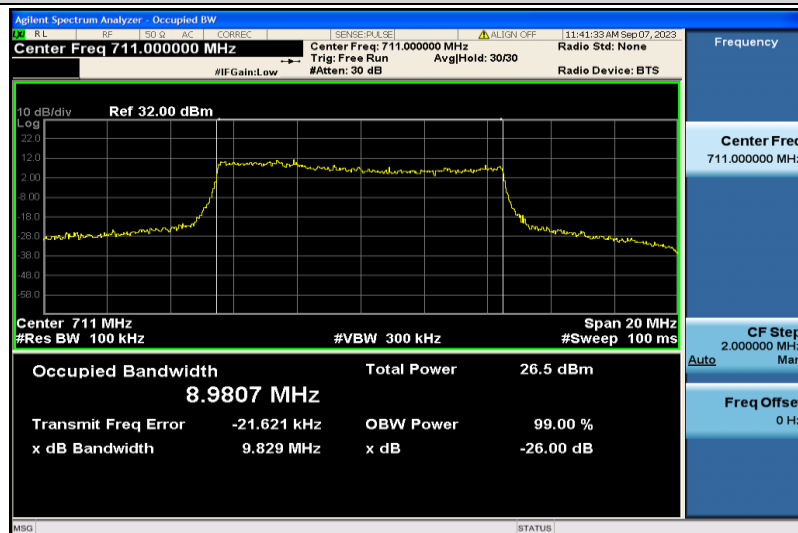
Band12-10MHz-QPSK-23130-50RB#0-8.9807
