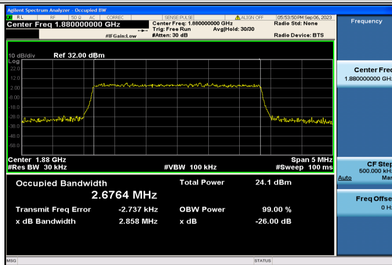
Band2-3MHz-16QAM-18900-15RB#0-2.6764
