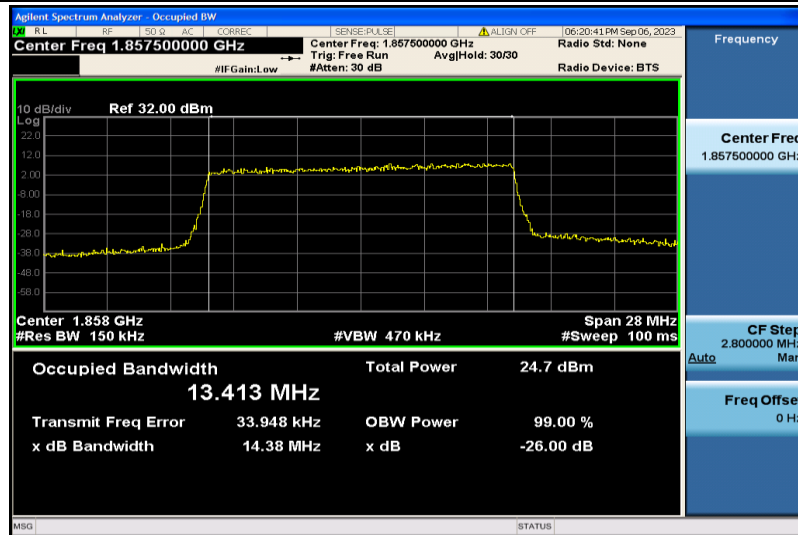
Band2-15MHz-16QAM-18675-75RB#0-13.413
