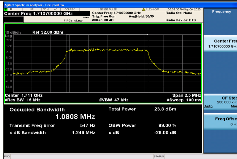
Band4-1.4MHz-16QAM-19957-6RB#0-1.0808
