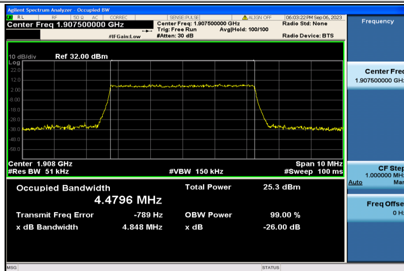
Band2-5MHz-QPSK-19175-25RB#0-4.4796
