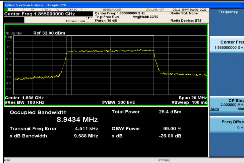
Band2-10MHz-QPSK-18650-50RB#0-8.9434
