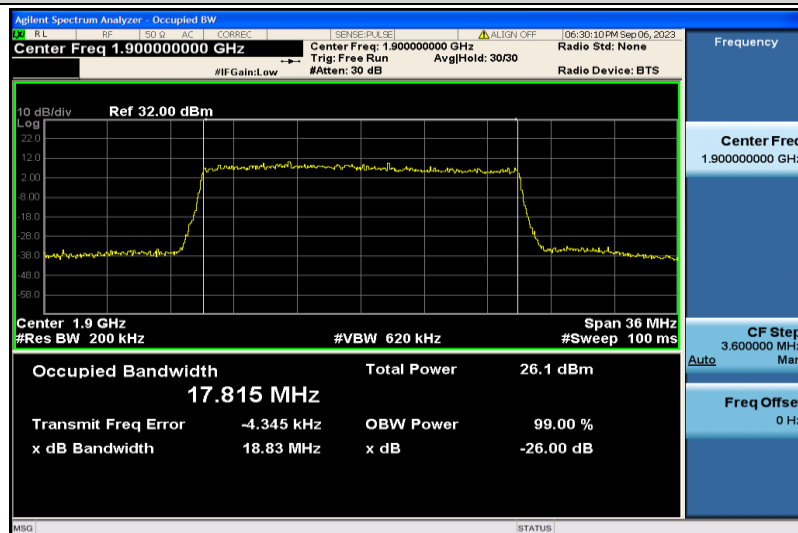
Band2-20MHz-QPSK-19100-100RB#0-17.815
