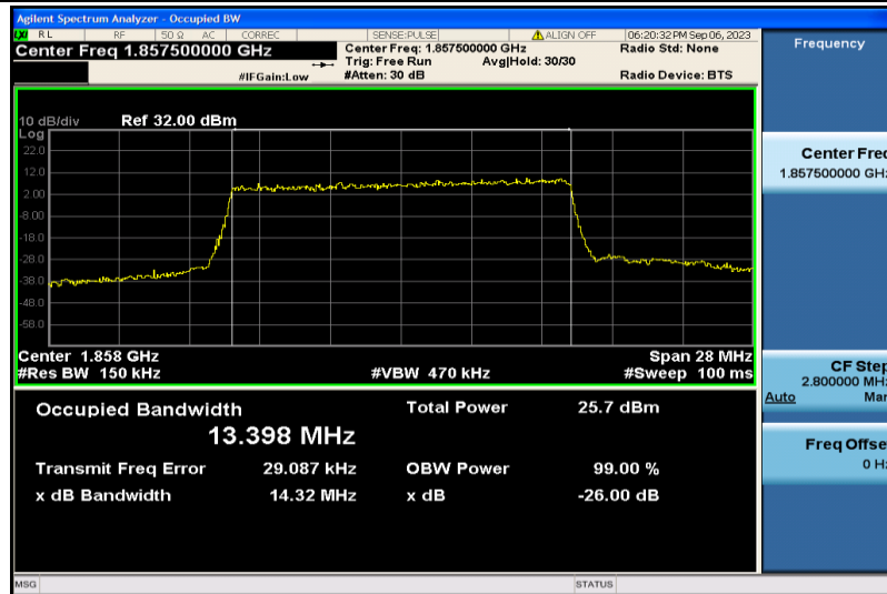
Band2-15MHz-QPSK-18675-75RB#0-13.398
