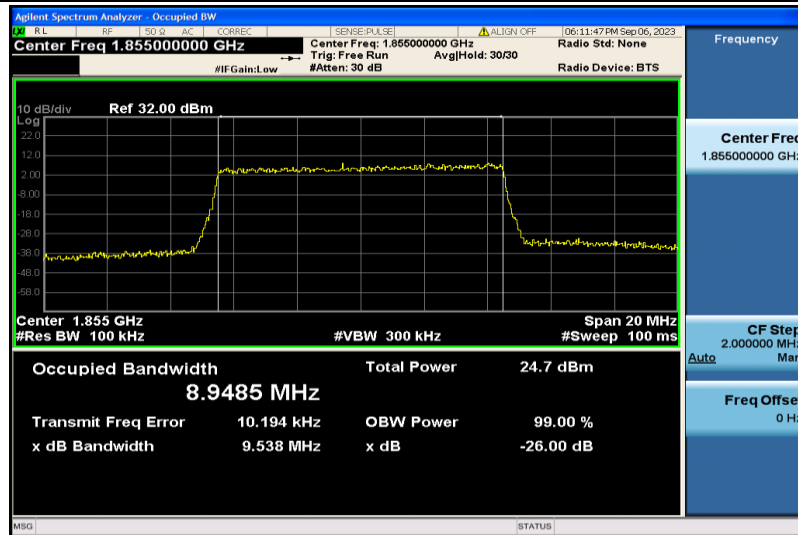
Band2-10MHz-16QAM-18650-50RB#0-8.9485
