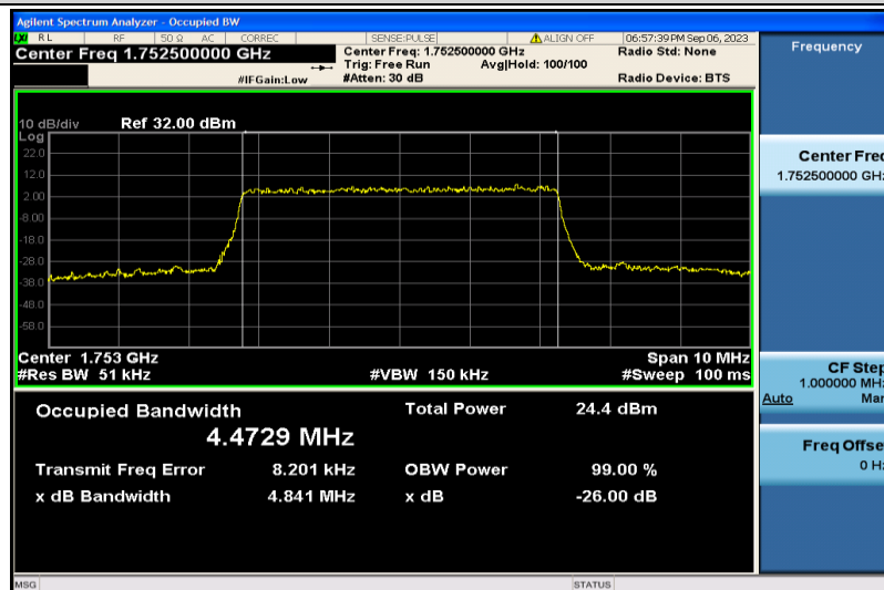
Band4-5MHz-16QAM-20375-25RB#0-4.4729
