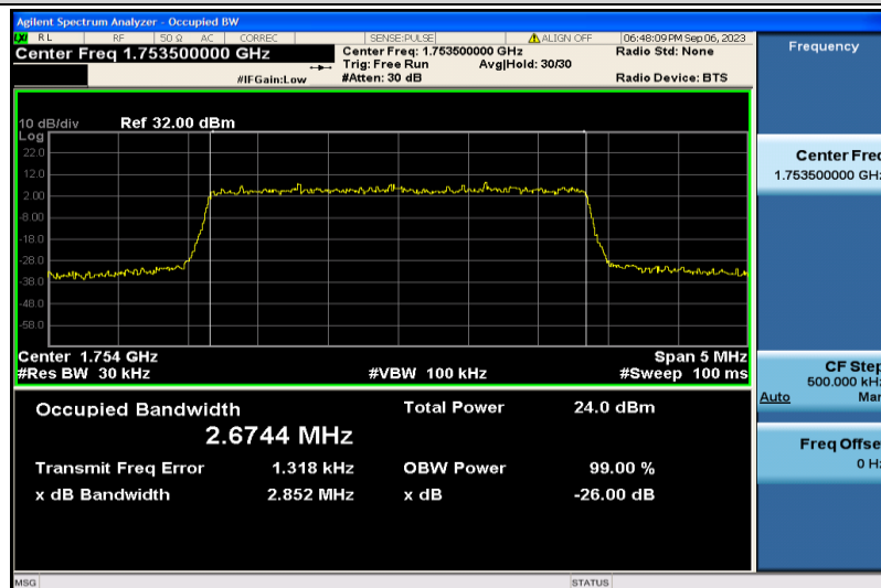
Band4-3MHz-16QAM-20385-15RB#0-2.6744
