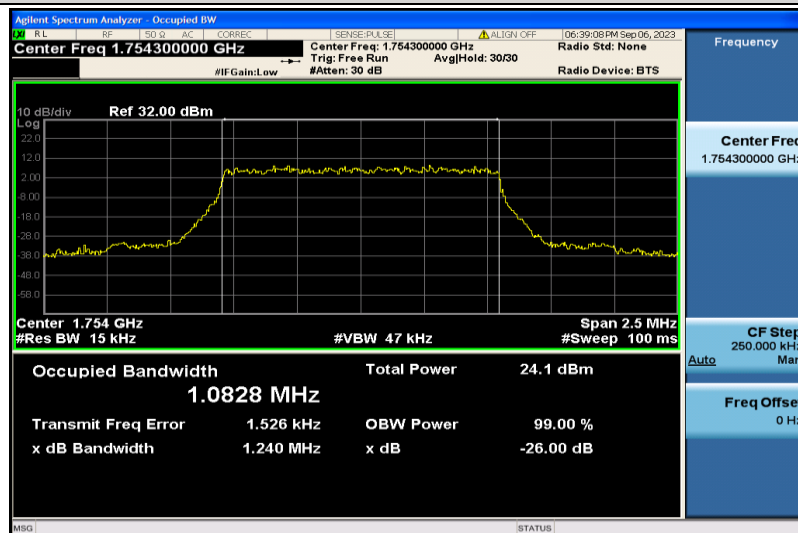
Band4-1.4MHz-QPSK-20393-6RB#0-1.0828
