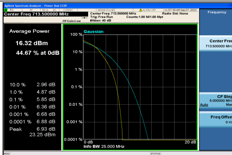
Band17-5MHz-16QAM-23825-25RB#0
