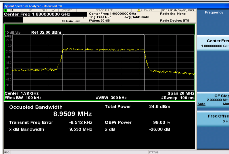
Band2-10MHz-16QAM-18900-50RB#0-8.9509
