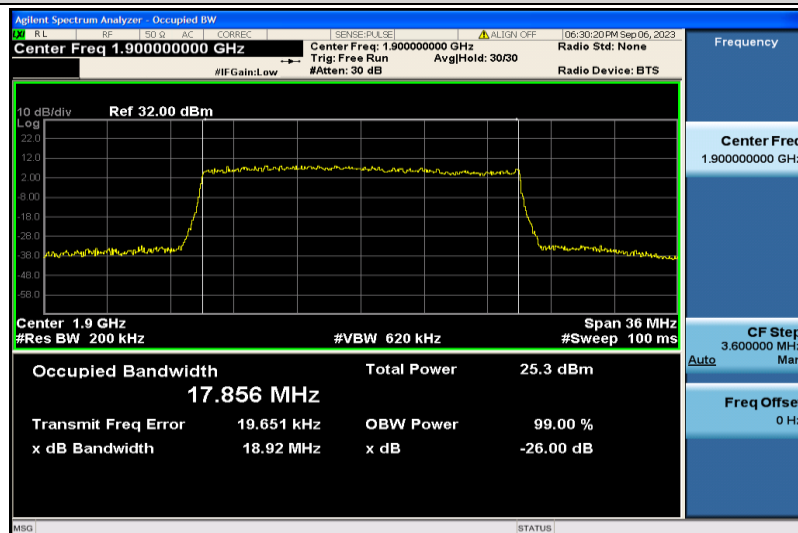
Band2-20MHz-16QAM-19100-100RB#0-17.856
