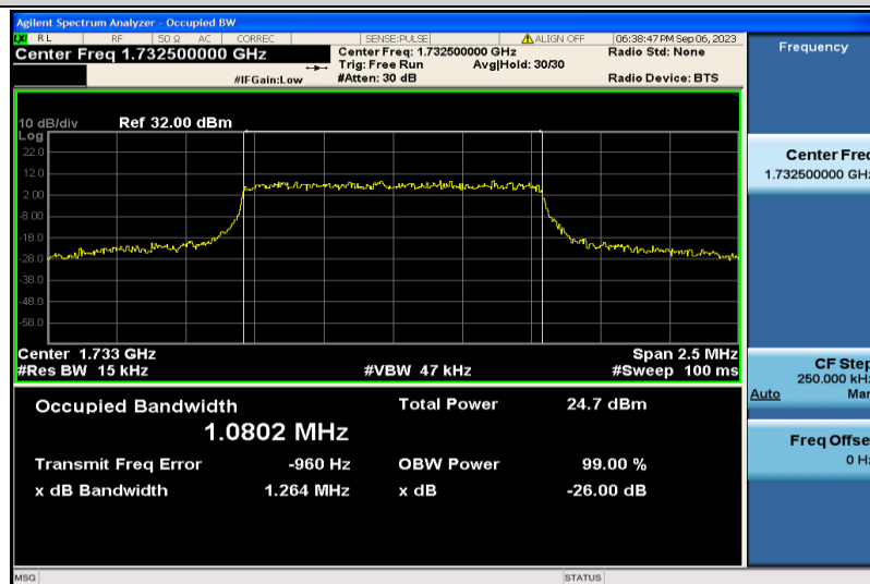
Band4-1.4MHz-QPSK-20175-6RB#0-1.0802
