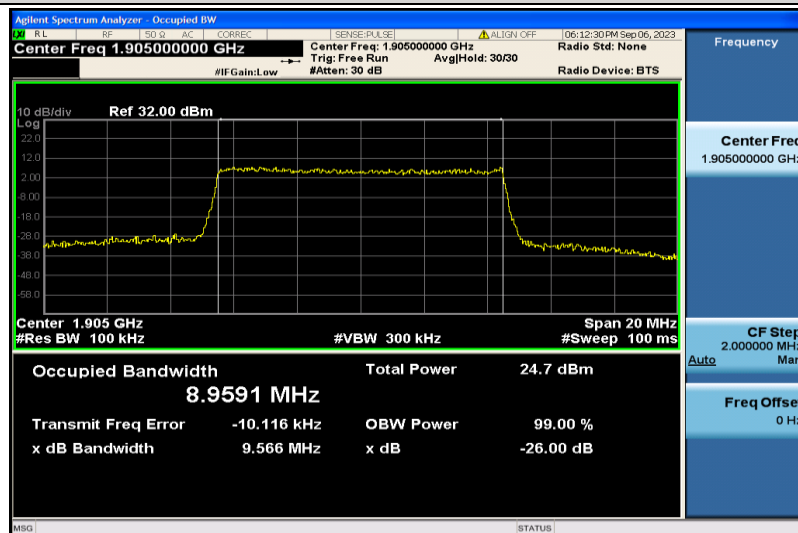
Band2-10MHz-16QAM-19150-50RB#0-8.9591
