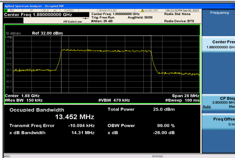
Band2-15MHz-16QAM-18900-75RB#0-13.452
