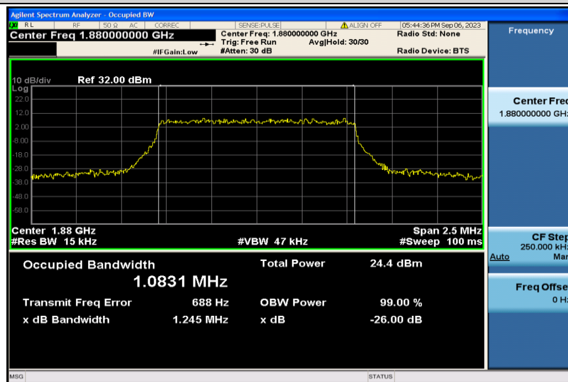
Band2-1.4MHz-QPSK-18900-6RB#0-1.0831
