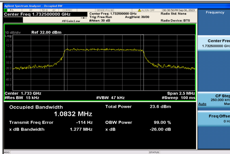
Band4-1.4MHz-16QAM-20175-6RB#0-1.0832
