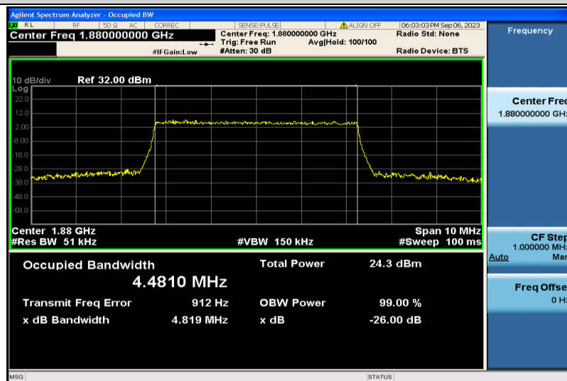
Band2-5MHz-16QAM-18900-25RB#0-4.4810
