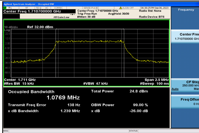
Band4-1.4MHz-QPSK-19957-6RB#0-1.0769
