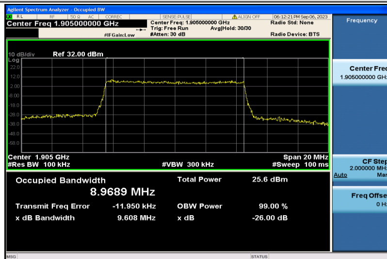
Band2-10MHz-QPSK-19150-50RB#0-8.9689
