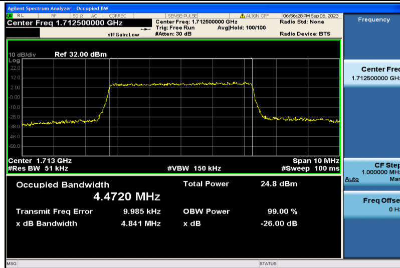
Band4-5MHz-16QAM-19975-25RB#0-4.4720
