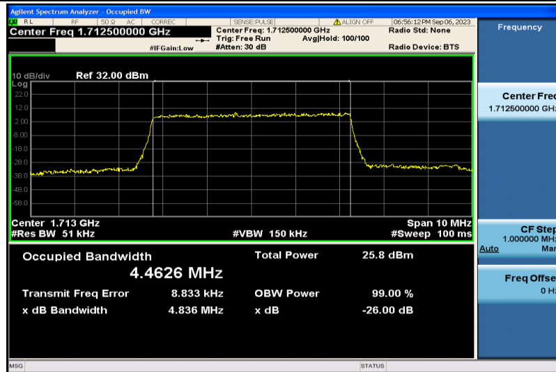
Band4-5MHz-QPSK-19975-25RB#0-4.4626
