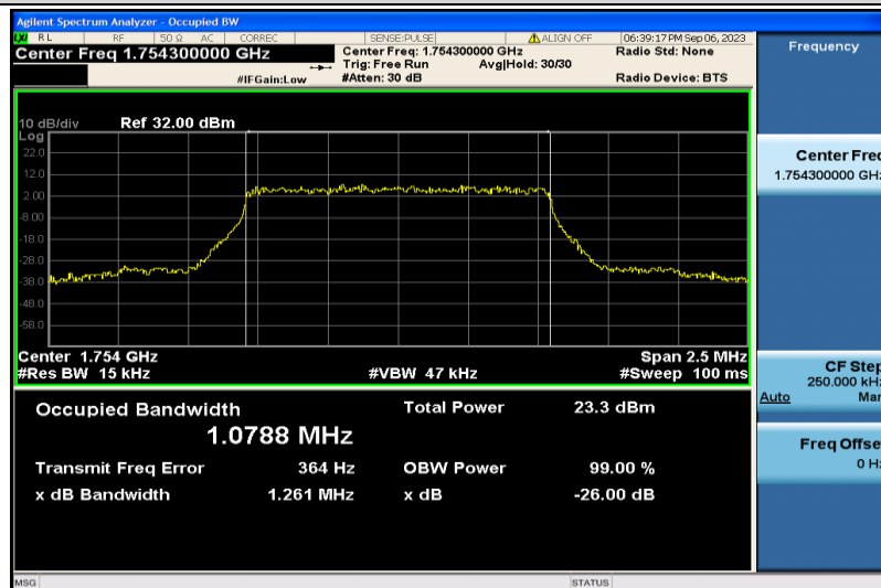
Band4-1.4MHz-16QAM-20393-6RB#0-1.0788
