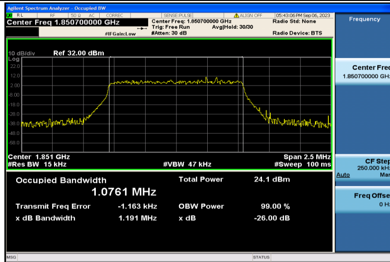
Band2-1.4MHz-QPSK-18607-6RB#0-1.0761
