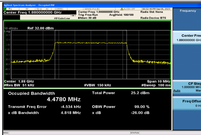
Band2-5MHz-QPSK-18900-25RB#0-4.4780
