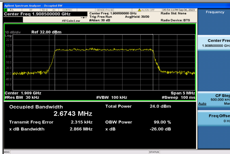
Band2-3MHz-16QAM-19185-15RB#0-2.6743
