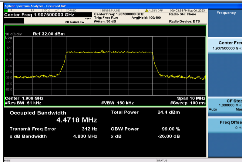
Band2-5MHz-16QAM-19175-25RB#0-4.4718
