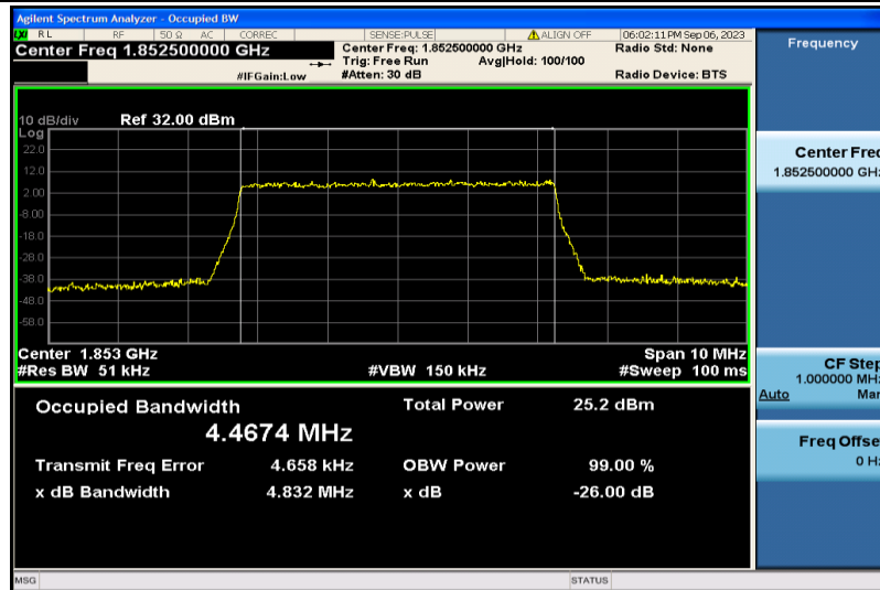
Band2-5MHz-QPSK-18625-25RB#0-4.4674
