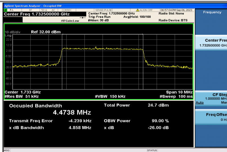
Band4-5MHz-16QAM-20175-25RB#0-4.4738
