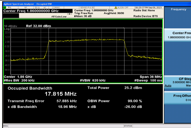
Band2-20MHz-16QAM-18700-100RB#0-17.815
