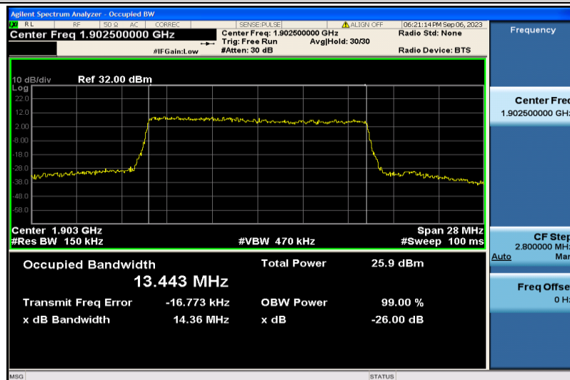
Band2-15MHz-QPSK-19125-75RB#0-13.443
