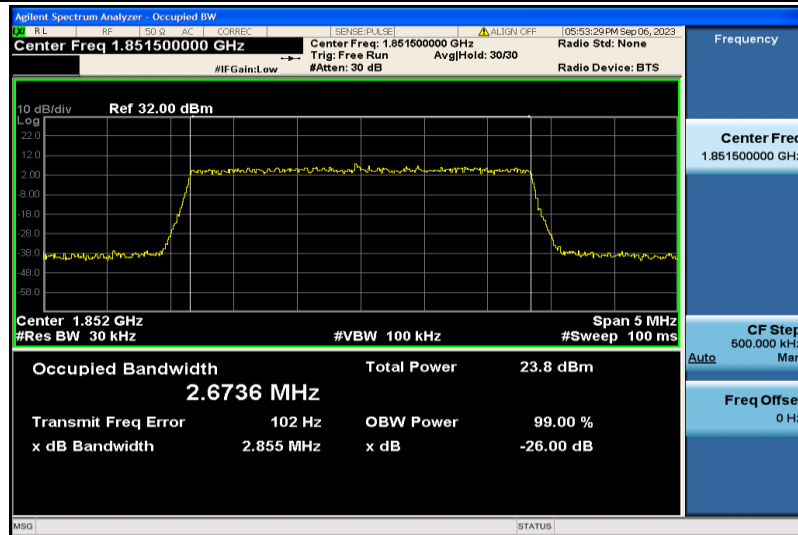
Band2-3MHz-16QAM-18615-15RB#0-2.6736
