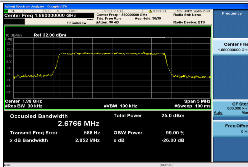
Band2-3MHz-QPSK-18900-15RB#0-2.6766
