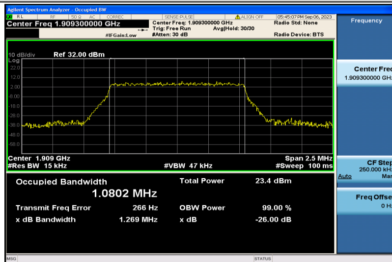
Band2-1.4MHz-16QAM-19193-6RB#0-1.0802
