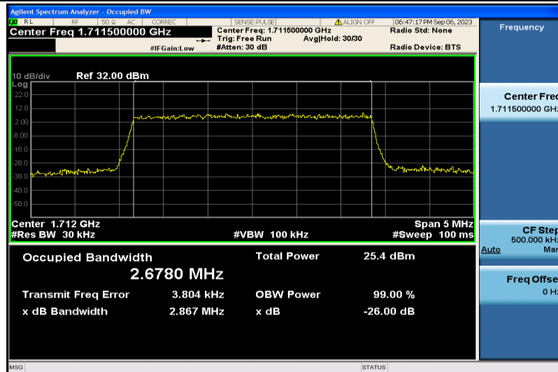
Band4-3MHz-QPSK-19965-15RB#0-2.6780
