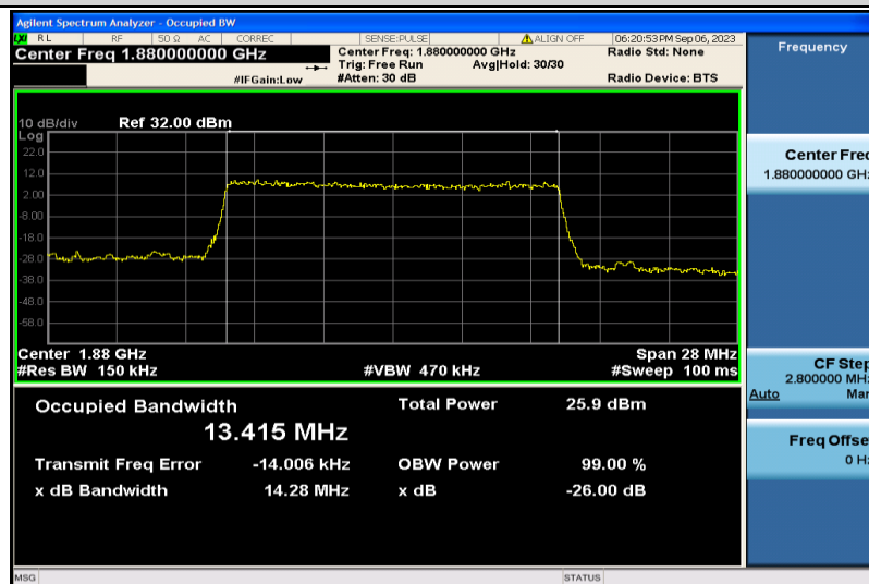
Band2-15MHz-QPSK-18900-75RB#0-13.415
