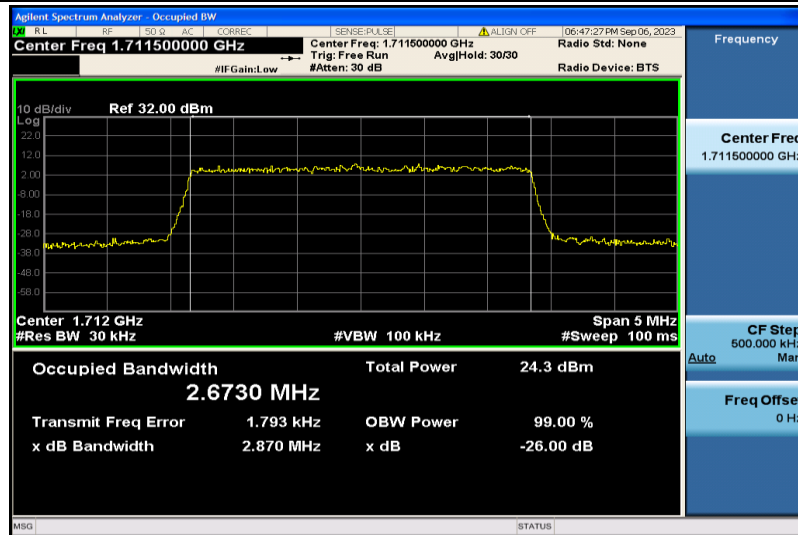
Band4-3MHz-16QAM-19965-15RB#0-2.6730
