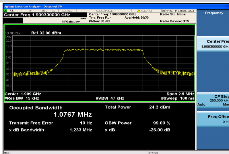
Band2-1.4MHz-QPSK-19193-6RB#0-1.0767
