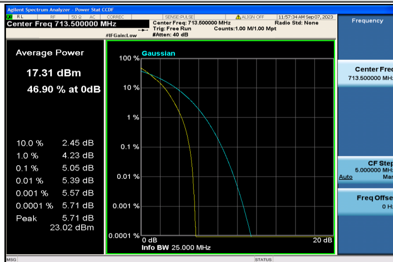
Band17-5MHz-QPSK-23825-25RB#0
