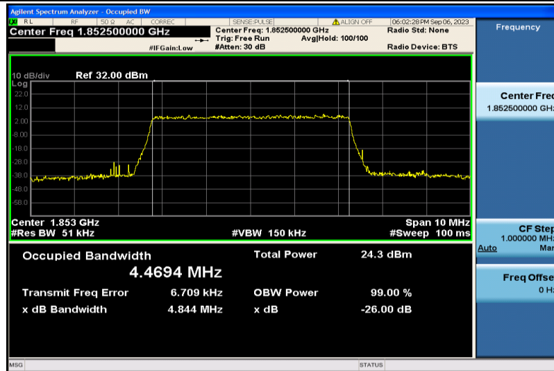
Band2-5MHz-16QAM-18625-25RB#0-4.4694
