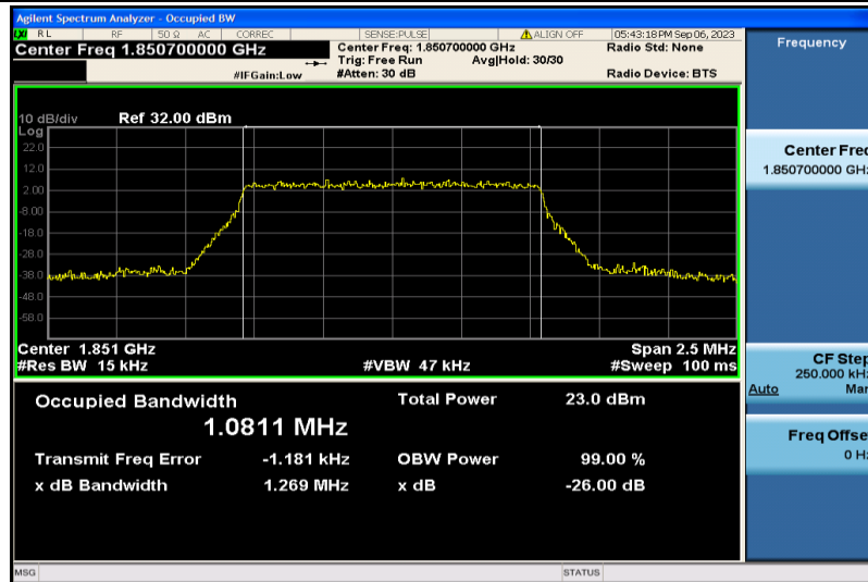
Band2-1.4MHz-16QAM-18607-6RB#0-1.0811
