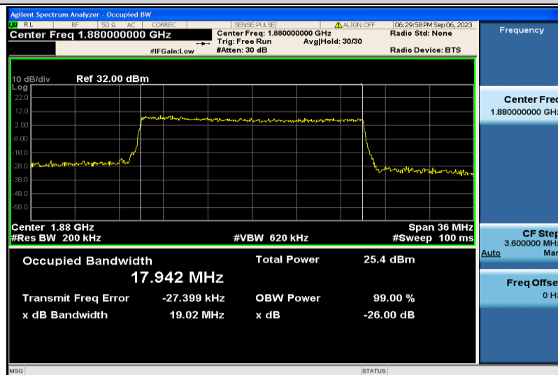
Band2-20MHz-16QAM-18900-100RB#0-17.942
