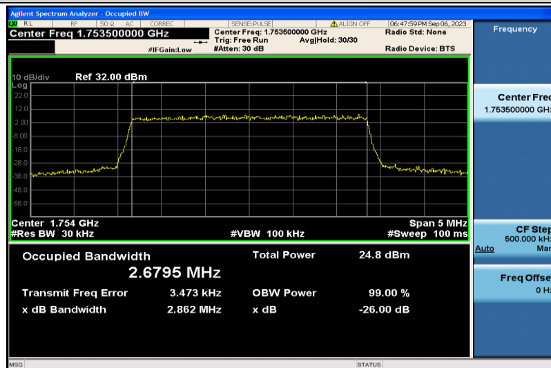
Band4-3MHz-QPSK-20385-15RB#0-2.6795
