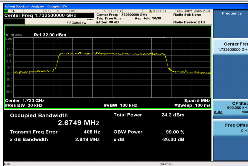
Band4-3MHz-16QAM-20175-15RB#0-2.6749
