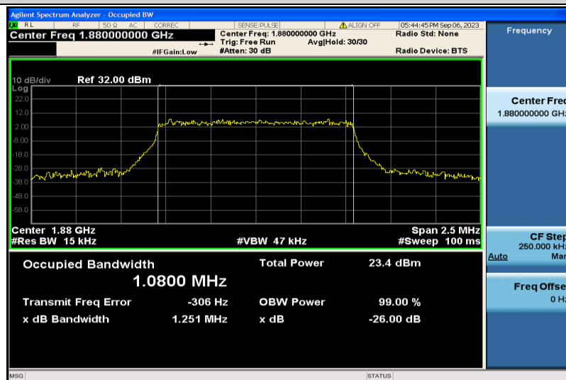
Band2-1.4MHz-16QAM-18900-6RB#0-1.0800
