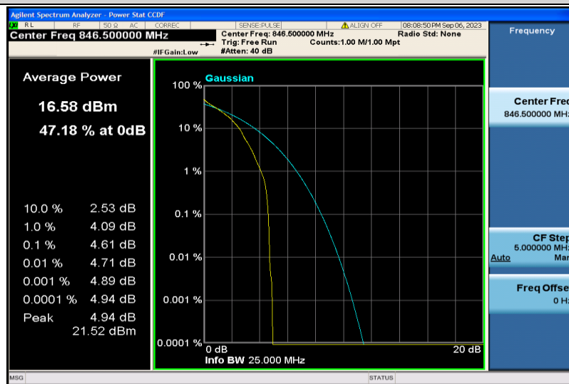
Band5-5MHz-QPSK-20625-1RB#0
