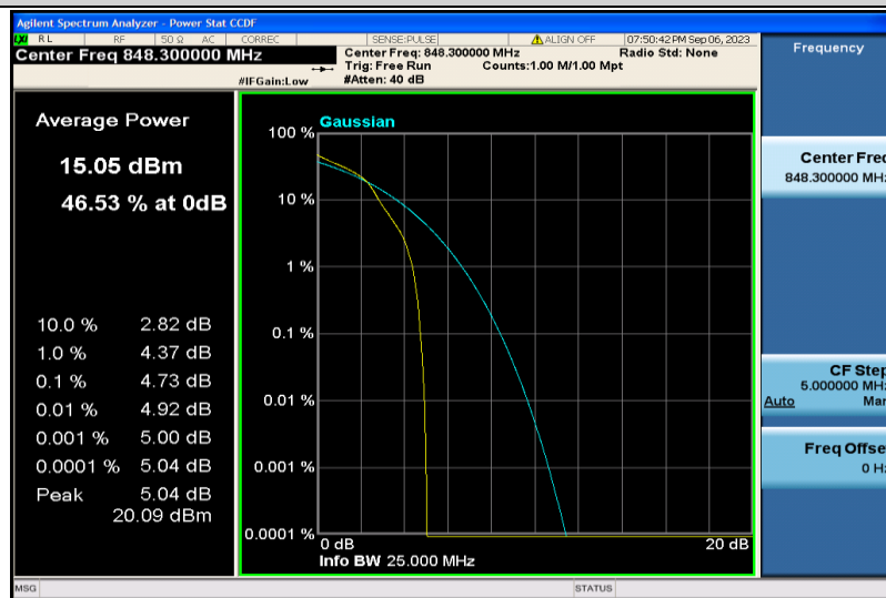
Band5-1.4MHz-16QAM-20643-1RB#0
