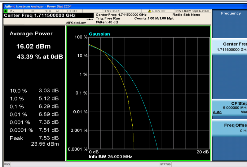
Band4-3MHz-16QAM-19965-15RB#0
