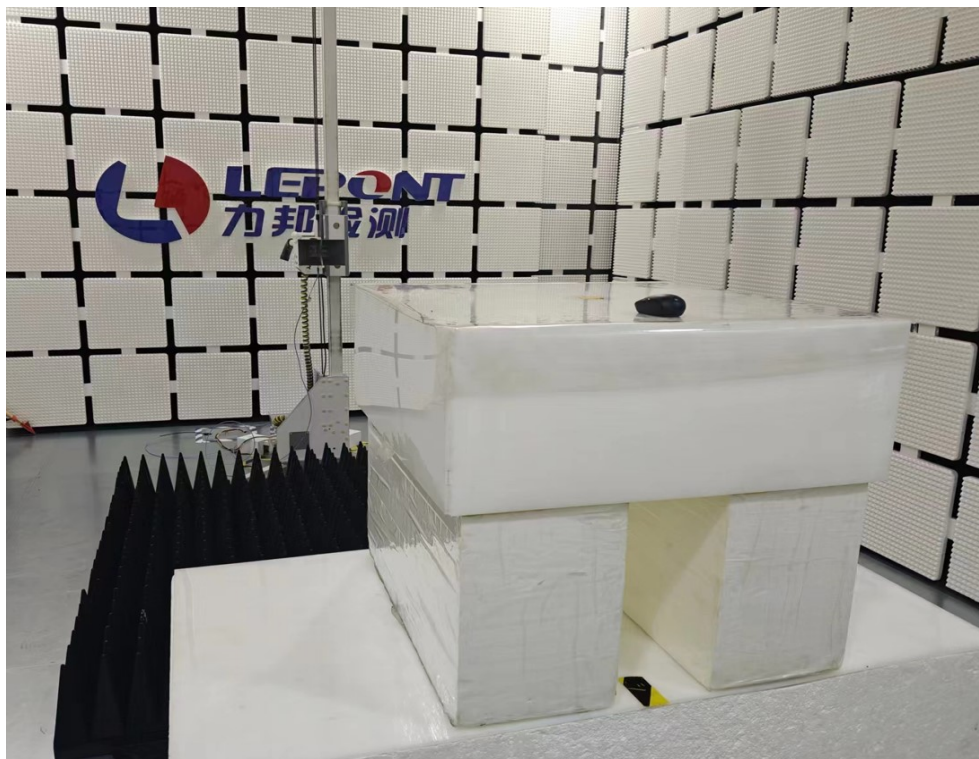
Photograph 2: Set-up for Radiated Spurious Emission, Above 1GHz
