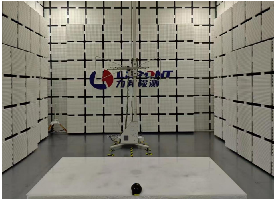
Photograph 1: Set-up for Radiated Spurious Emission, 30MHz - 1GHz
