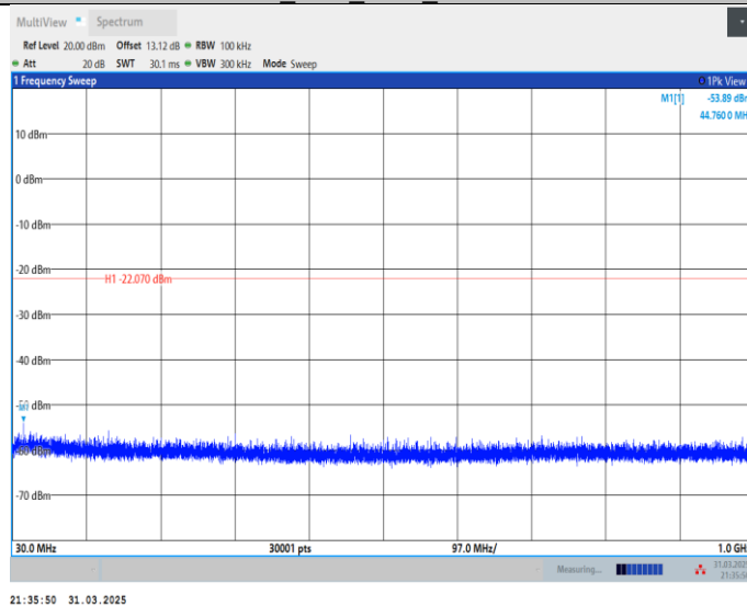
SRD_Ant1_2403_30~1000
