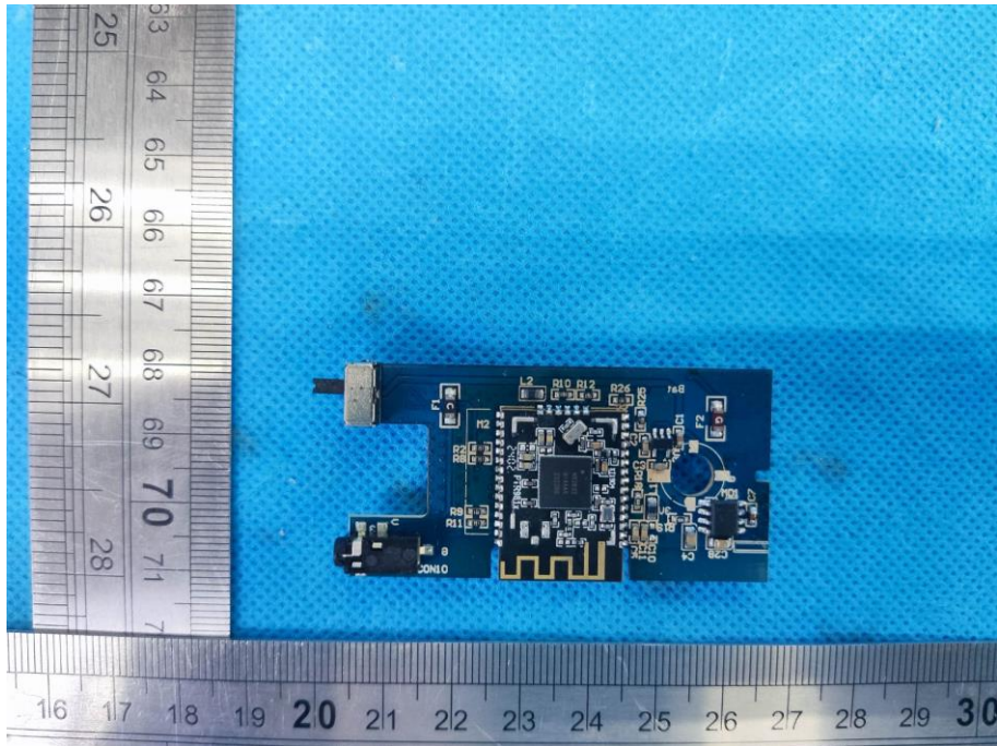
Inner View of the EUT
