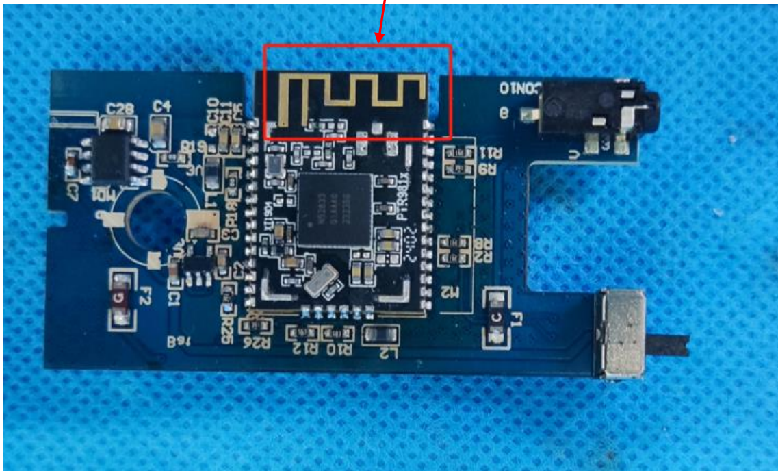
wireless antenna
