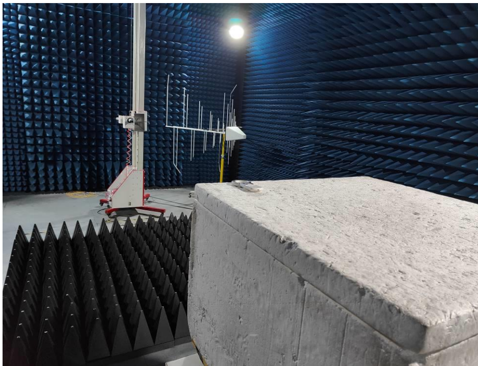
Above 1GHz
