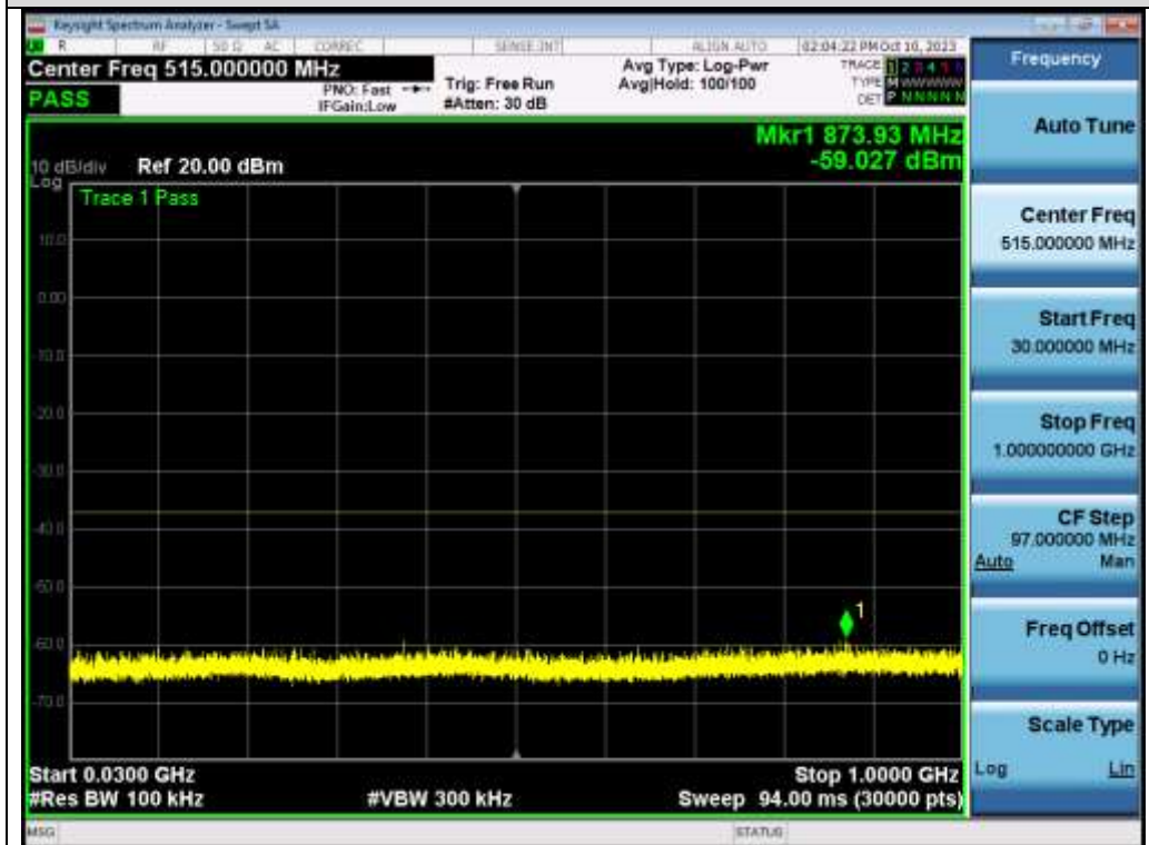
Test_Graph_802.11a_ANT2_5240_6Mbps_Frequency Band 1
