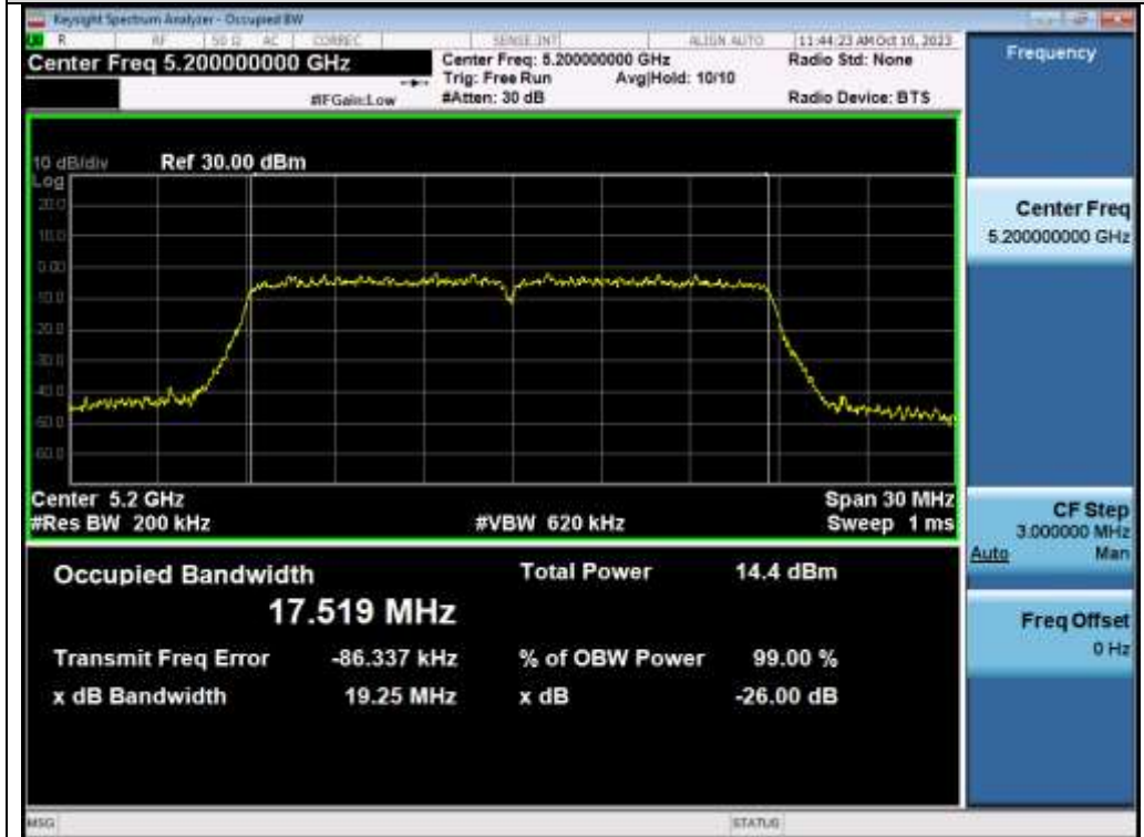
Test_Graph_802.11ac20_ANT1_5200_MCS0_OBW
