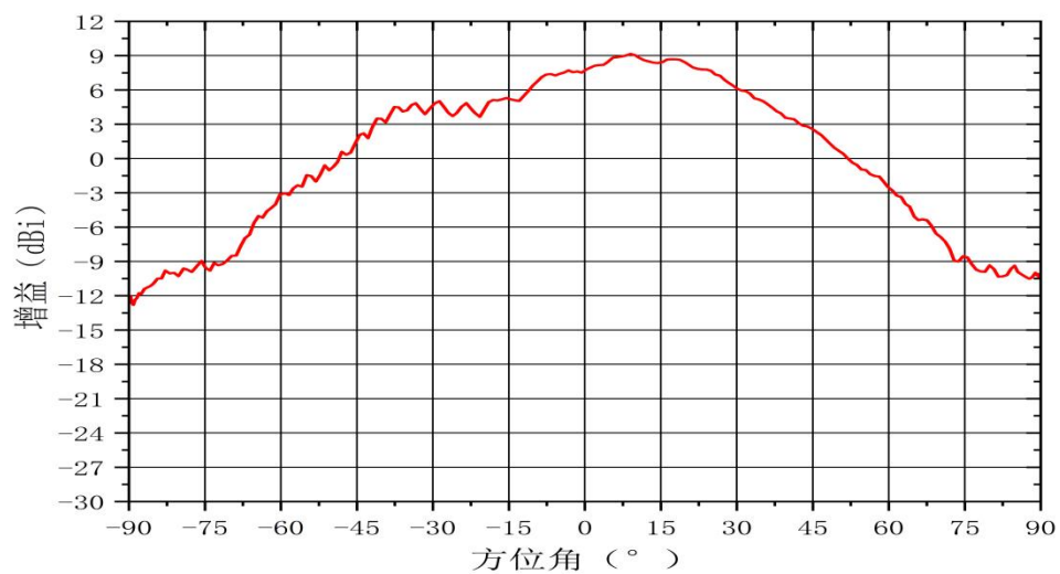
方位面方向图(TX1)Freq:62.0GHz
