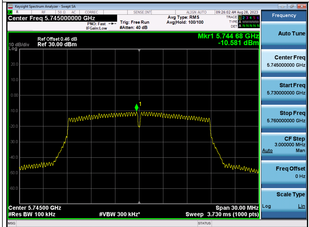
Test_Graph_802.11ac20_ANT2_5745_MCS0_PSD
