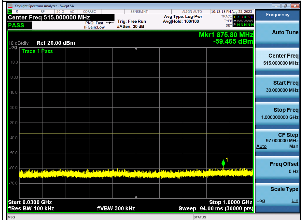
Test_Graph_802.11a_ANT2_5320_6Mbps_Frequency Band 1
