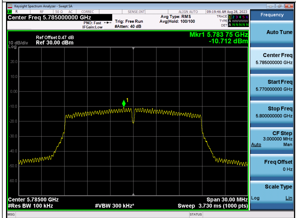
Test_Graph_802.11n20_ANT2_5785_MCS0_PSD
