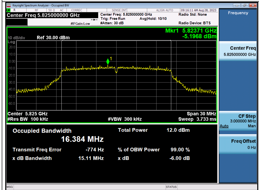
Test_Graph_802.11a_ANT2_5825_6Mbps_DTSSBW
