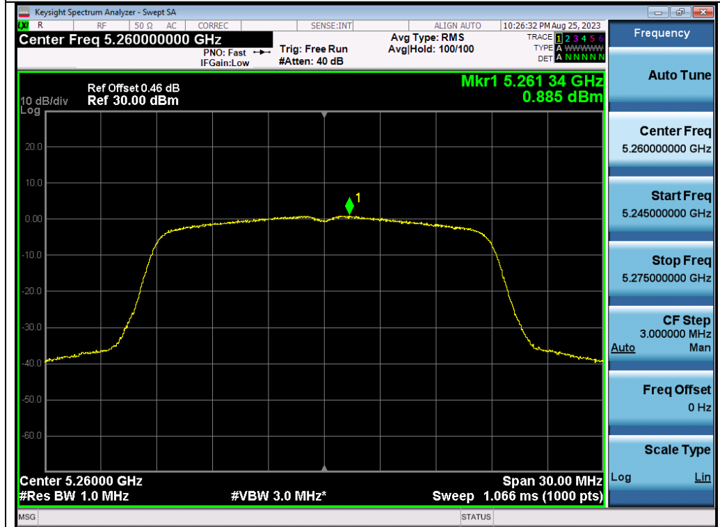
Test_Graph_802.11ac20_ANT2_5260_MCS0_PSD
