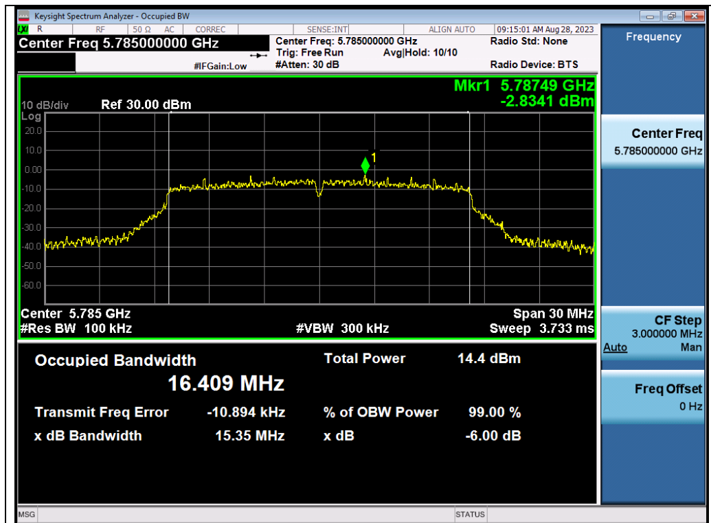
Test_Graph_802.11a_ANT2_5785_6Mbps_DTSSBW
