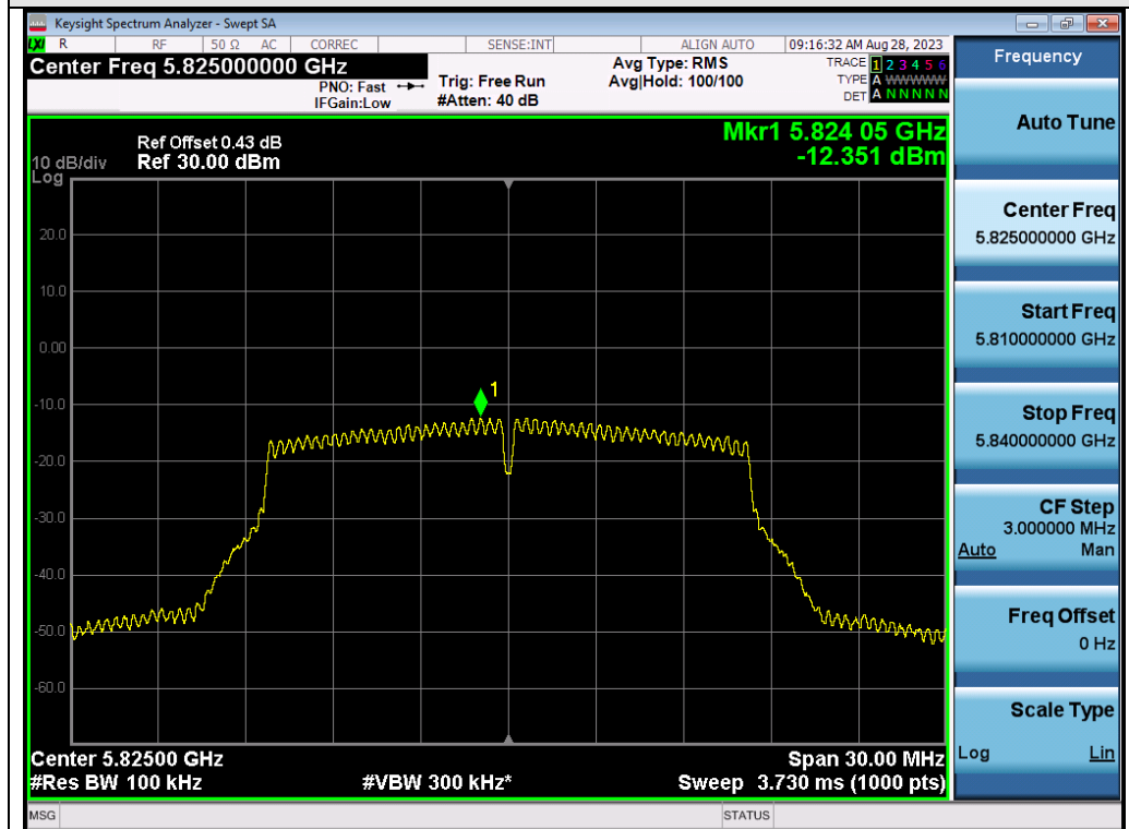
Test_Graph_802.11a_ANT2_5825_6Mbps_PSD
