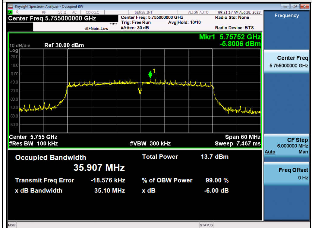
Test_Graph_802.11n40_ANT2_5755_MCS0_DTSBW
