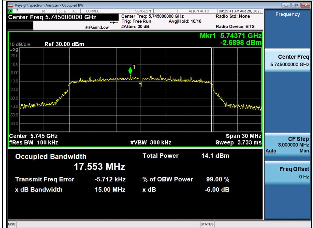
Test_Graph_802.11ac20_ANT2_5745_MCS0_DTSBW
