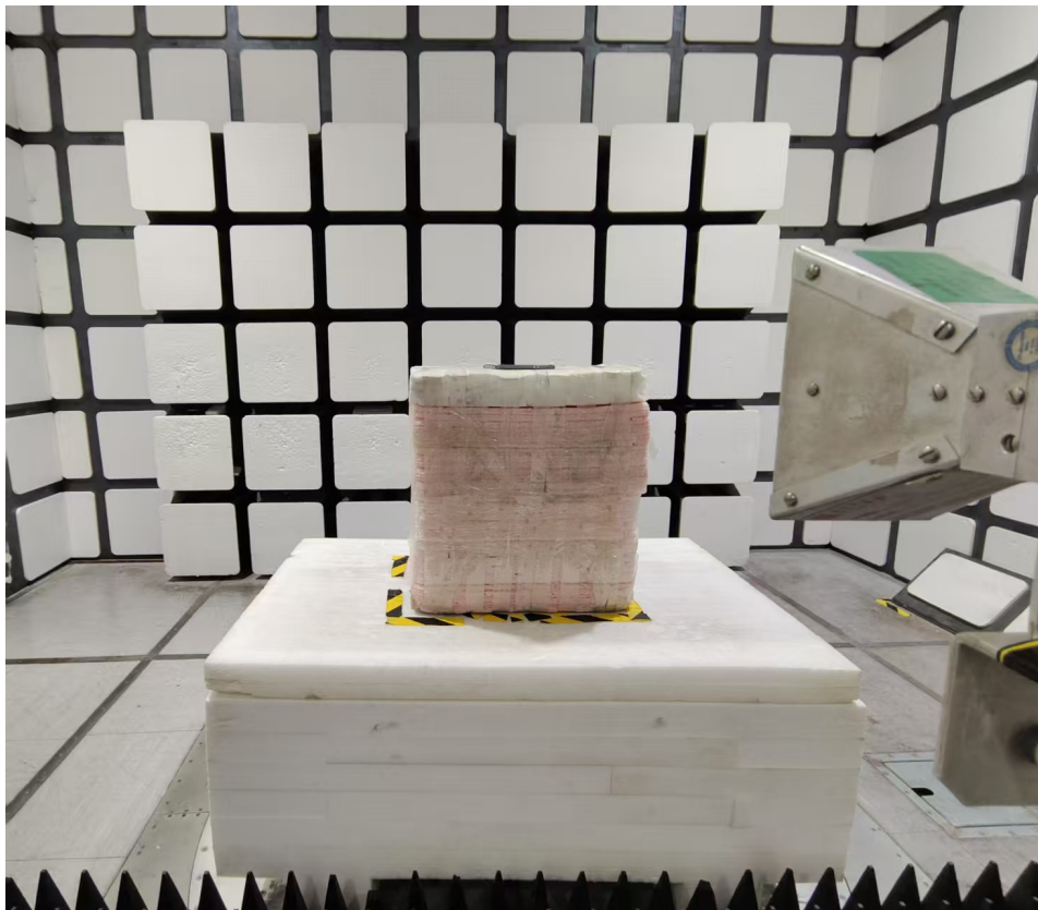
Radiated Emissions View (18-40 GHz)
