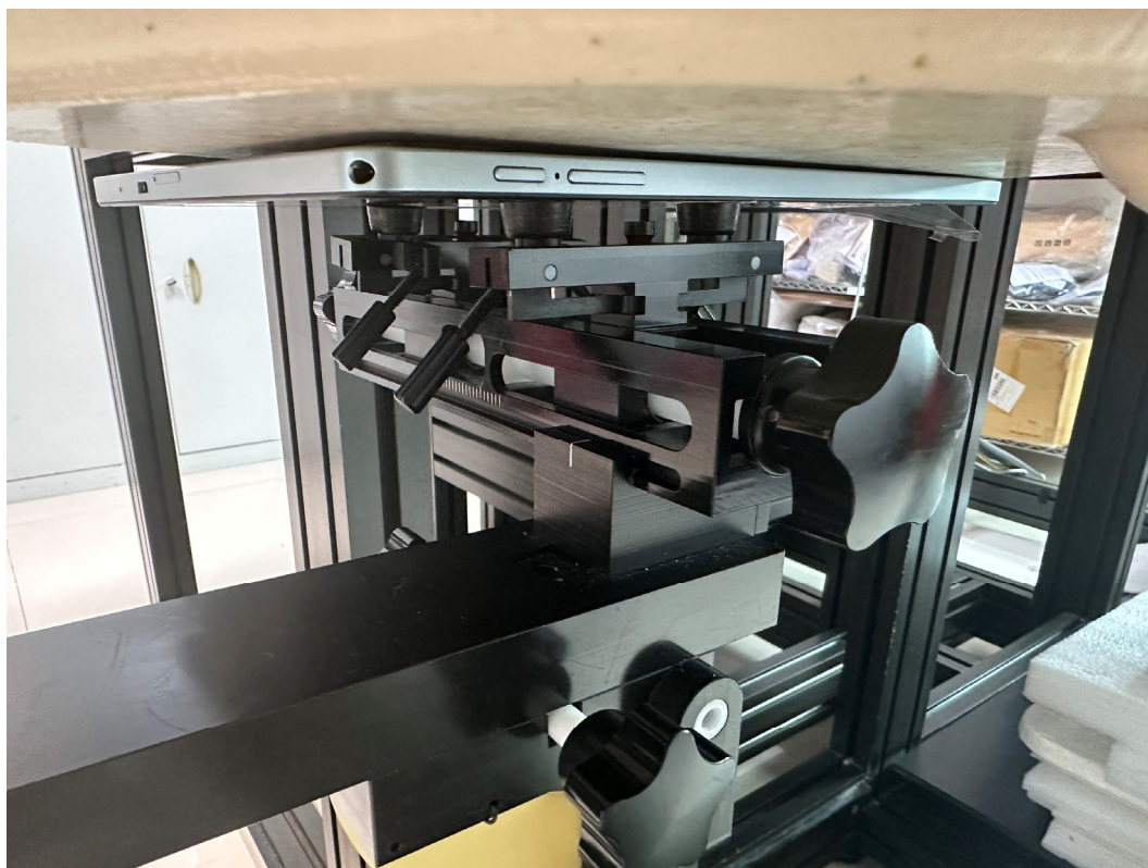
Body Back- WIFI/BT Antenna Setup Photo (0 mm)
