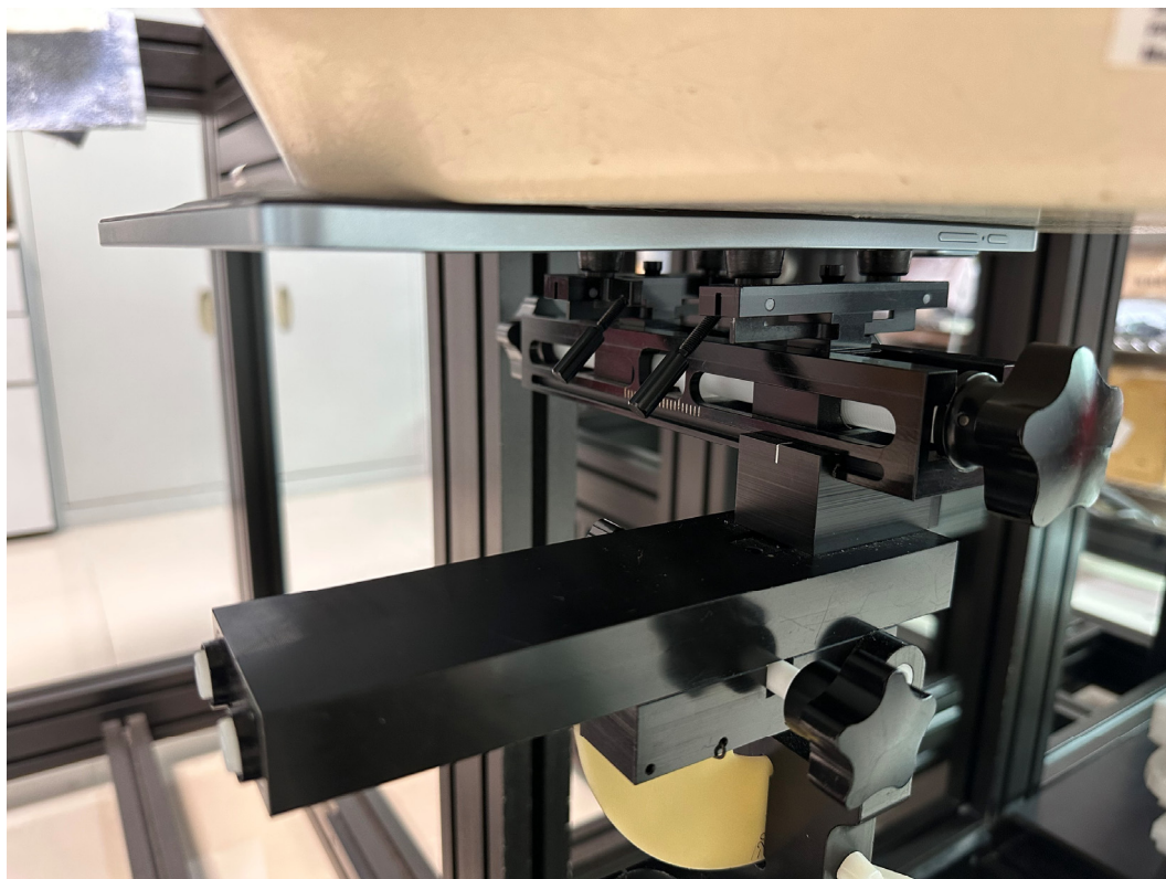
Body Front- WIFI/BT Antenna Setup Photo (0 mm)
