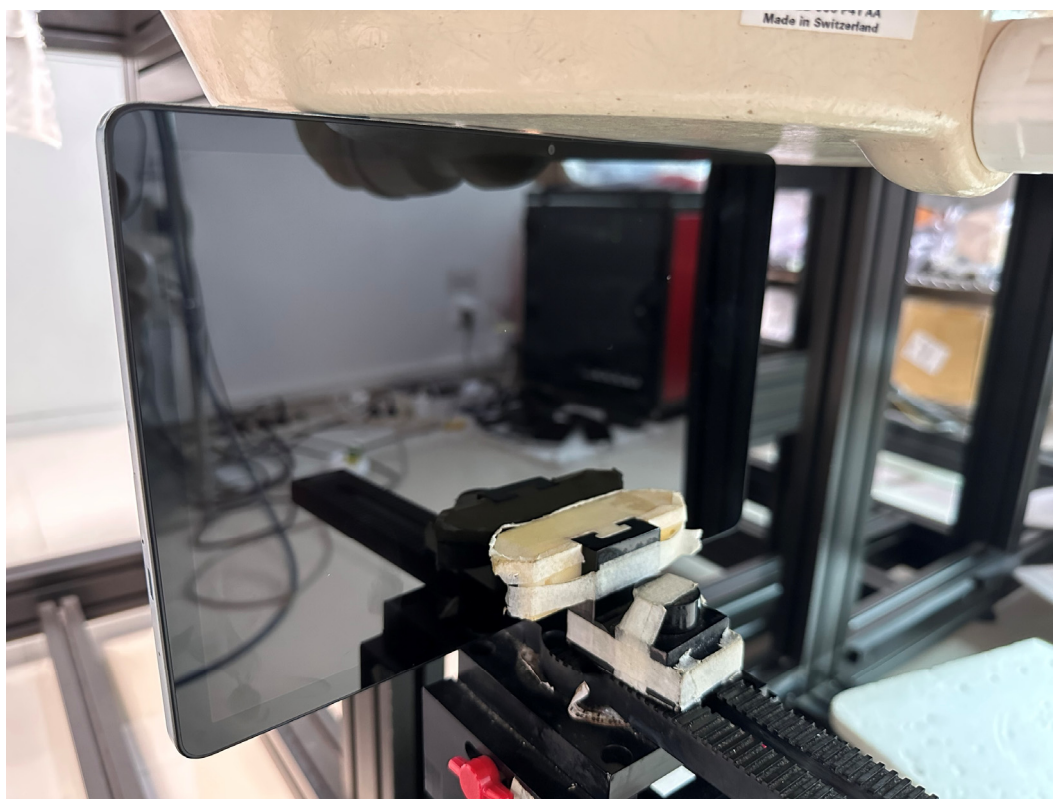
Body Top-WIFI/BT Antenna Setup Photo (0 mm)
