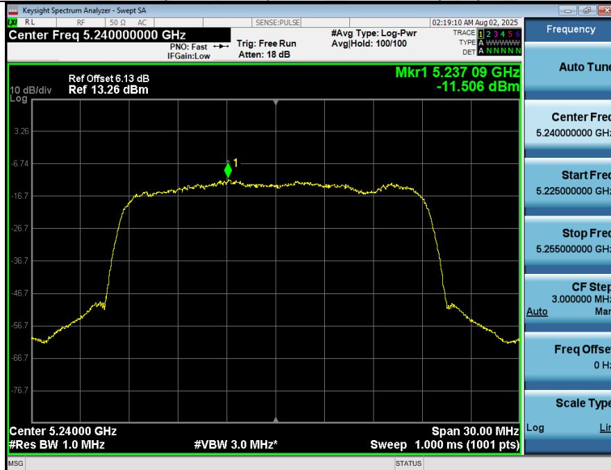
Power Spectral Density NVNT_ANT1_802_11n(HT20)_5240
