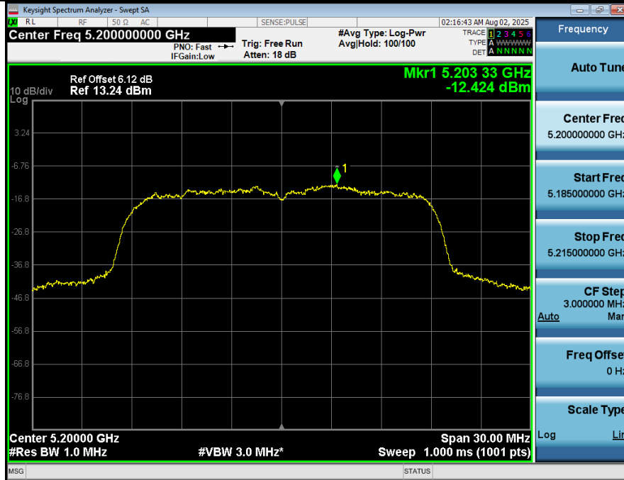
Power Spectral Density NVNT_ANT1_802_11n(HT20)_5200
