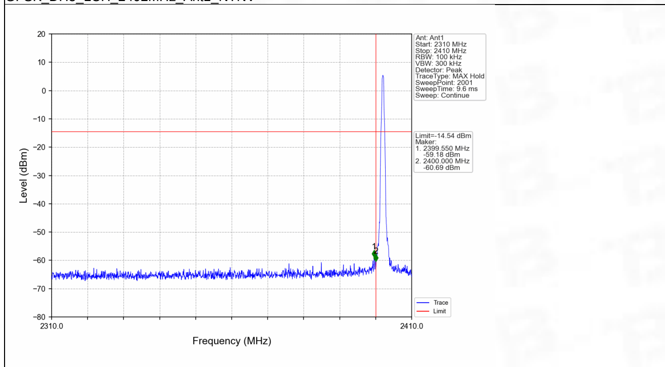
GFSK_DH5_LCH_2402MHz_Ant1_NTNV
