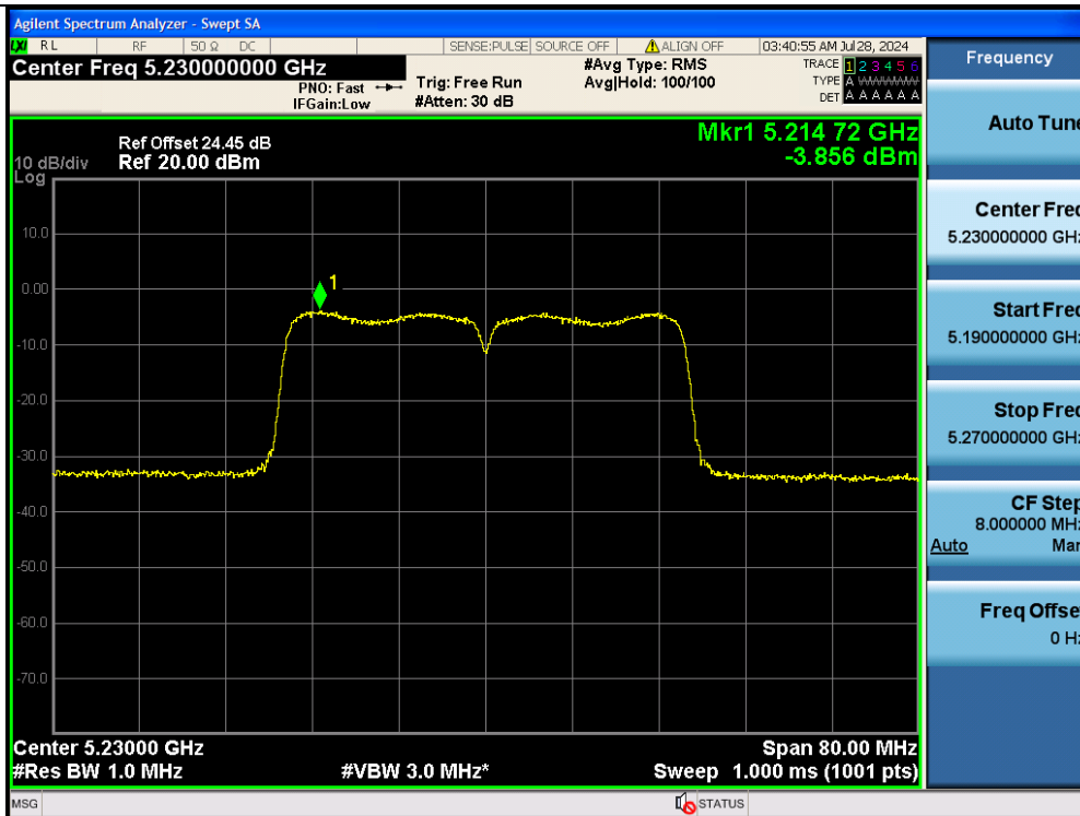
11AC40MIMO-Ant2-5230-PASS
