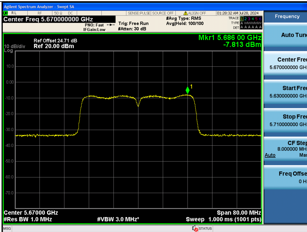
11N40MIMO-Ant2-5670-PASS
