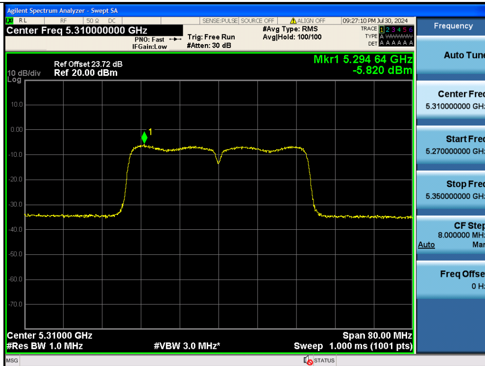
11AC40MIMO-Ant2-5310-PASS
