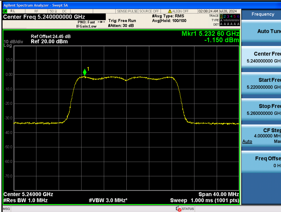
11AC20MIMO-Ant2-5240-PASS
