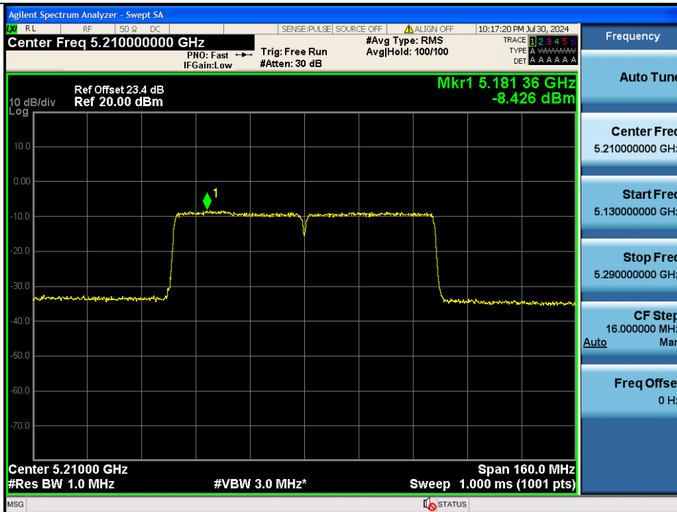
11AC80MIMO-Ant2-5210-PASS
