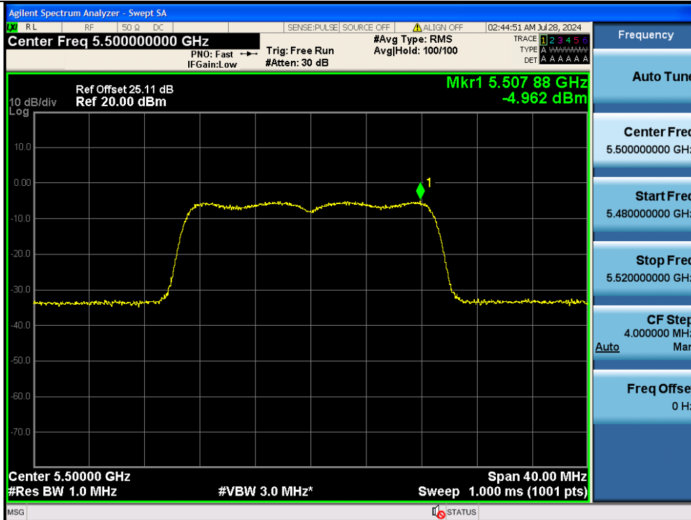
11AC20MIMO-Ant2-5500-PASS
