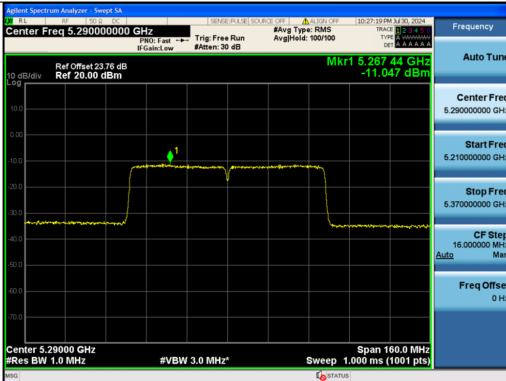
11AC80MIMO-Ant1-5530-PASS
