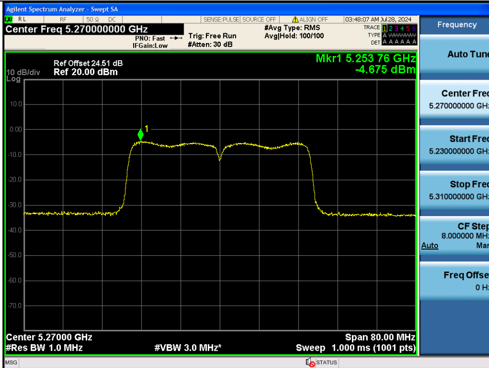
11AC40MIMO-Ant2-5270-PASS
