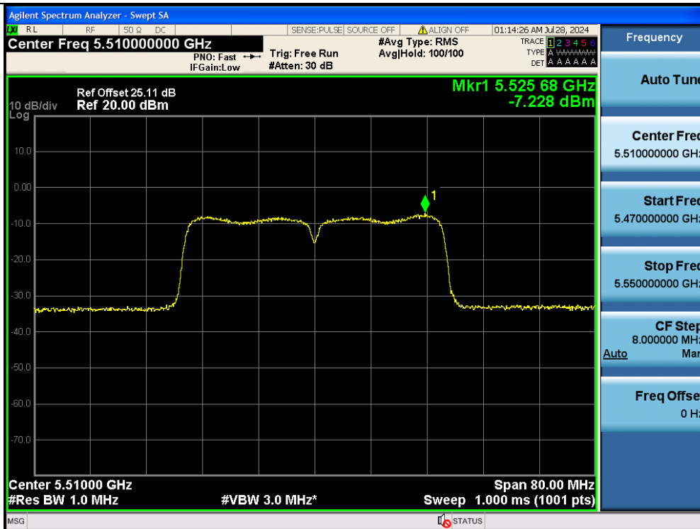
11N40MIMO-Ant2-5510-PASS
