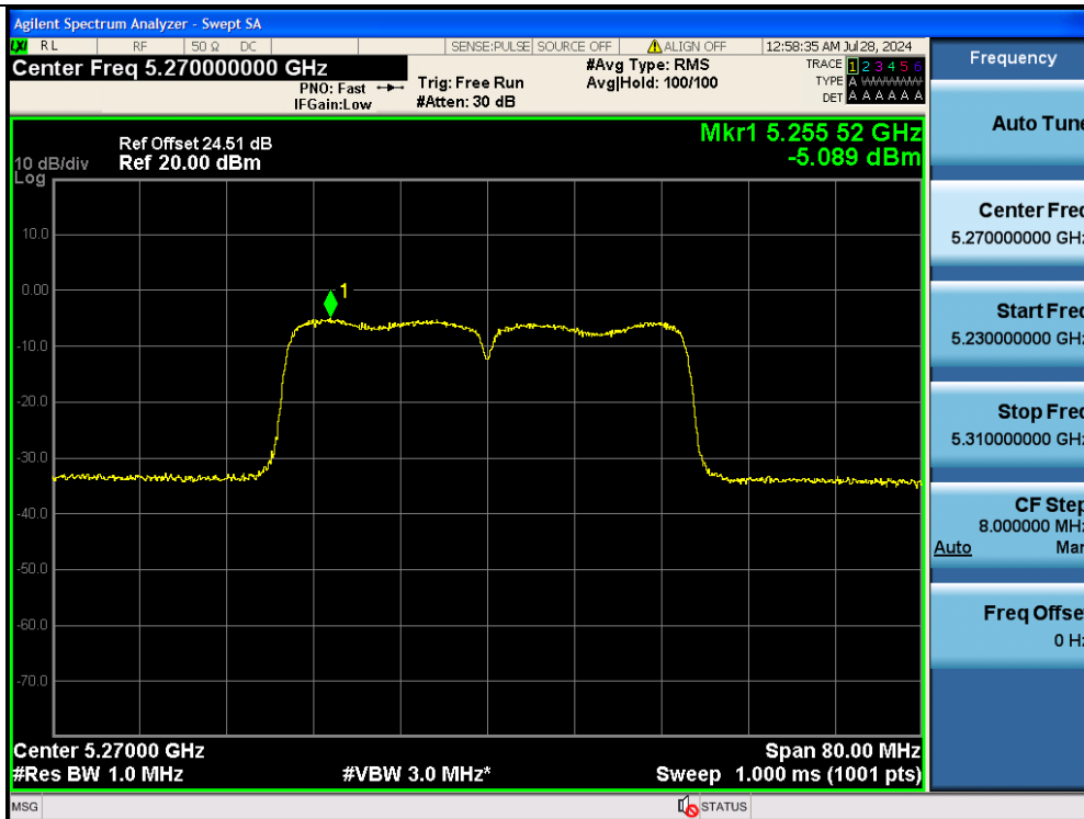
11N40MIMO-Ant2-5270-PASS
