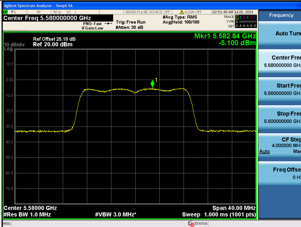
11AC20MIMO-Ant2-5580-PASS
