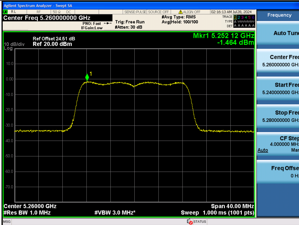
11AC20MIMO-Ant2-5260-PASS
