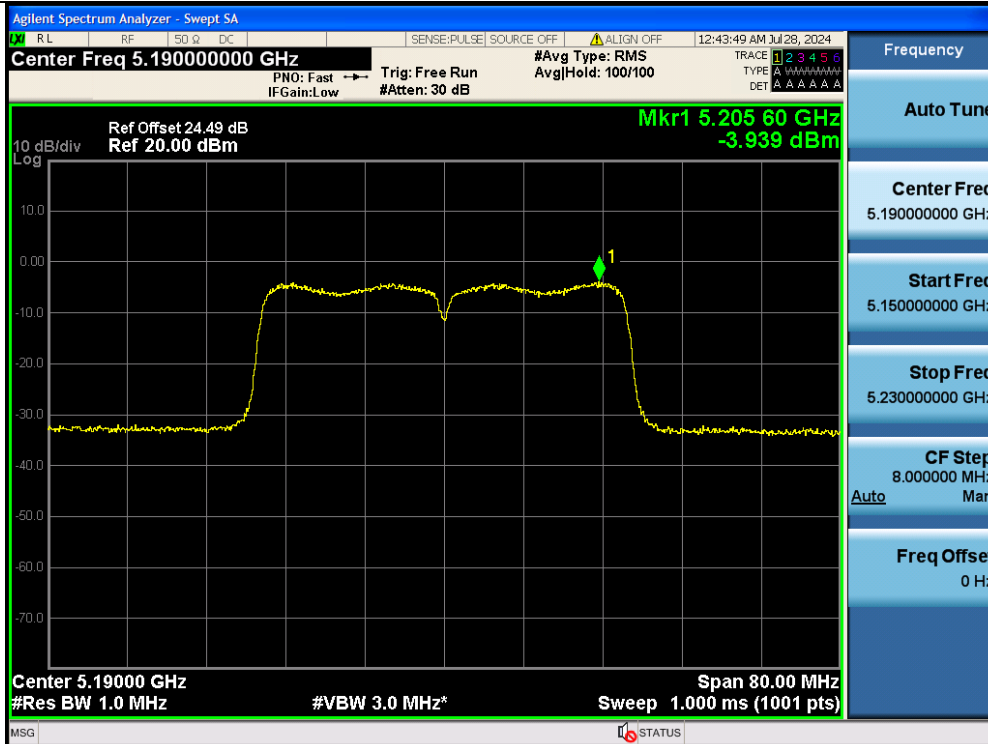
11N40MIMO-Ant2-5190-PASS
