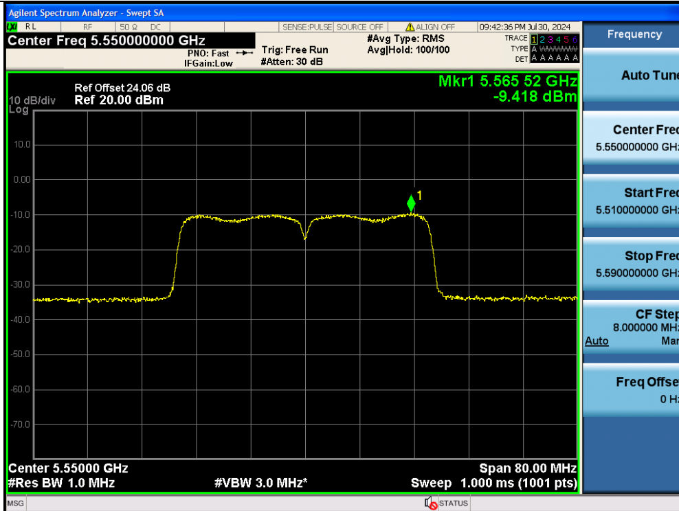
11AC40MIMO-Ant2-5550-PASS
