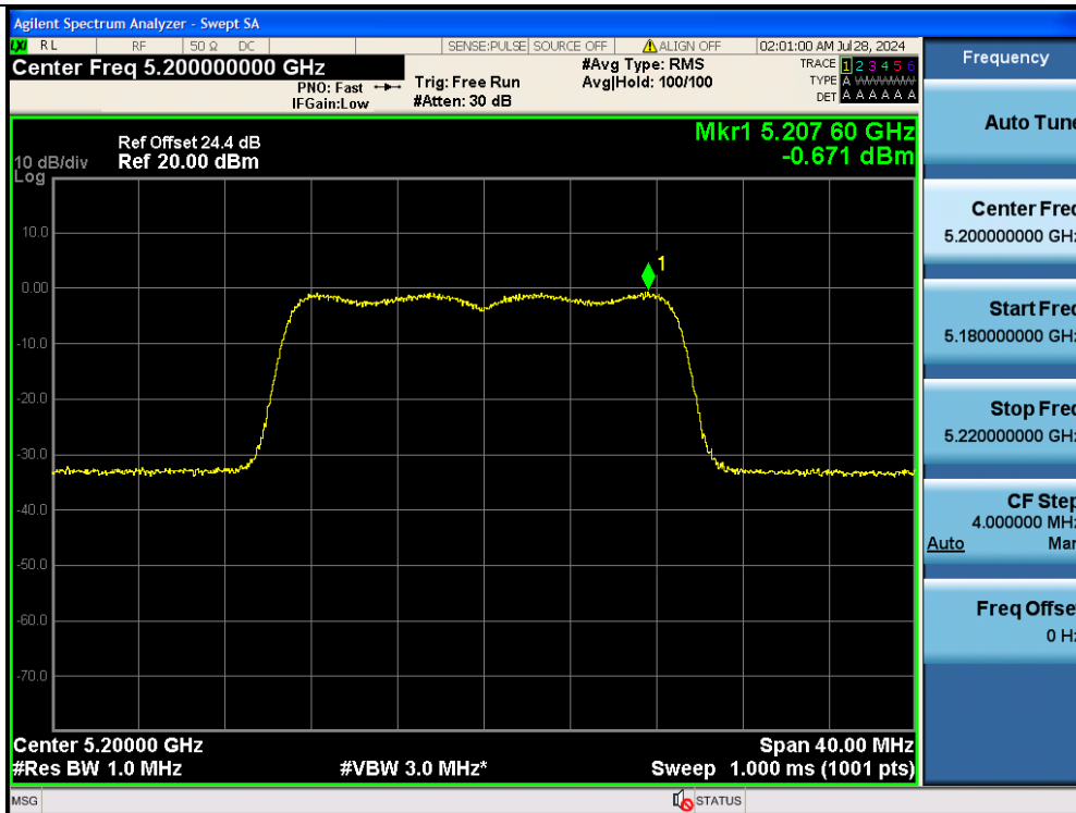
11AC20MIMO-Ant2-5200-PASS
