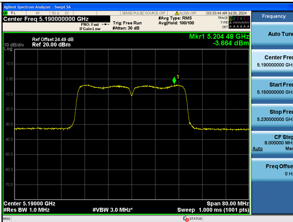
11AC40MIMO-Ant2-5190-PASS
