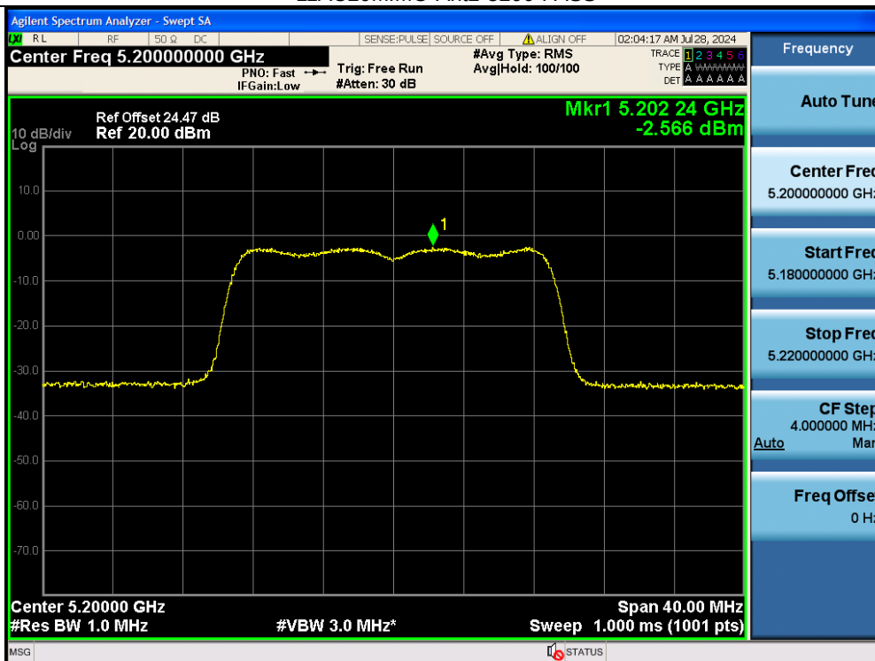
11AC20MIMO-Ant1-5240-PASS
