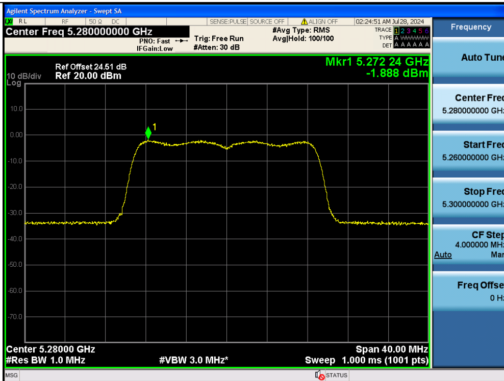
11AC20MIMO-Ant2-5280-PASS
