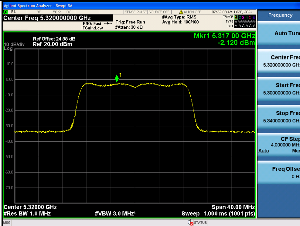
11AC20MIMO-Ant2-5320-PASS
