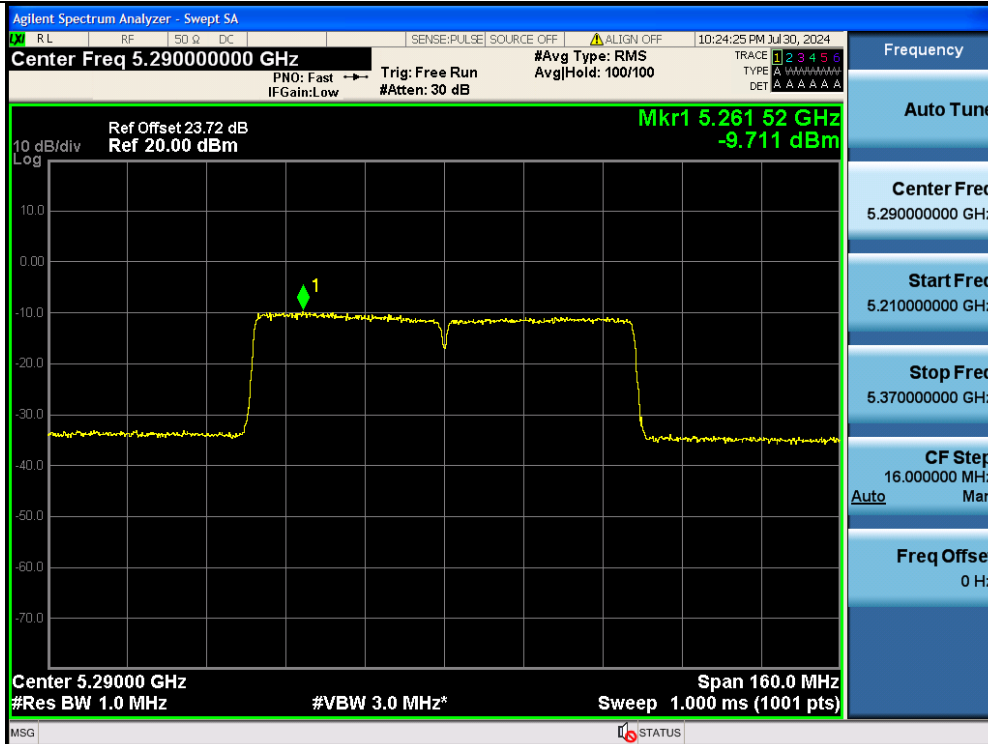
11AC80MIMO-Ant2-5290-PASS
