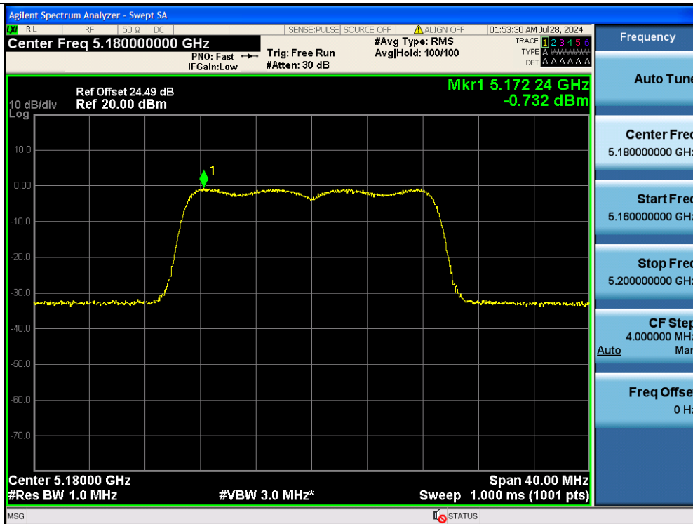
11AC20MIMO-Ant2-5180-PASS
