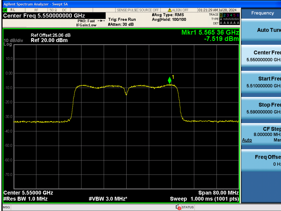
11N40MIMO-Ant2-5550-PASS
