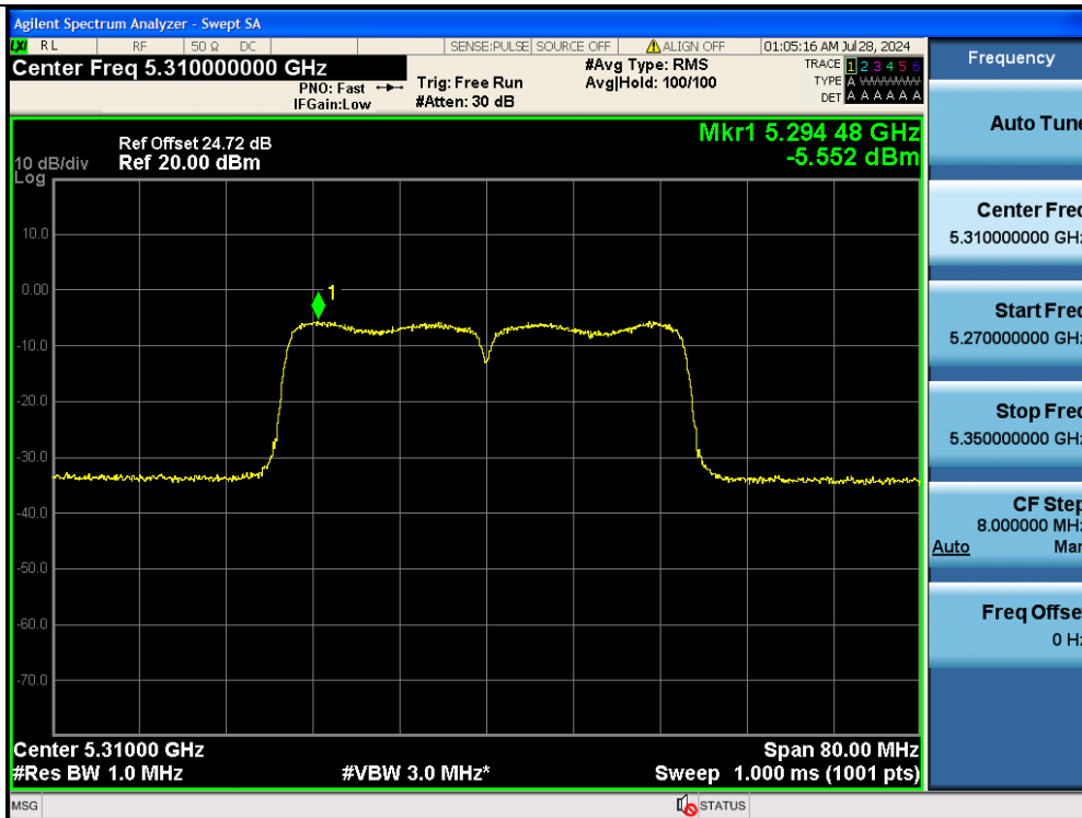
11N40MIMO-Ant2-5310-PASS
