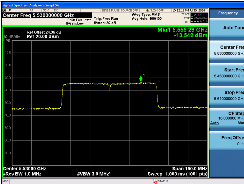
11AC80MIMO-Ant2-5530-PASS
