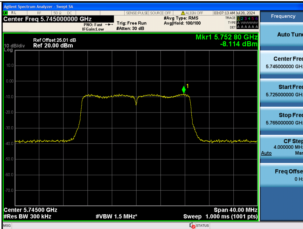
11AC20MIMO-Ant2-5745-PASS
