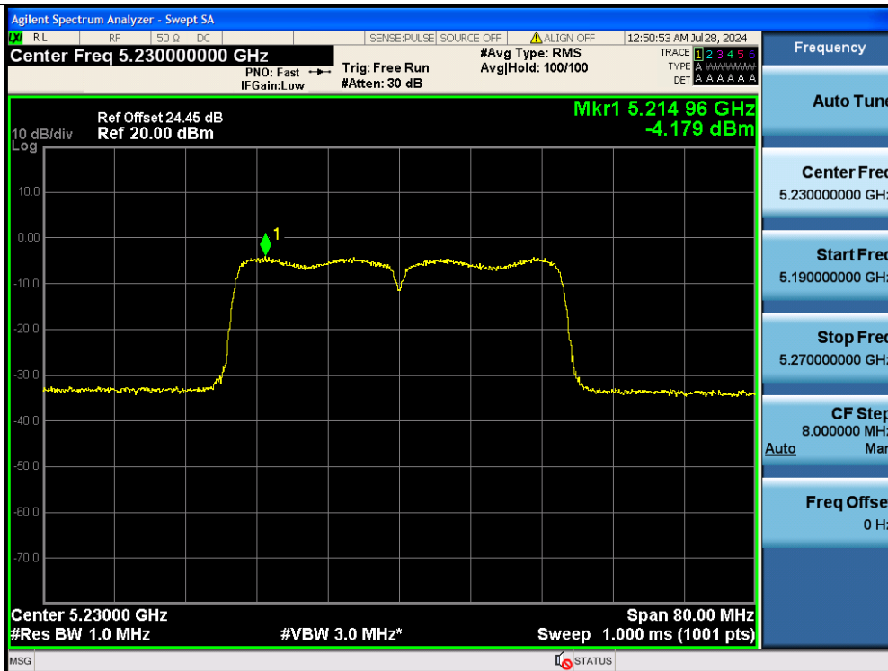
11N40MIMO-Ant2-5230-PASS
