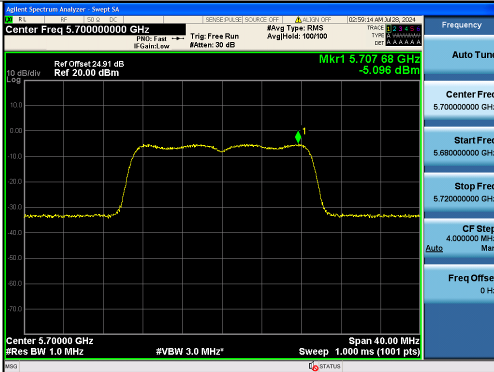
11AC20MIMO-Ant2-5700-PASS
