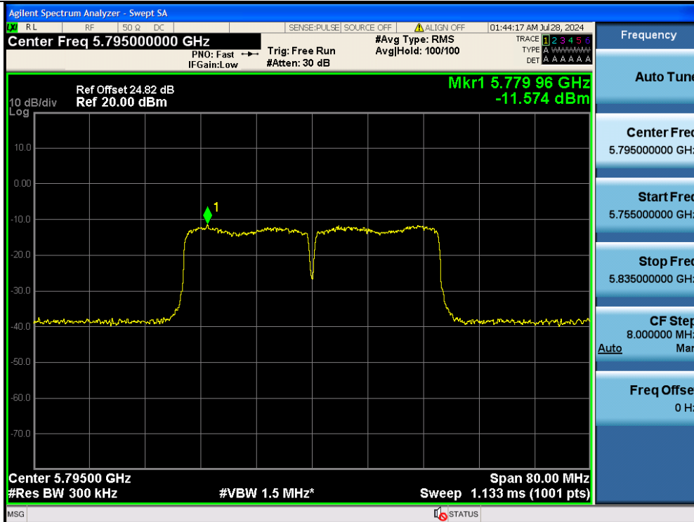
11N40MIMO-Ant2-5795-PASS
