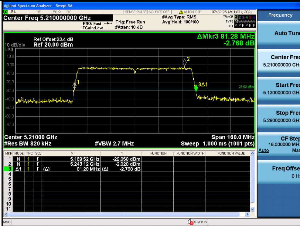
11AC80MIMO-Ant2-5210
