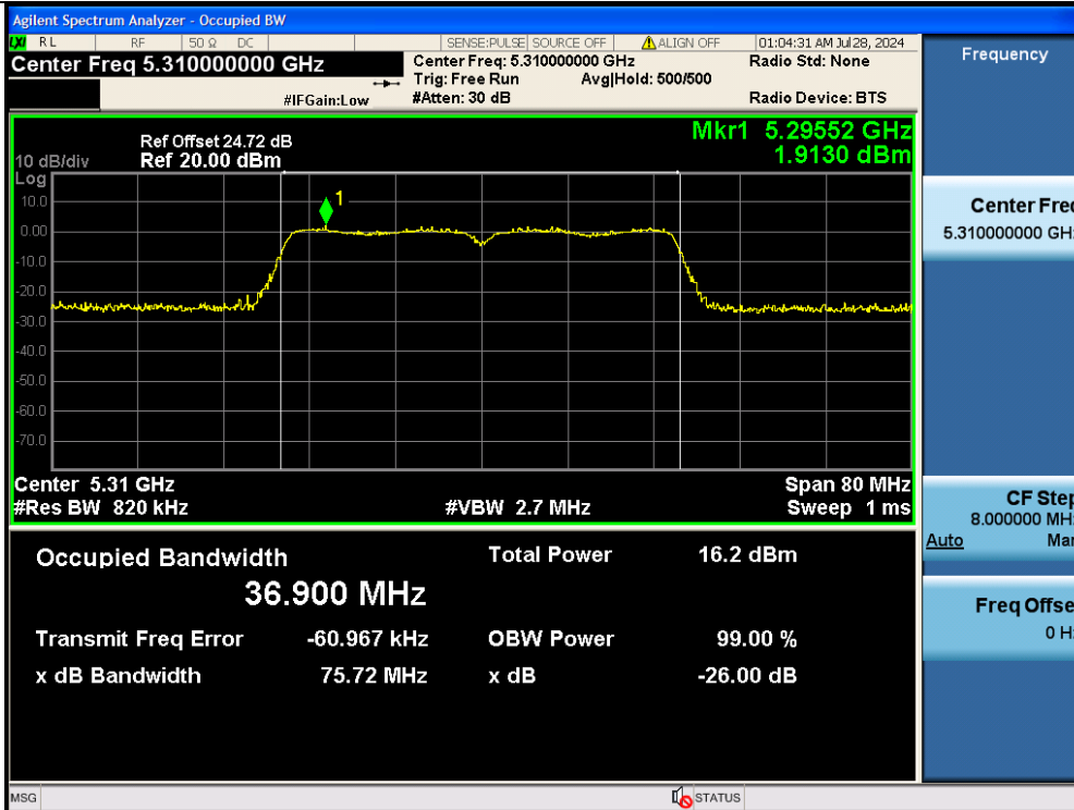
11N40MIMO-Ant2-5310
