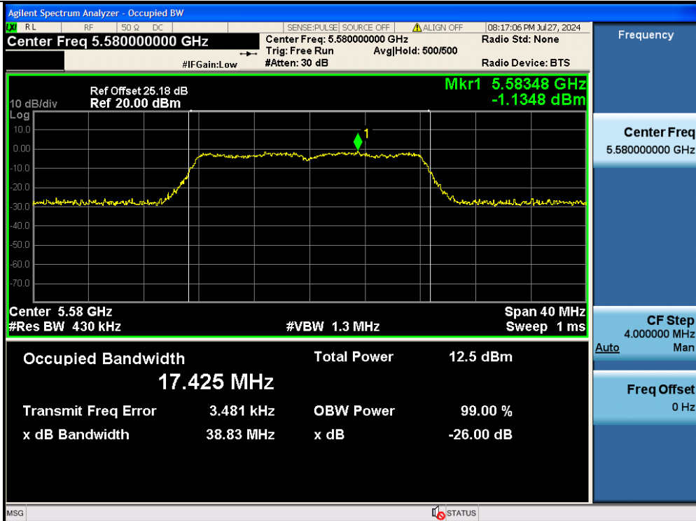
11A-Ant2-5580
