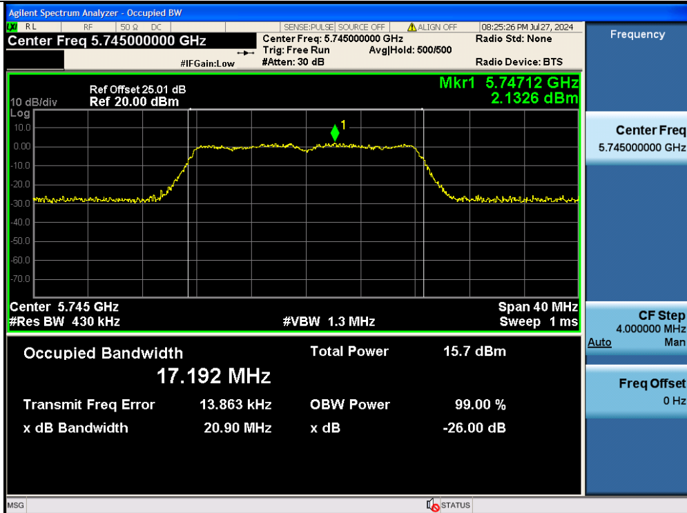
11A-Ant2-5745
