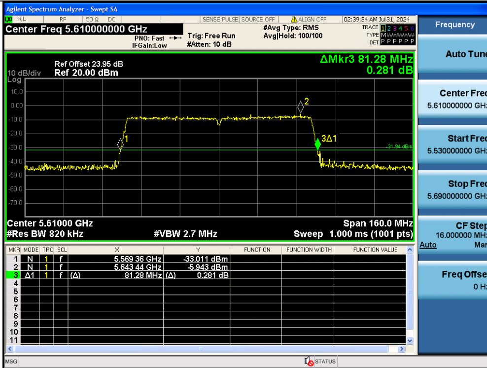
11AC80MIMO-Ant2-5610
