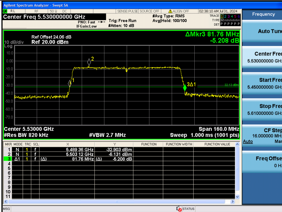
11AC80MIMO-Ant2-5530
