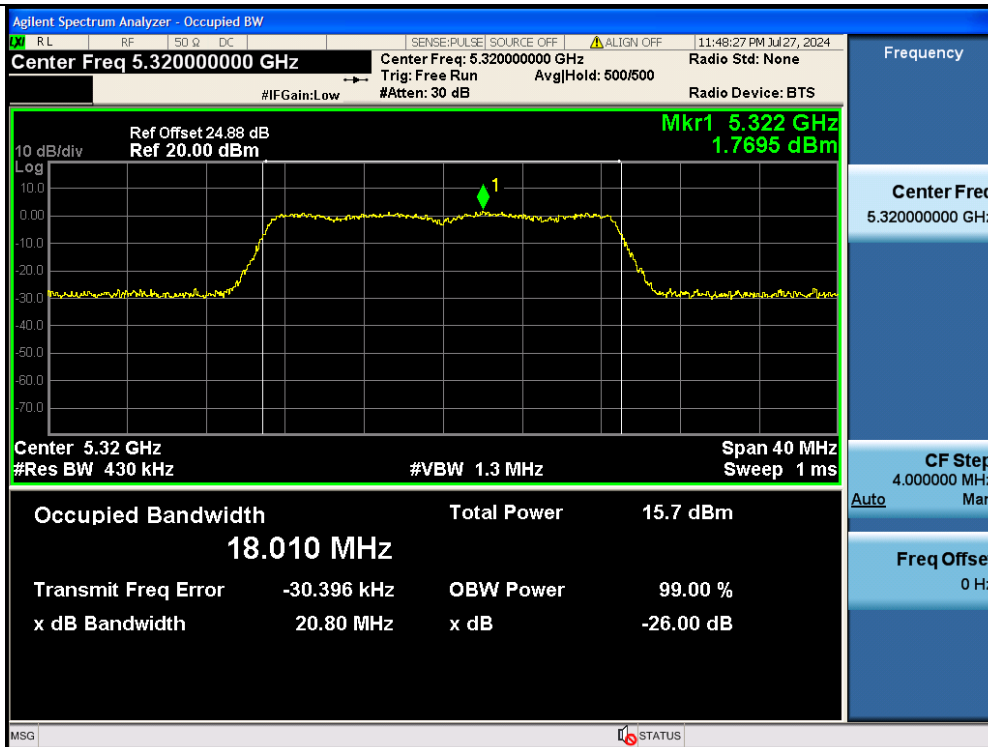
11N20MIMO-Ant2-5320
