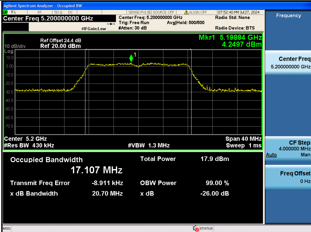
11A-Ant2-5200
