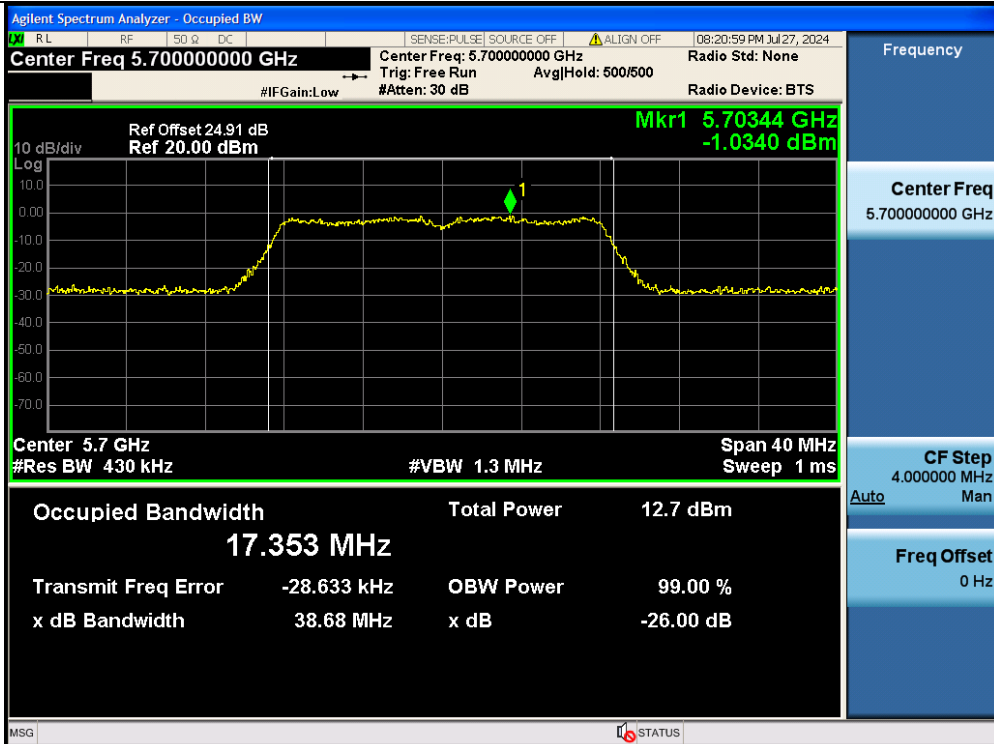
11A-Ant2-5700
