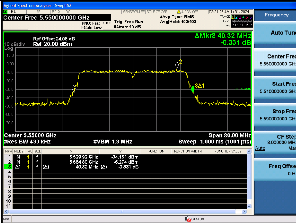
11AC40MIMO-Ant2-5550
