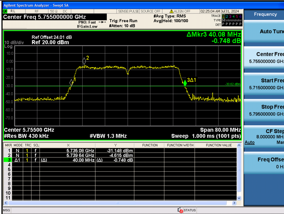
11AC40MIMO-Ant2-5755
