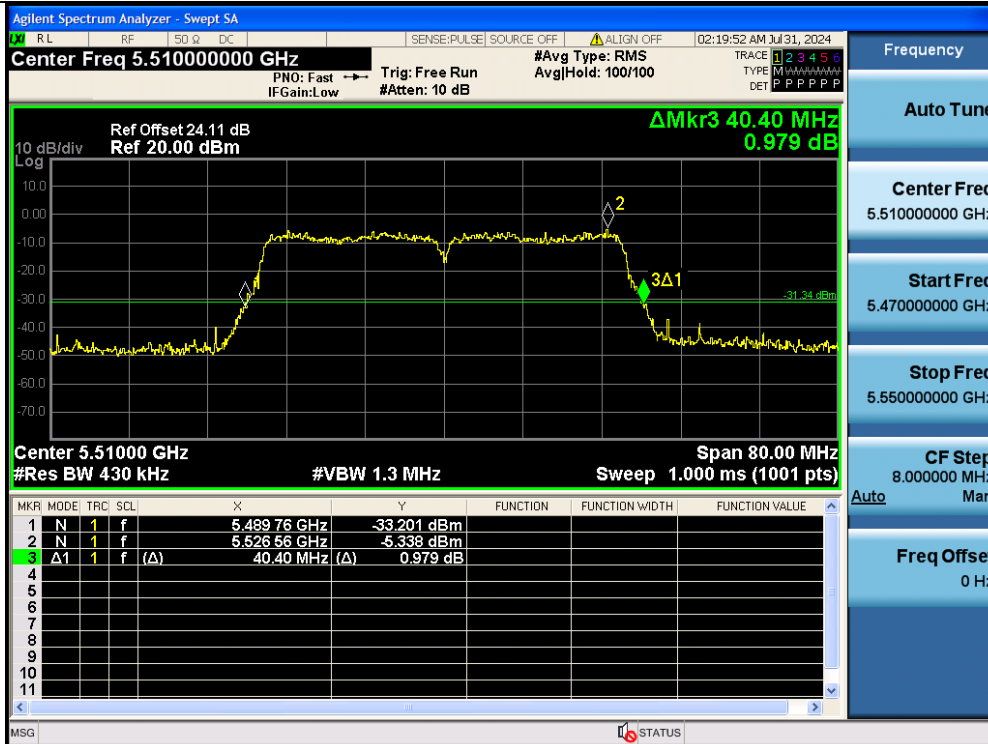
11AC40MIMO-Ant2-5510
