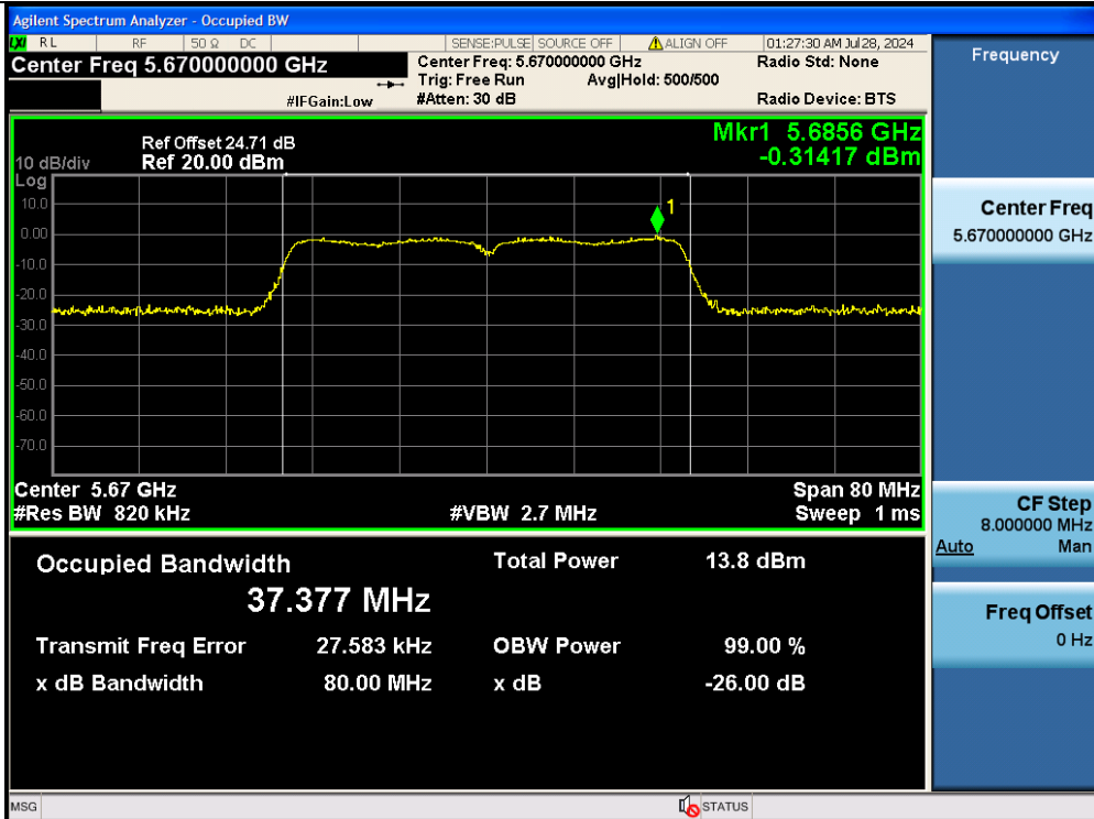
11N40MIMO-Ant2-5670
