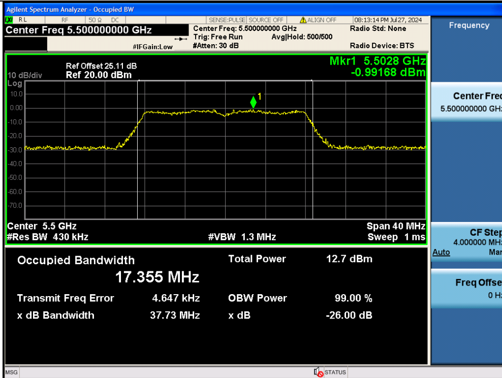
11A-Ant2-5500
