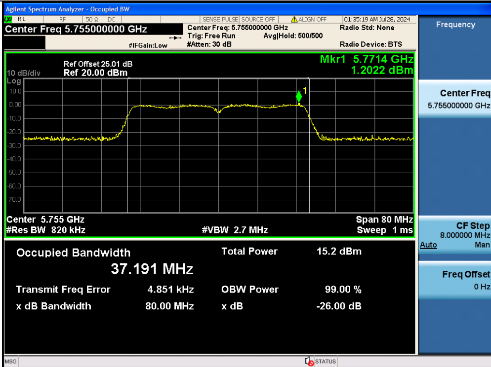
11N40MIMO-Ant2-5755
