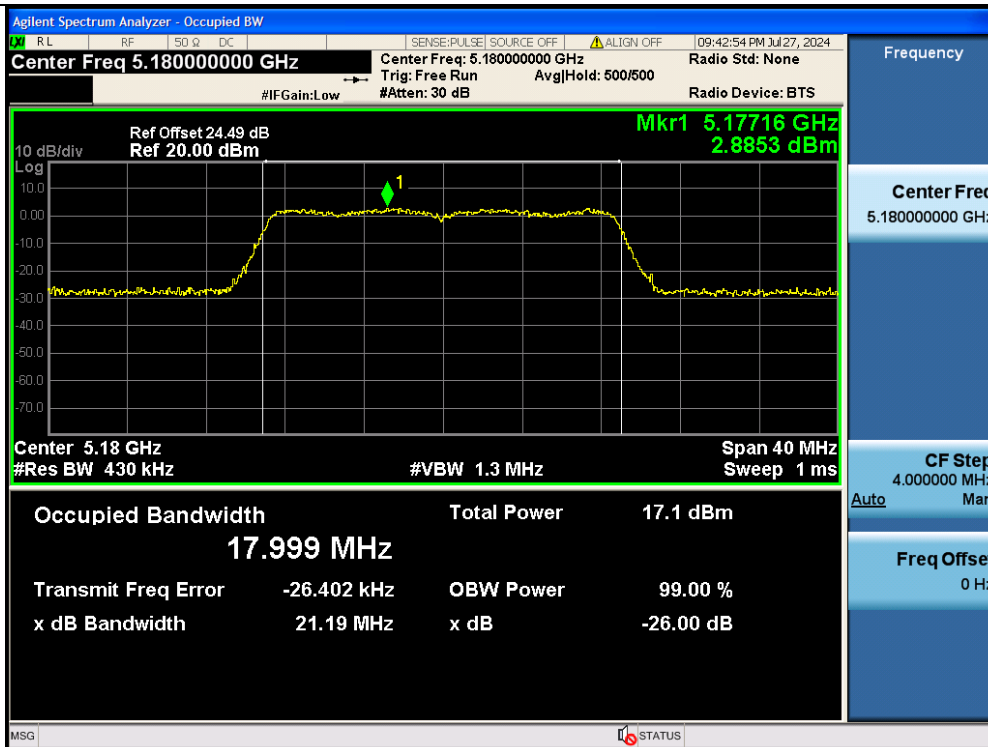
11N20MIMO-Ant2-5180
