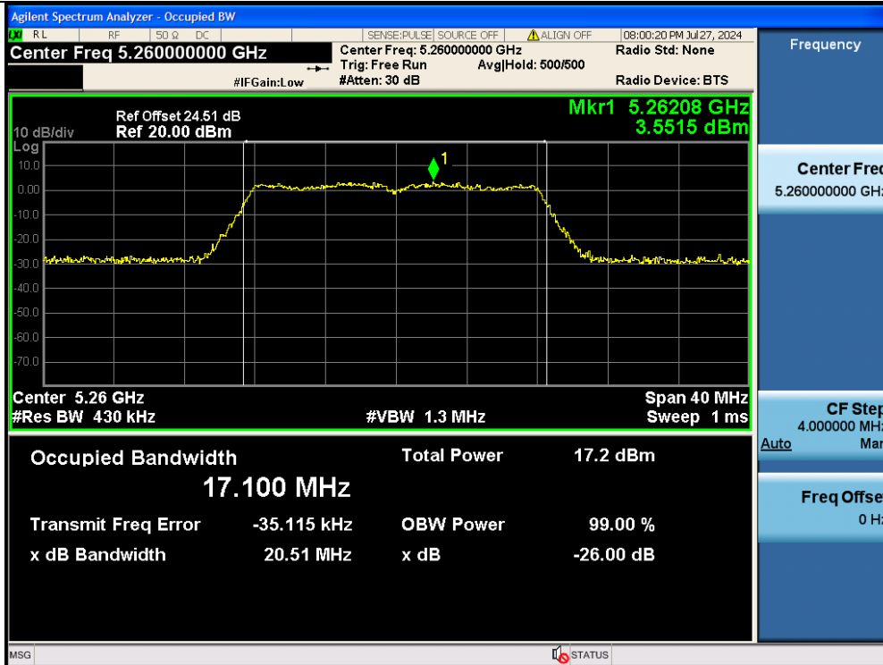
11A-Ant2-5260
