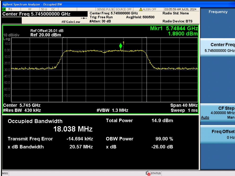
11AC20MIMO-Ant2-5745
