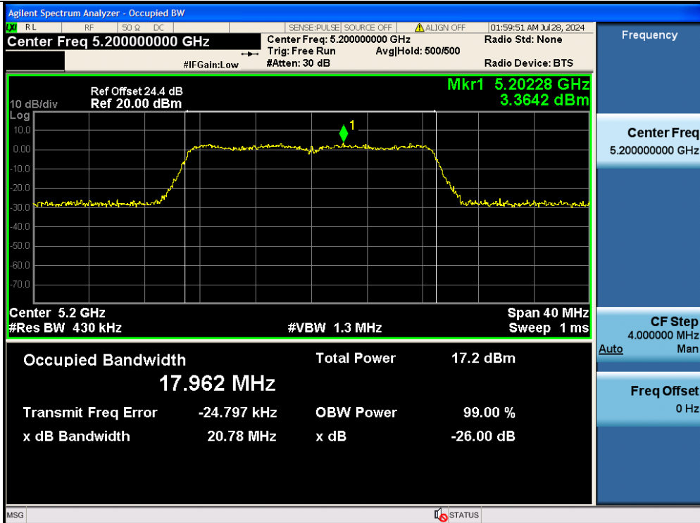
11AC20MIMO-Ant2-5200
