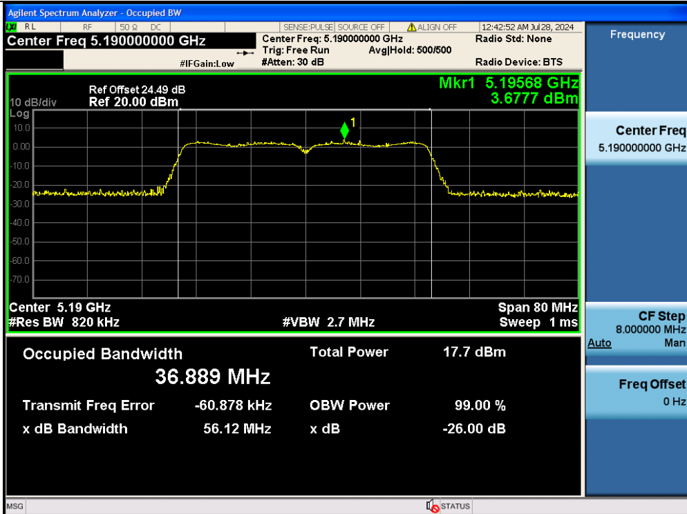
11N40MIMO-Ant2-5190
