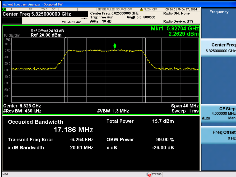
11A-Ant2-5825
