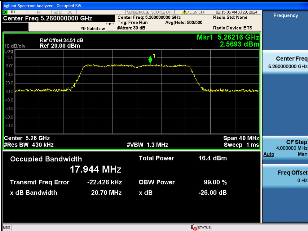
11AC20MIMO-Ant2-5260
