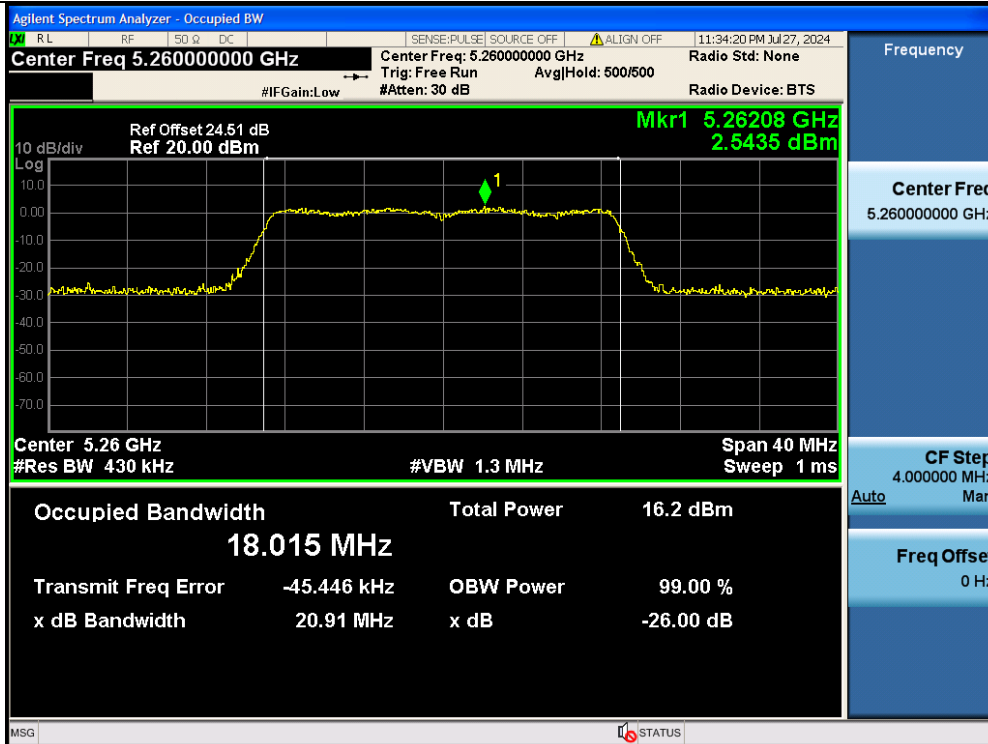
11N20MIMO-Ant2-5260
