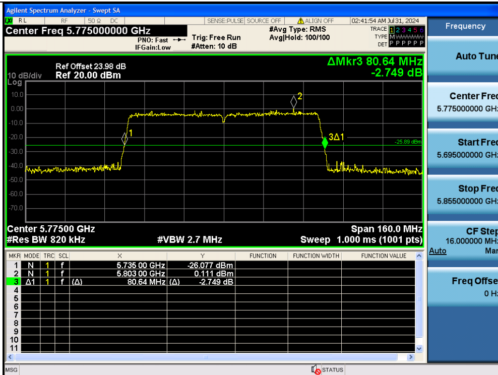
11AC80MIMO-Ant2-5775
