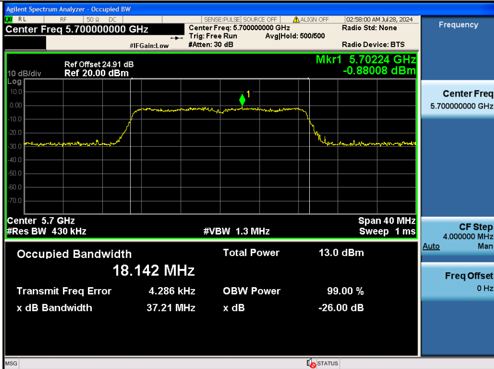
11AC20MIMO-Ant2-5700
