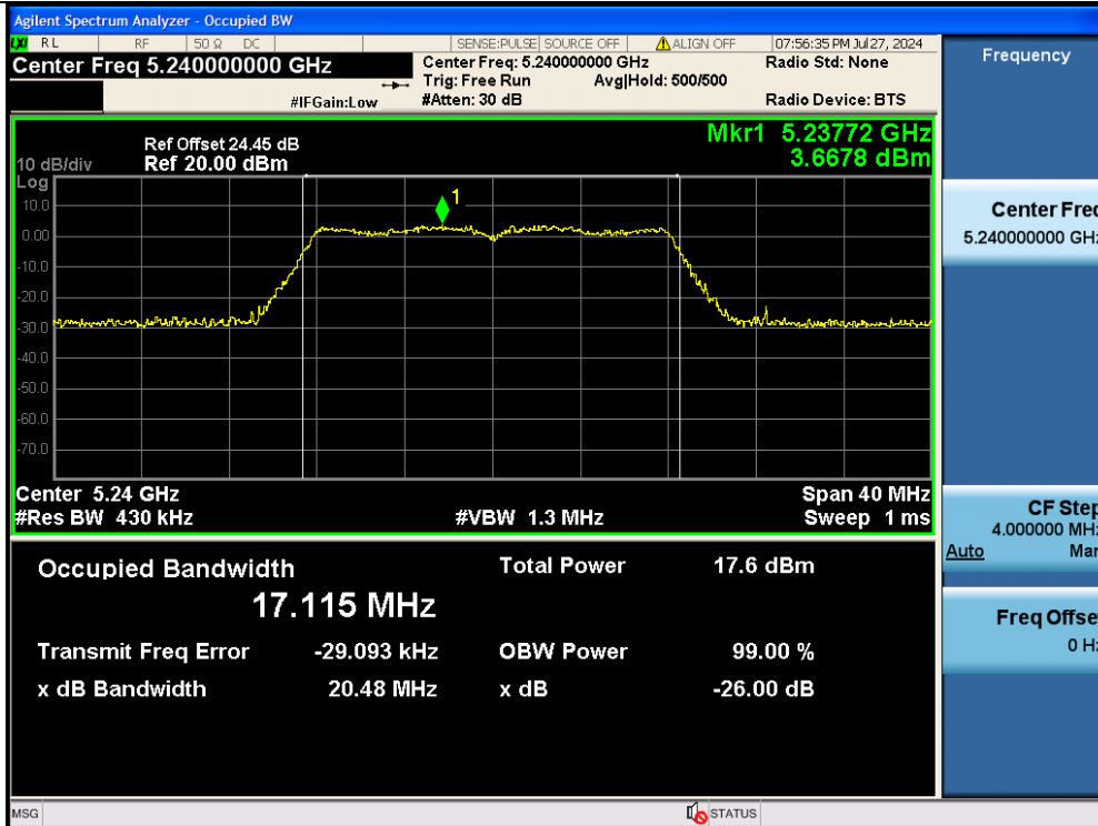
11A-Ant2-5240
