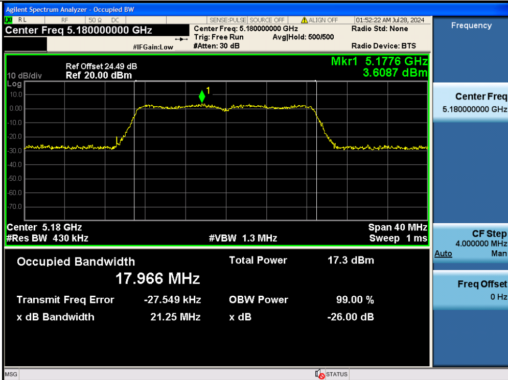
11AC20MIMO-Ant2-5180
