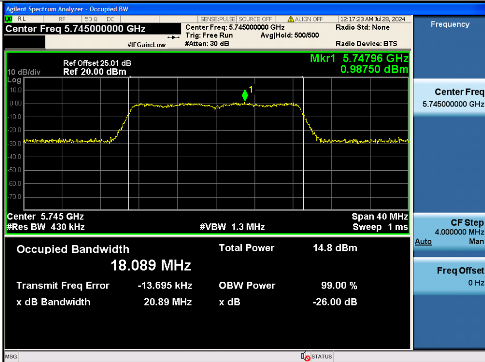
11N20MIMO-Ant2-5745
