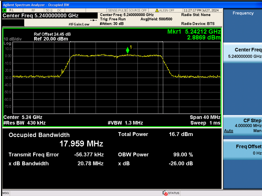
11N20MIMO-Ant2-5240
