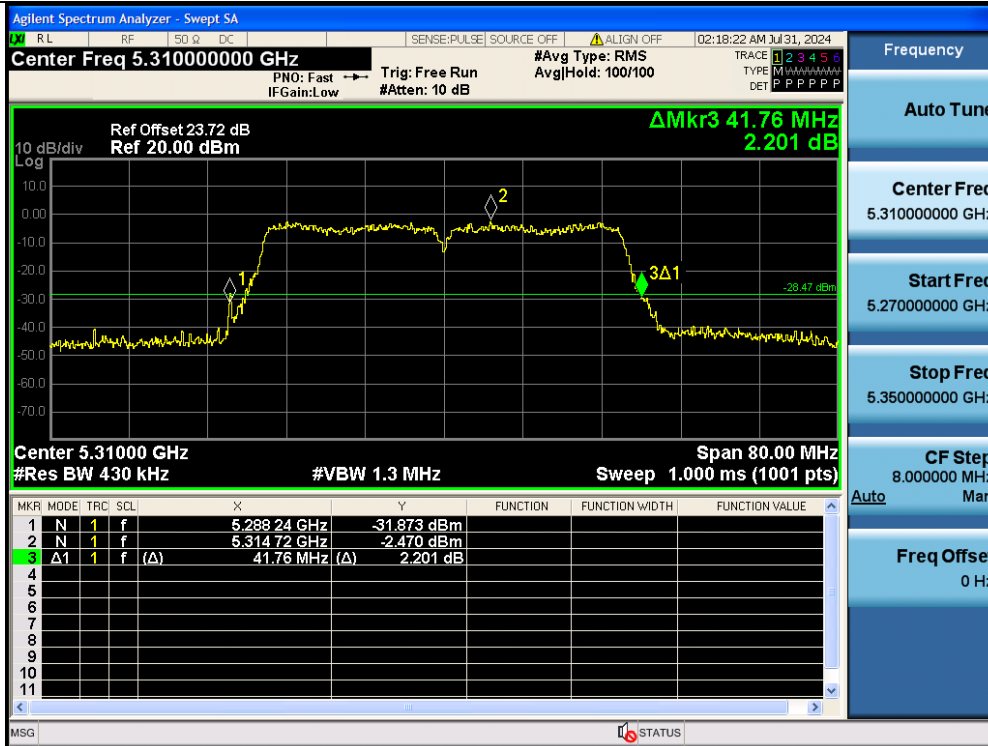
11AC40MIMO-Ant2-5310
