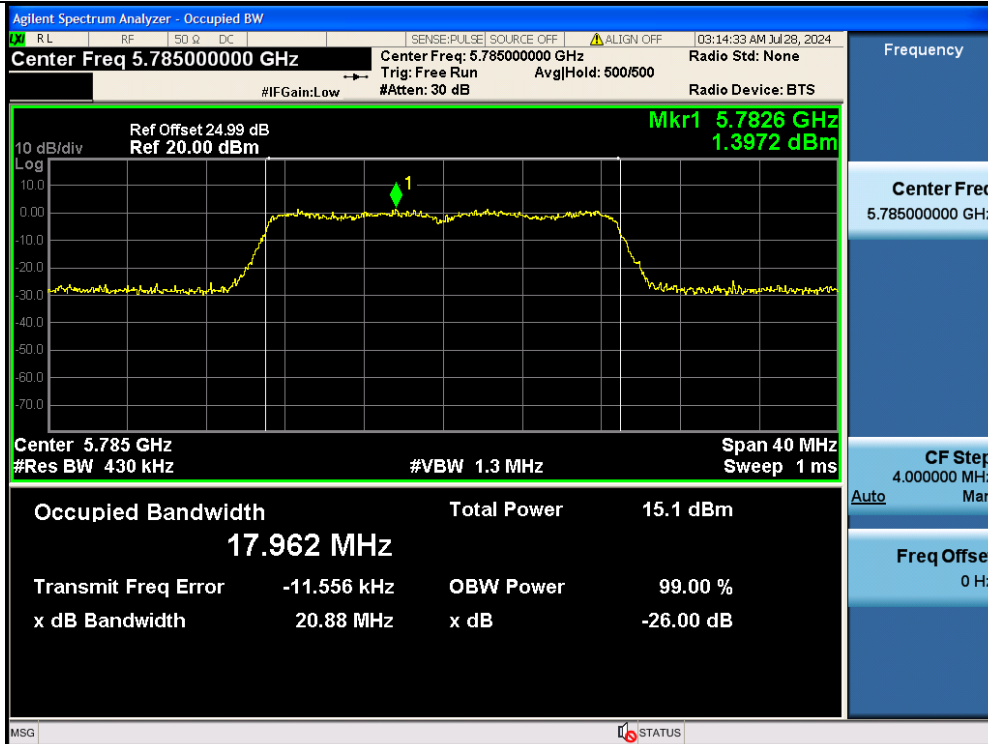
11AC20MIMO-Ant2-5785
