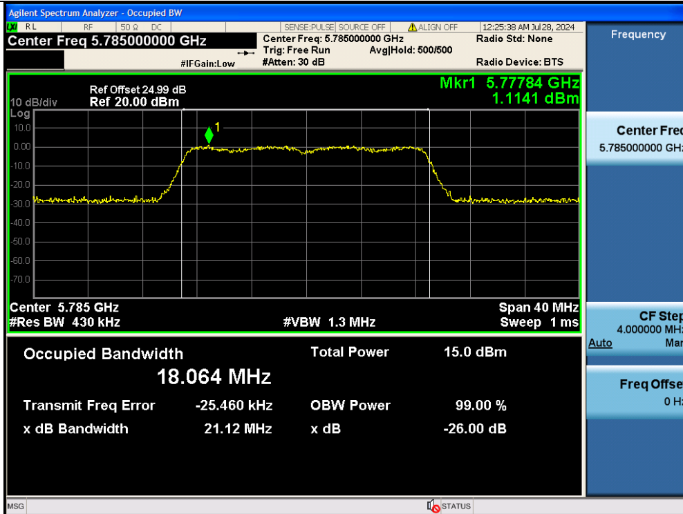
11N20MIMO-Ant2-5785
