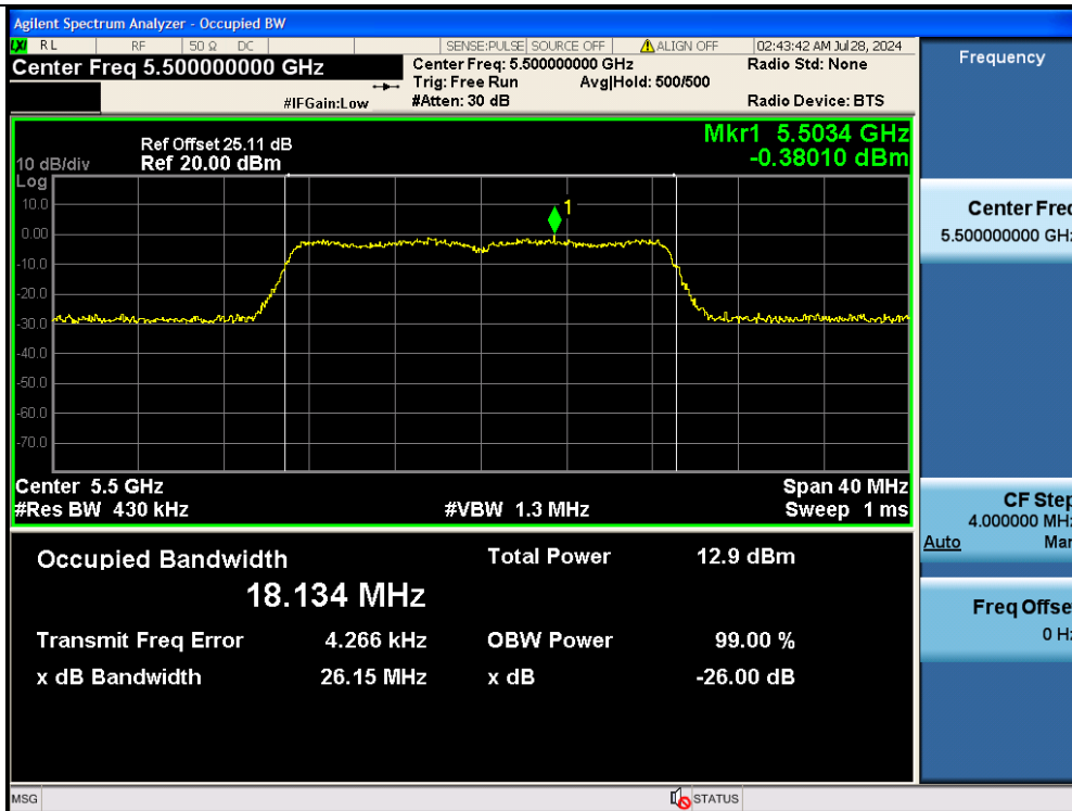
11AC20MIMO-Ant2-5500
