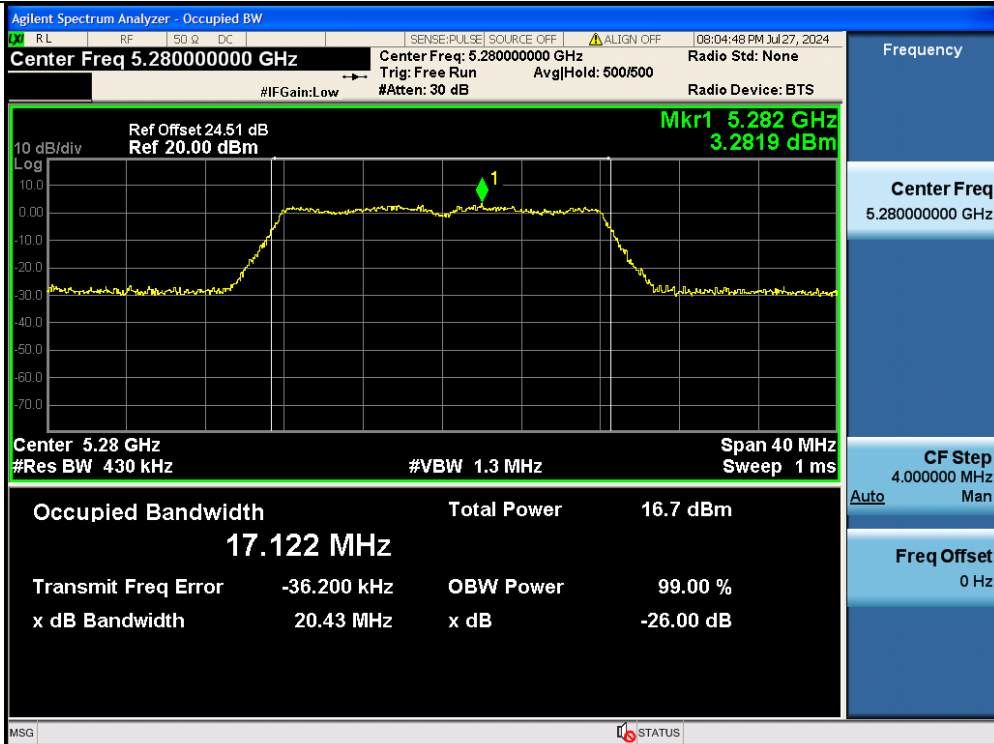
11A-Ant2-5280
