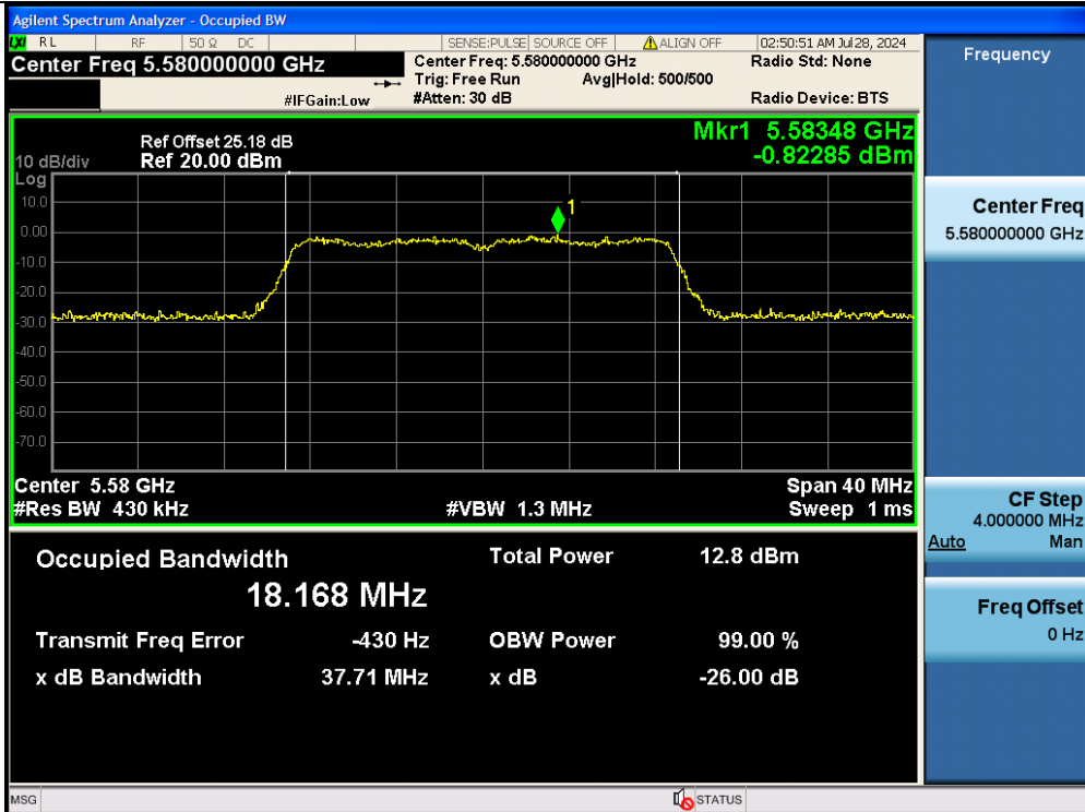
11AC20MIMO-Ant2-5580
