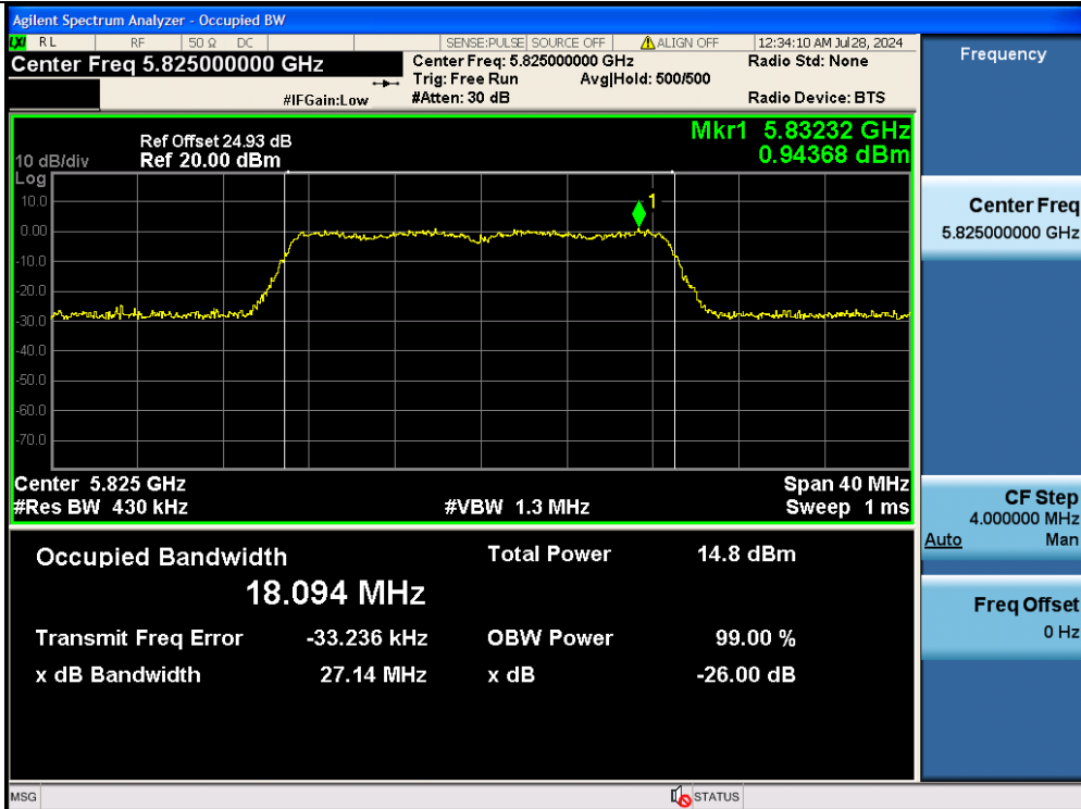
11N20MIMO-Ant2-5825
