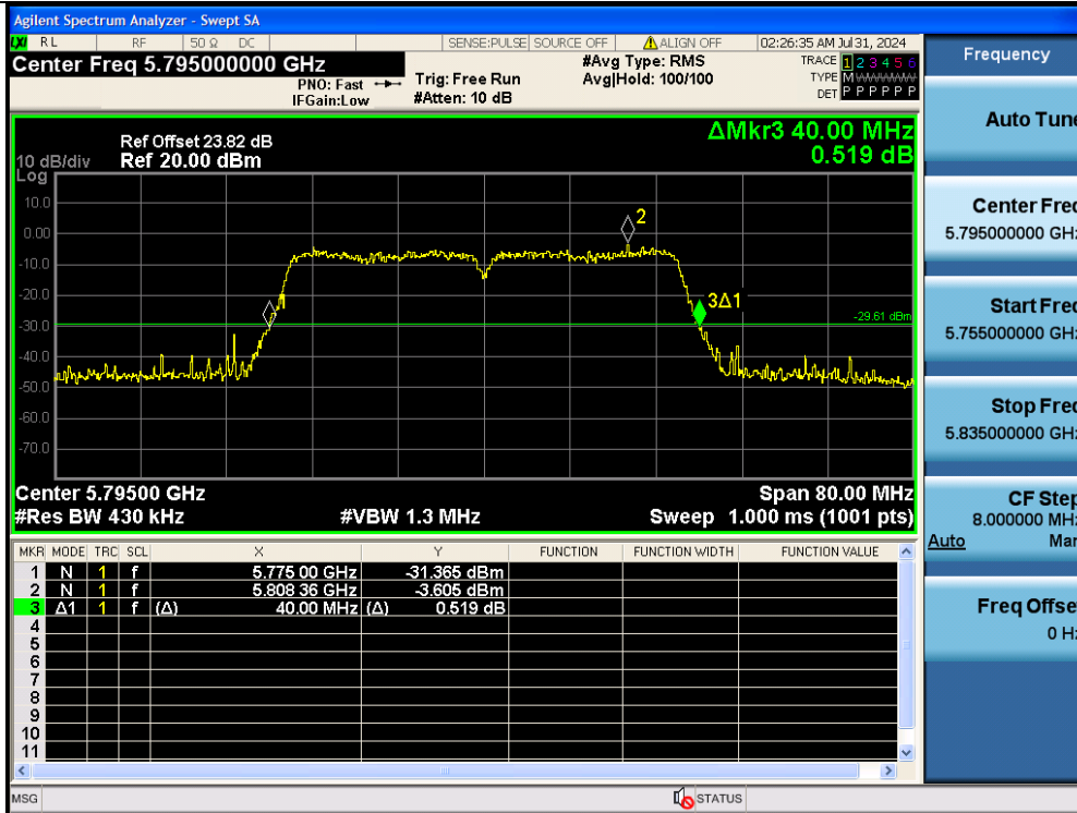
11AC40MIMO-Ant2-5795
