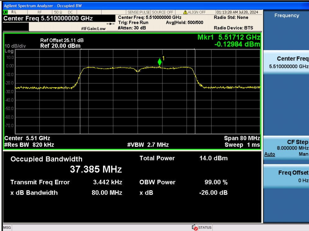
11N40MIMO-Ant2-5510
