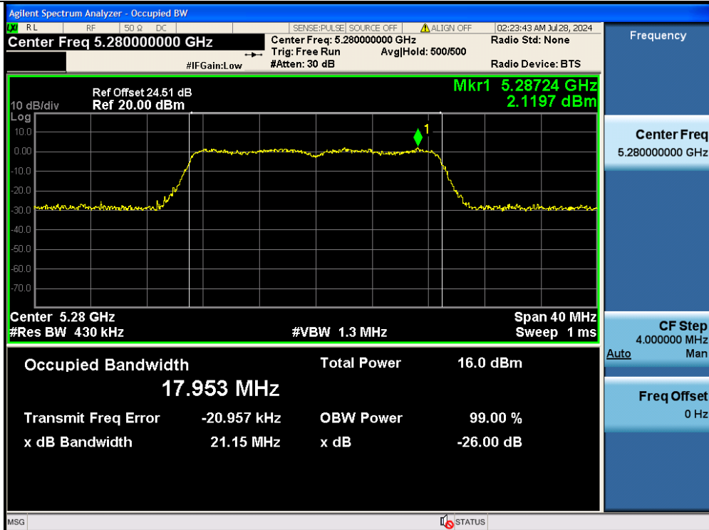
11AC20MIMO-Ant2-5280
