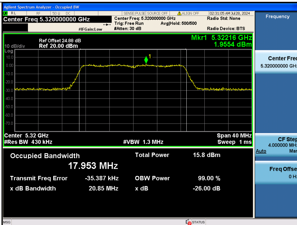
11AC20MIMO-Ant2-5320
