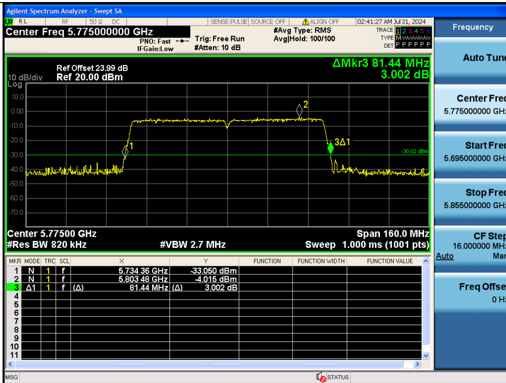
11AC80MIMO-Ant2-5775
