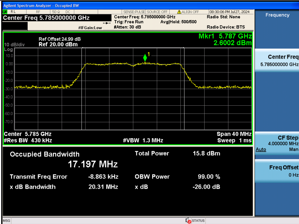
11A-Ant2-5785
