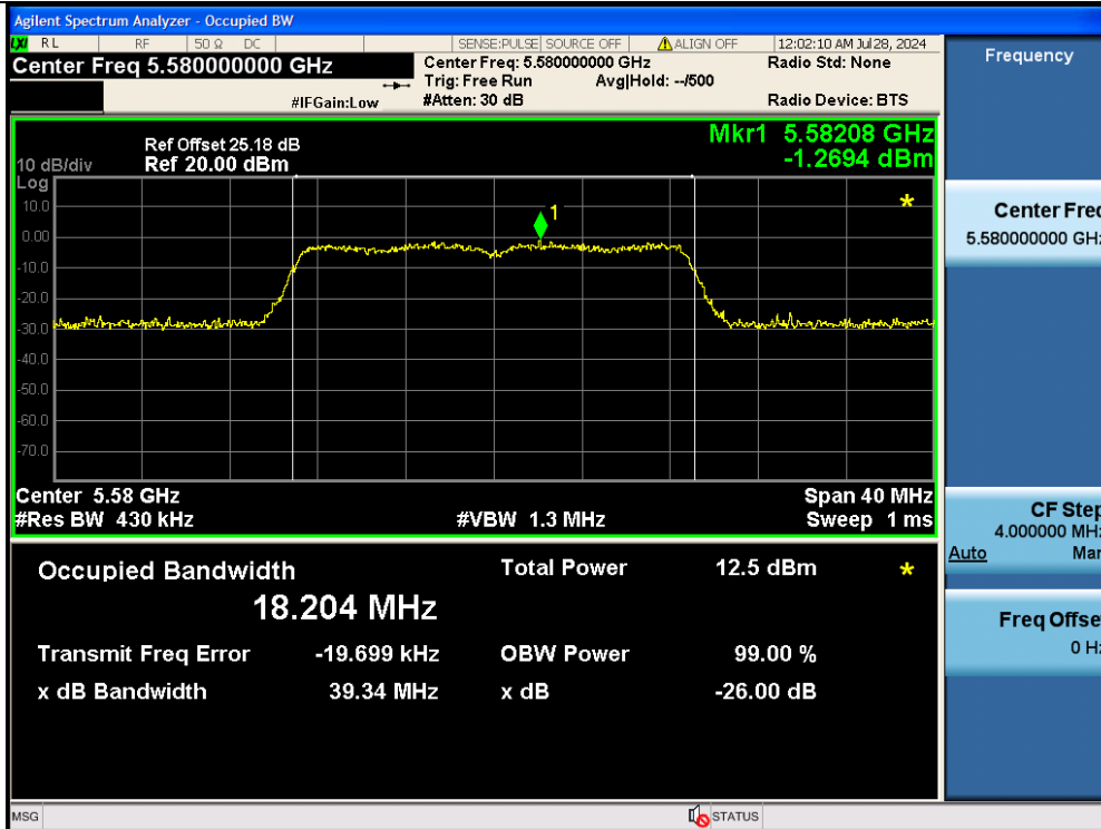
11N20MIMO-Ant2-5580
