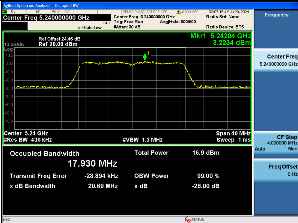
11AC20MIMO-Ant2-5240
