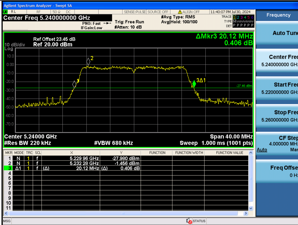
11N20MIMO-Ant2-5240
