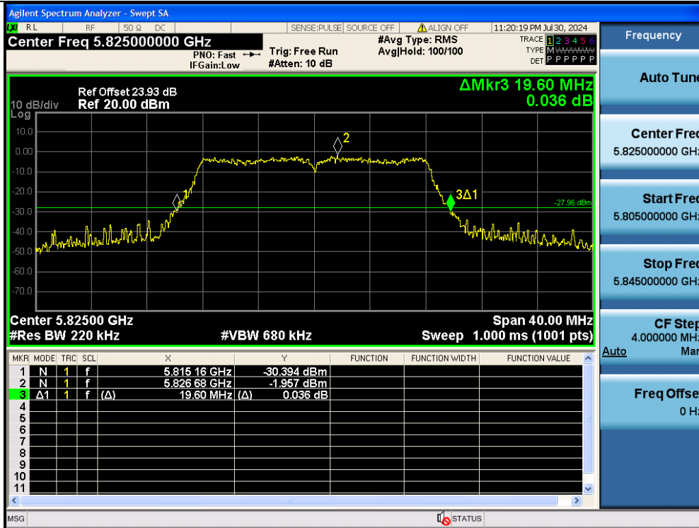
11A-Ant2-5825
