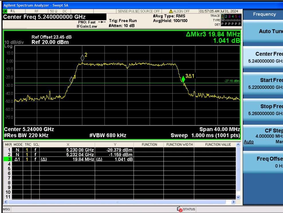
11AC20MIMO-Ant2-5240
