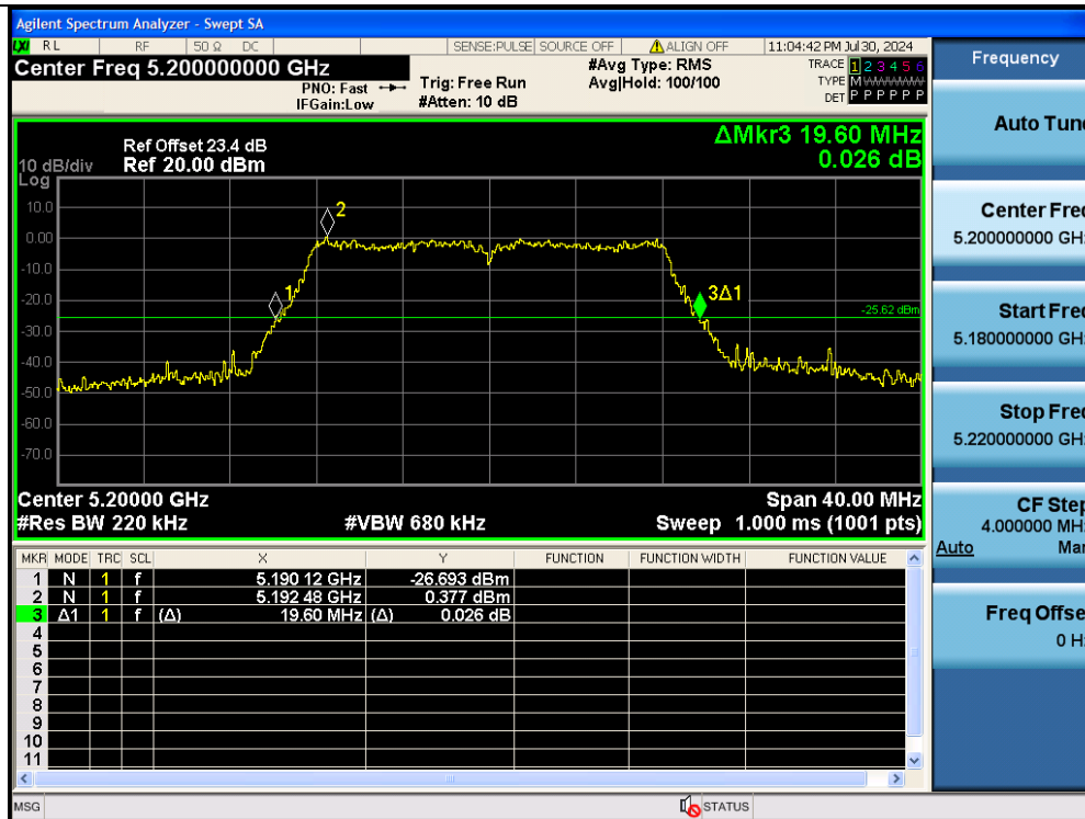
11A-Ant2-5200
