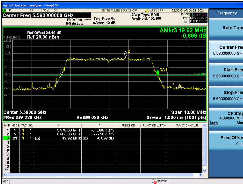
11AC20MIMO-Ant2-5580
