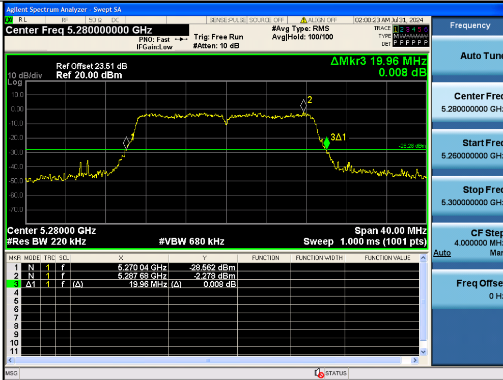
11AC20MIMO-Ant2-5280
