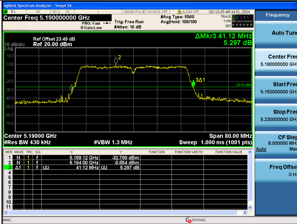
11AC40MIMO-Ant2-5190
