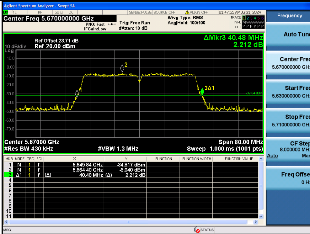
11N40MIMO-Ant2-5670
