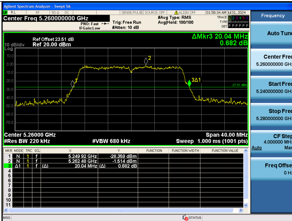
11AC20MIMO-Ant2-5260
