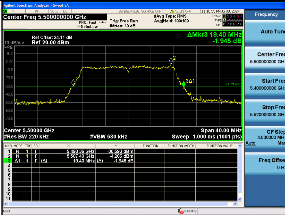
11A-Ant2-5500
