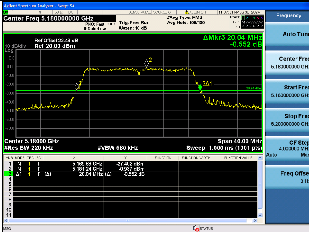
11N20MIMO-Ant2-5180
