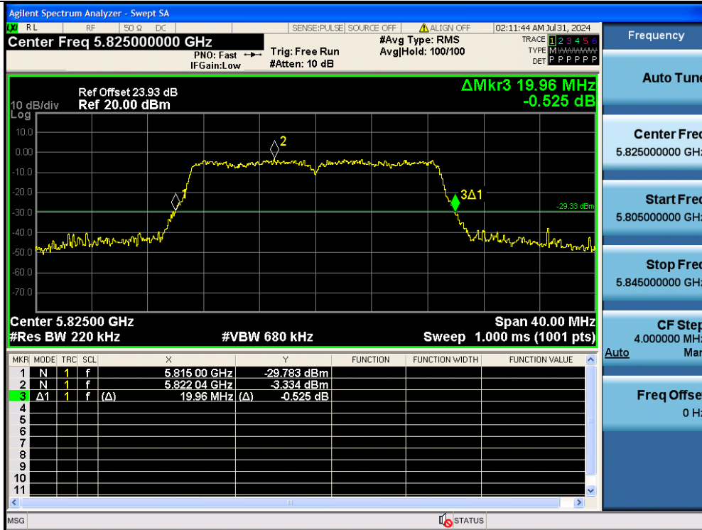
11AC20MIMO-Ant2-5825
