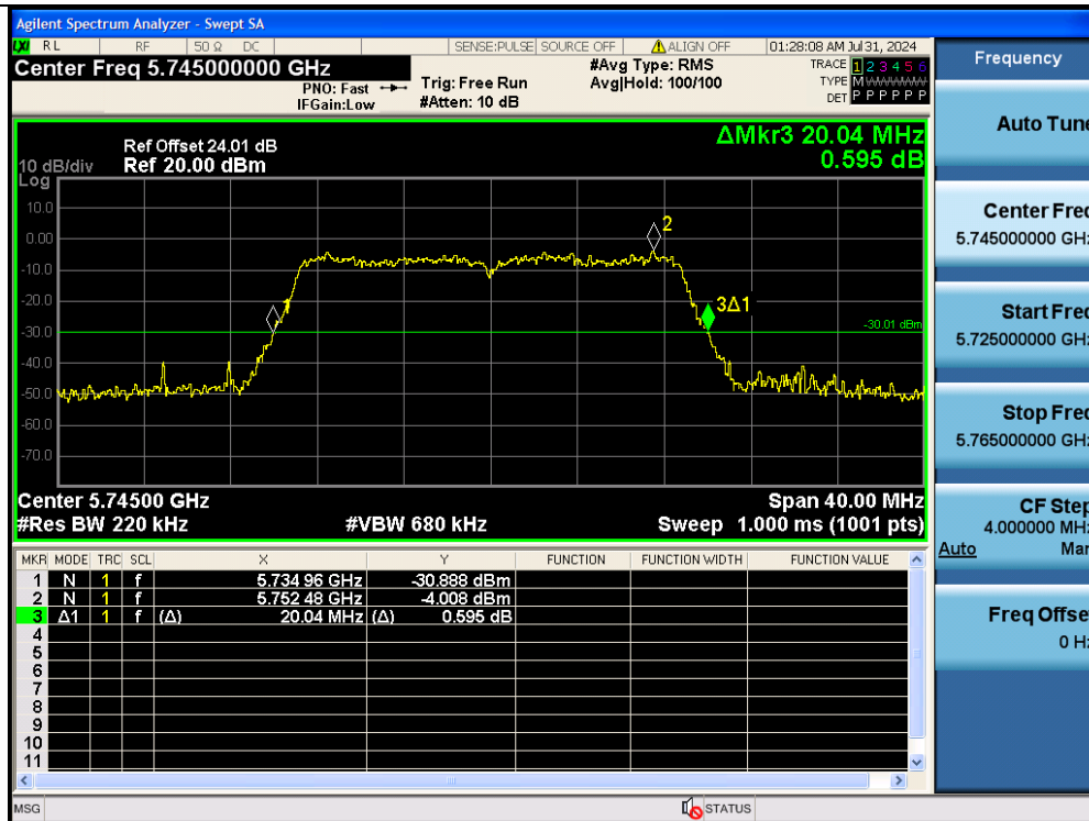
11N20MIMO-Ant2-5745
