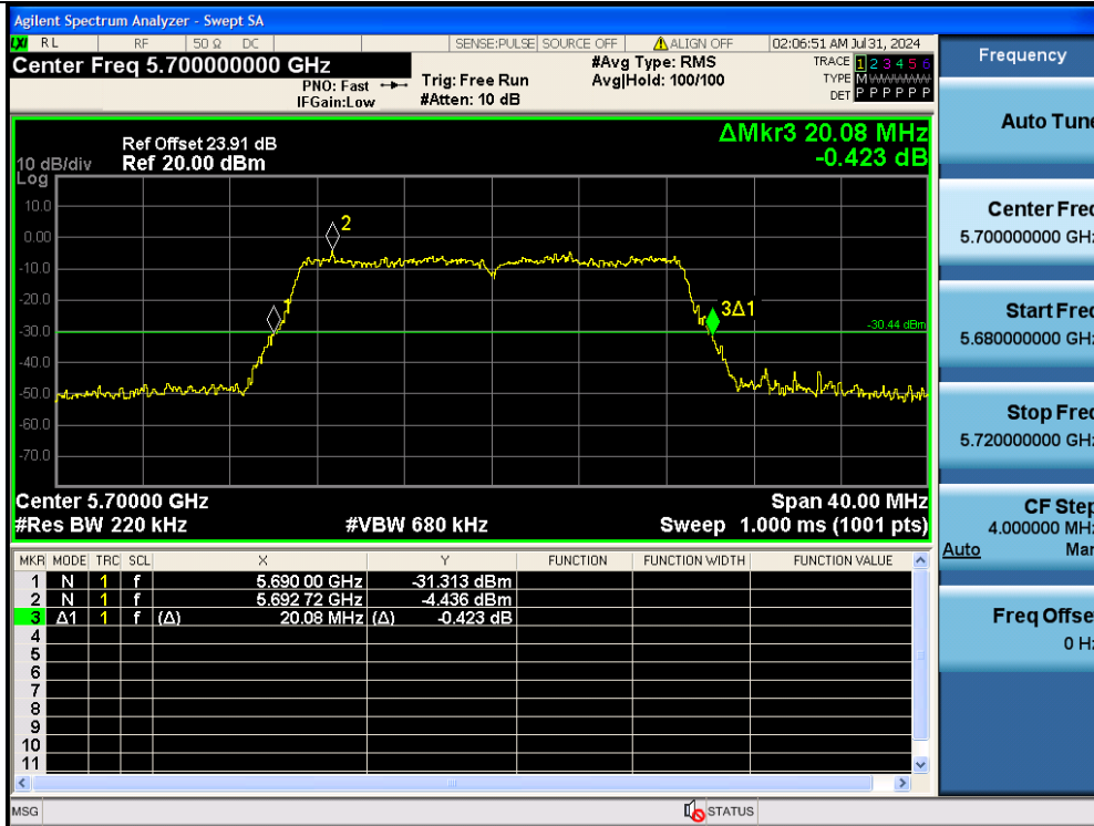
11AC20MIMO-Ant2-5700
