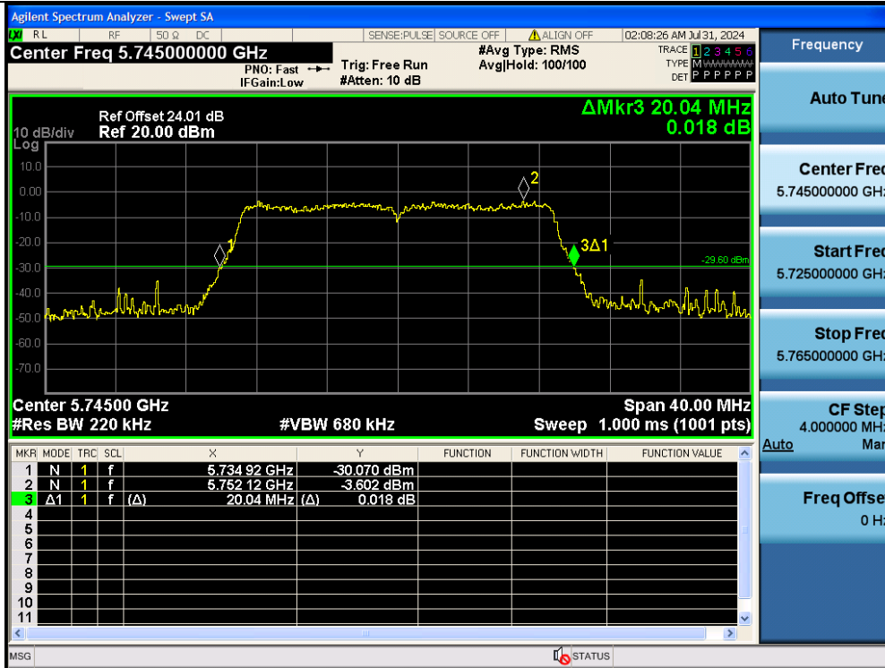
11AC20MIMO-Ant2-5745
