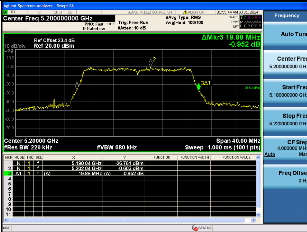
11AC20MIMO-Ant2-5200
