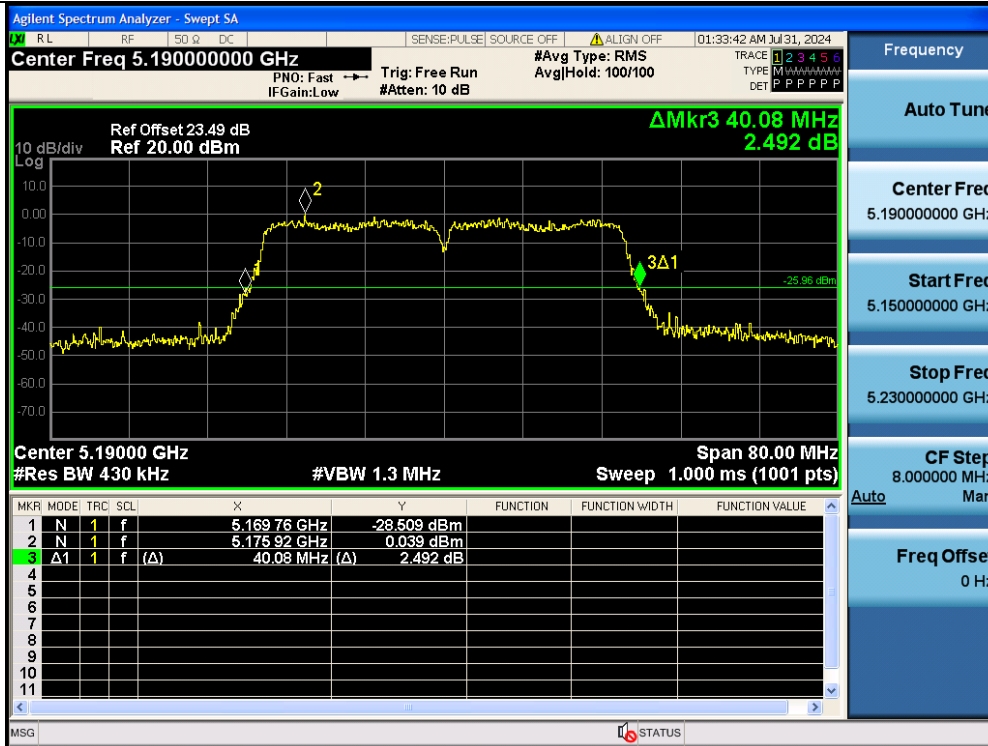
11N40MIMO-Ant2-5190
