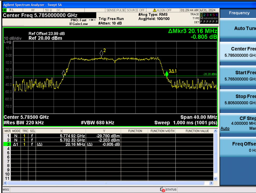
11N20MIMO-Ant2-5785
