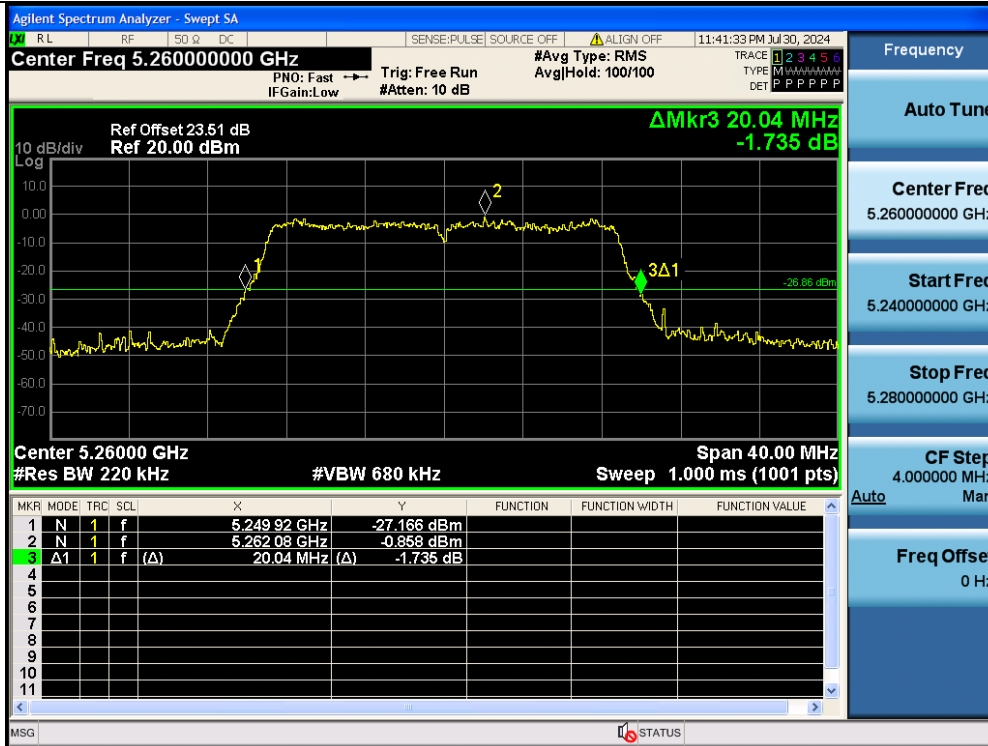
11N20MIMO-Ant2-5260
