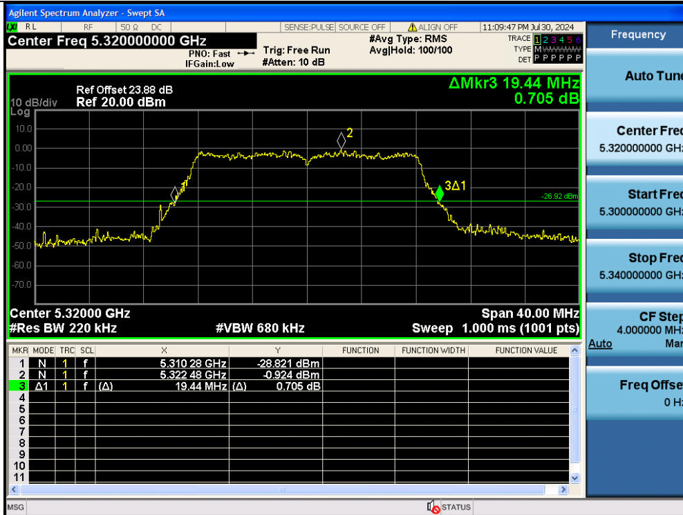
11A-Ant2-5320
