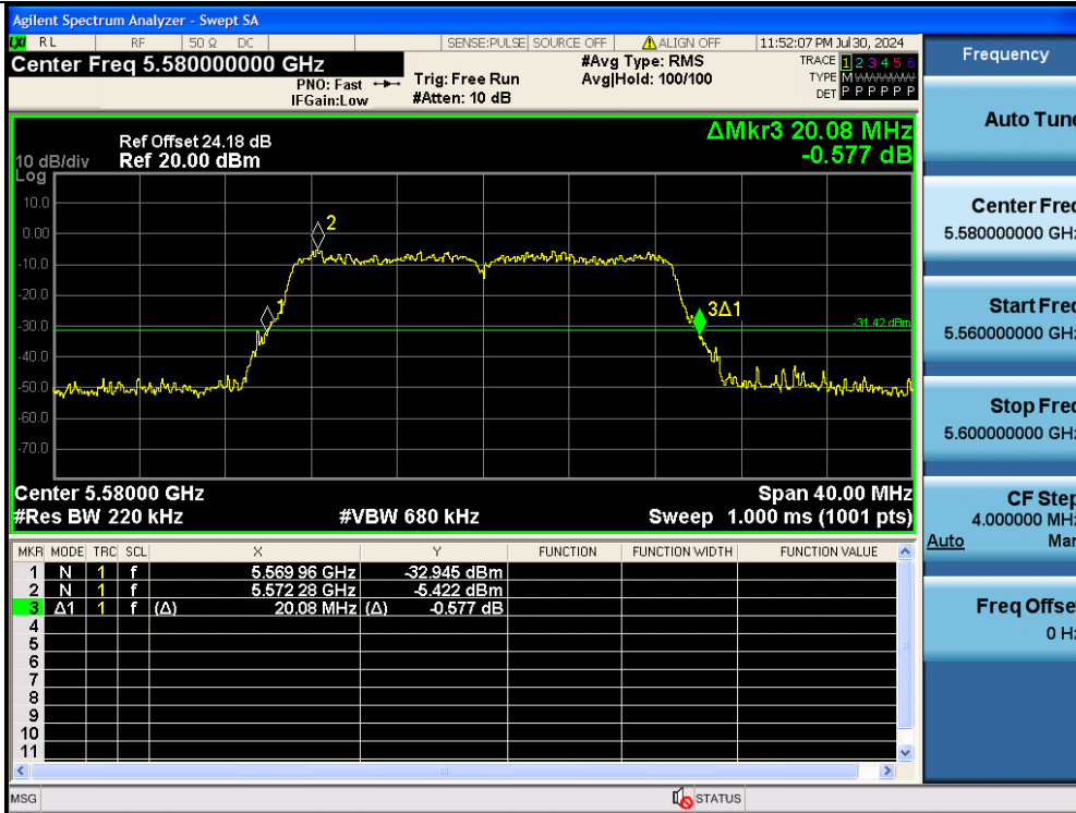
11N20MIMO-Ant2-5580
