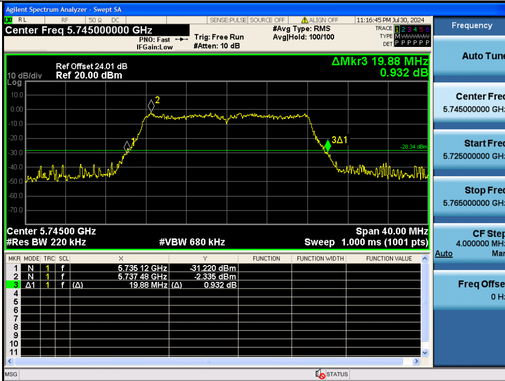
11A-Ant2-5745
