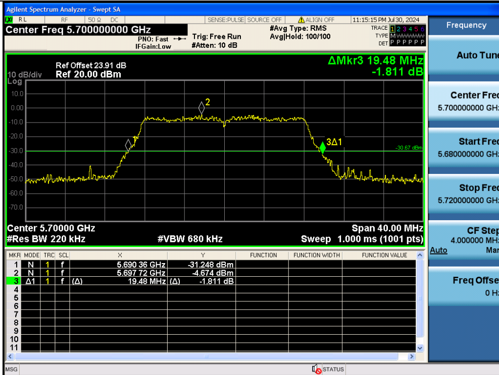
11A-Ant2-5700
