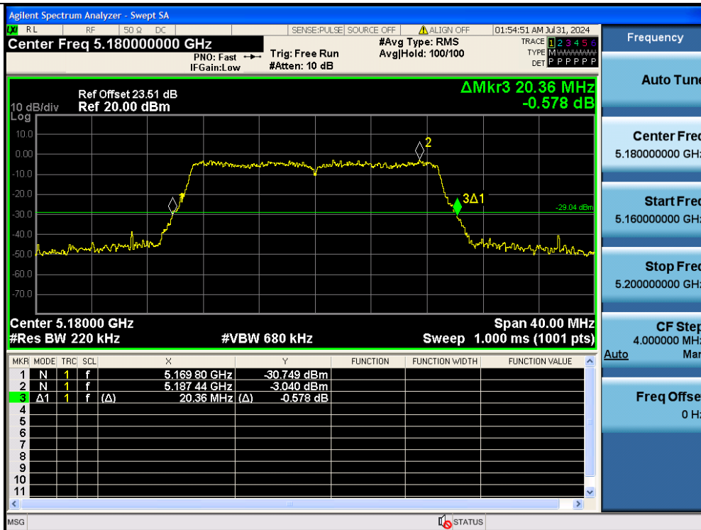
11AC20MIMO-Ant1-5180
