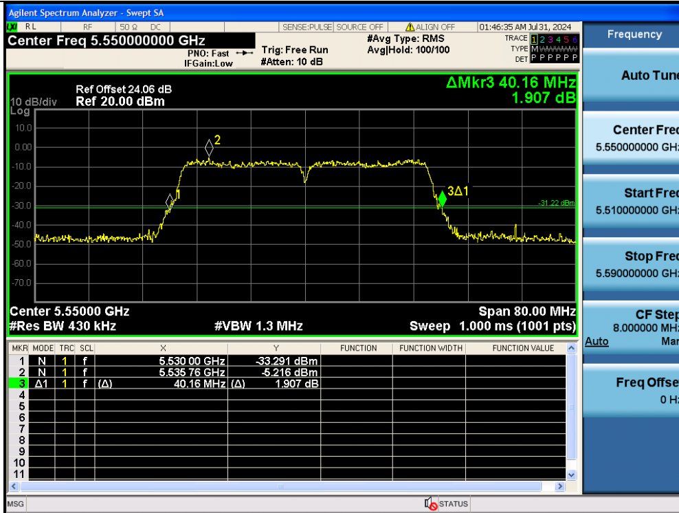
11N40MIMO-Ant2-5550
