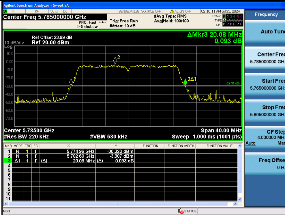
11AC20MIMO-Ant2-5785
