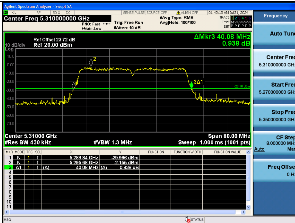
11N40MIMO-Ant2-5310
