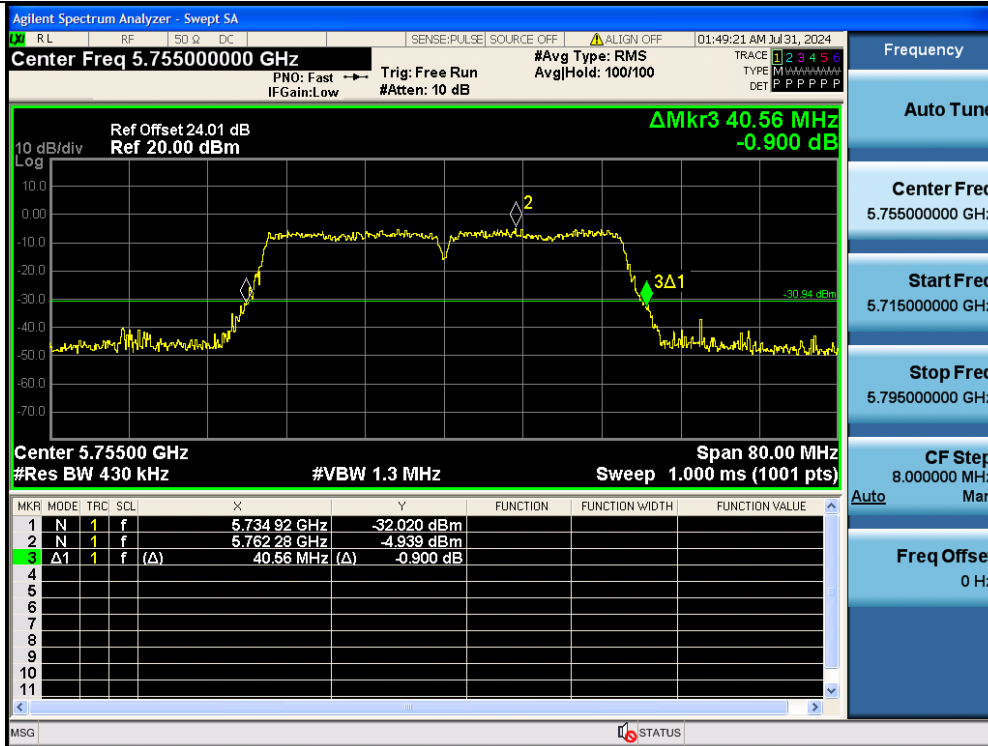
11N40MIMO-Ant2-5755
