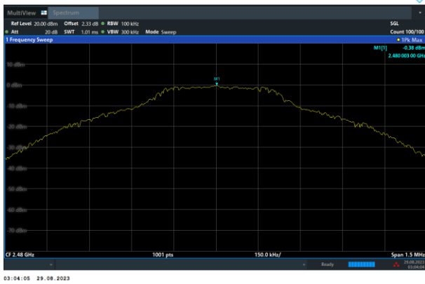
GFSK on Channel 78
