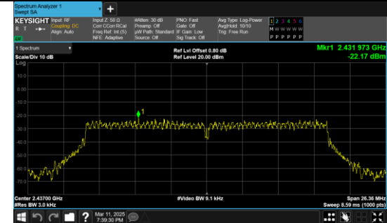
IEEE 802.11n Channel 6 20MHz Antenna 0
