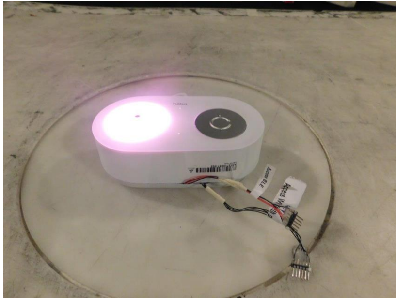
Below 1GHz Radiated Test Setup
