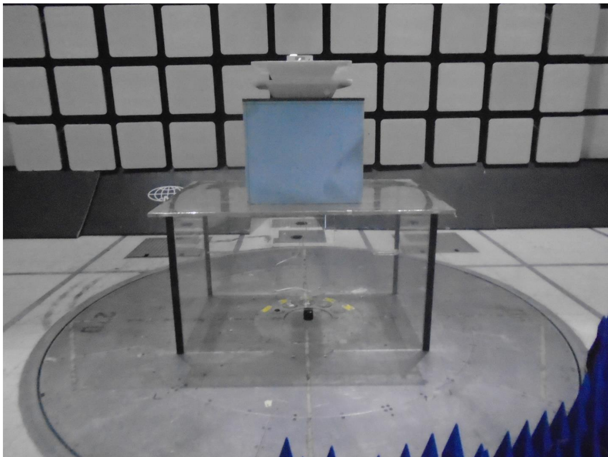
1GHz – 40GHz Radiated Emissions (Front Side)
