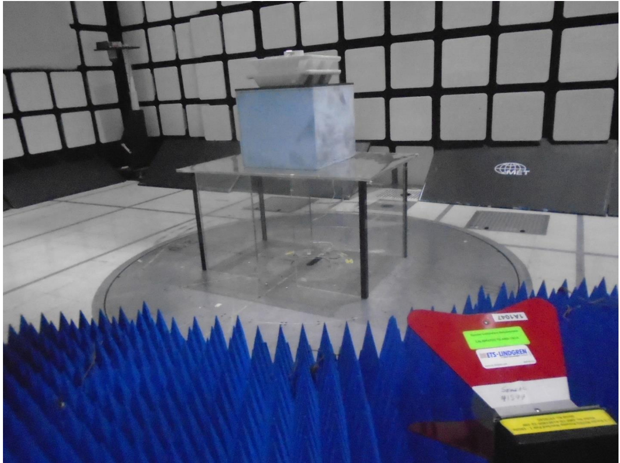
Radiated Emissions 1Ghz – 40GHz (Antenna View)
