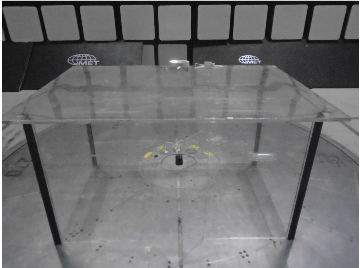
30MHz – 1GHz Radiated Emissions (Front Side)
