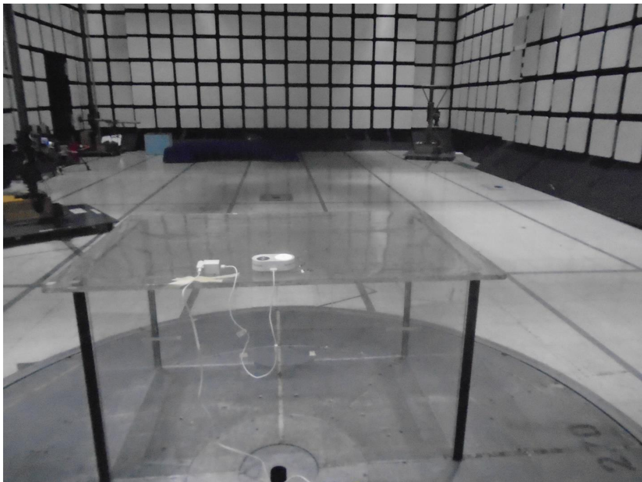
30MHz – 1GHz Radiated Emissions (Rear View)
