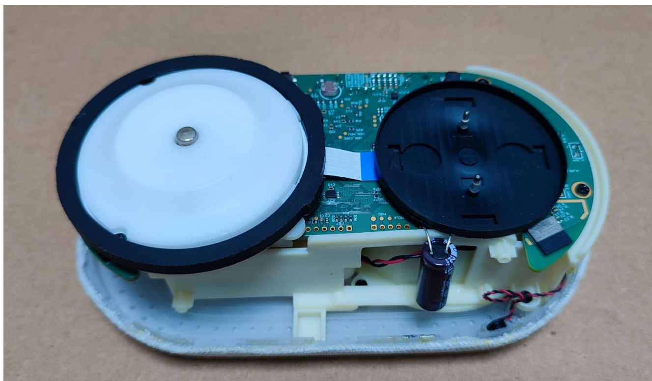
Hälsa Hub with Top Enclosure Removed
