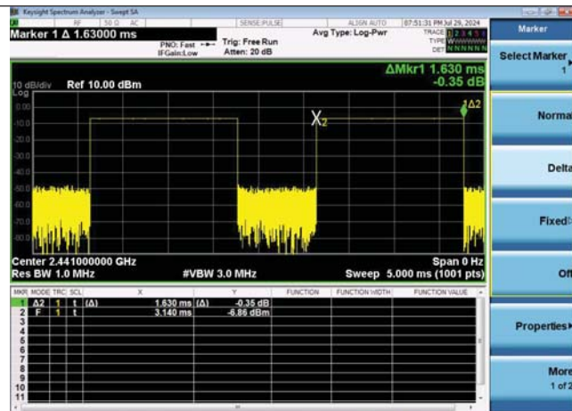
DH3 burst time
