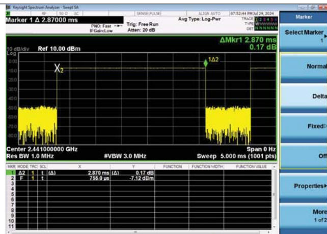
DH5 burst time
