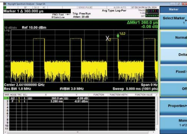
DH1 burst time
