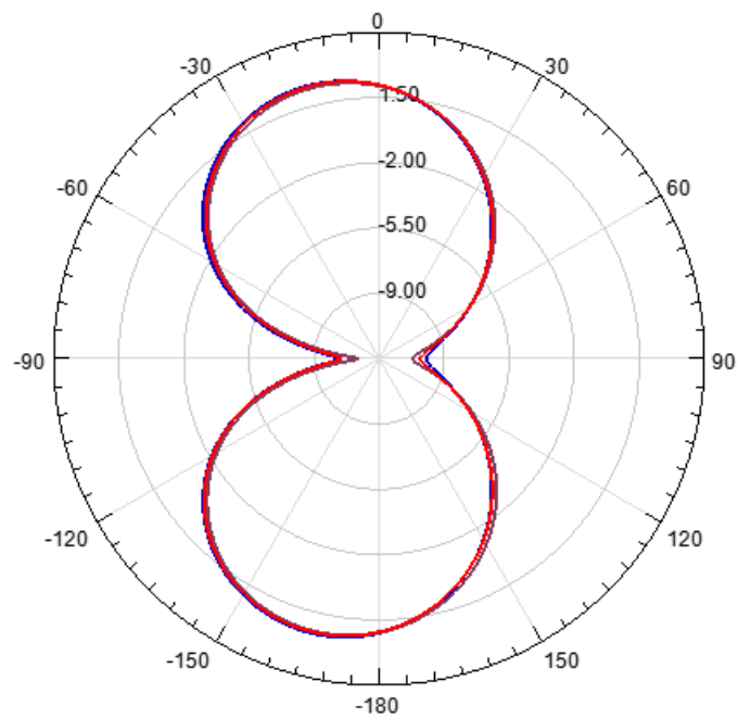
Radiation Pattern Y0
