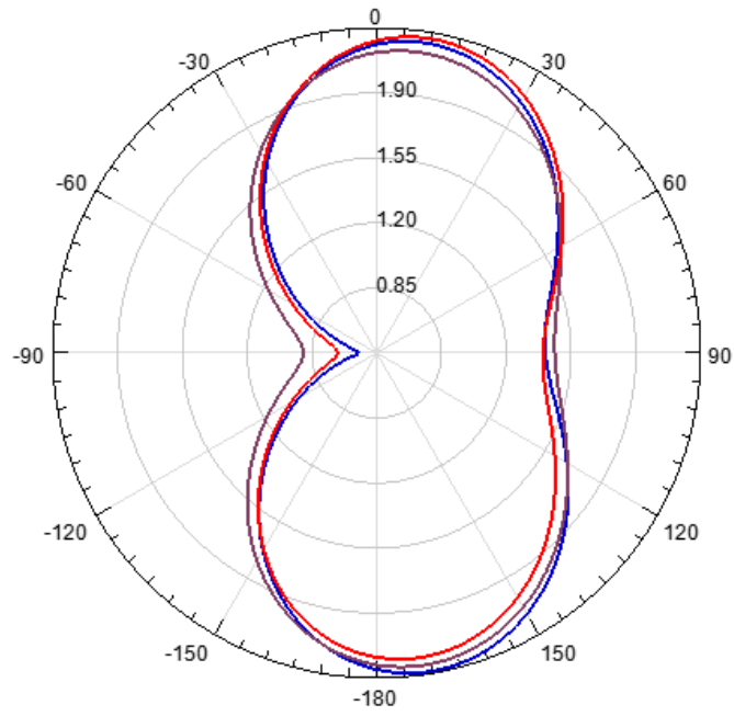
Radiation Pattern X0Z
