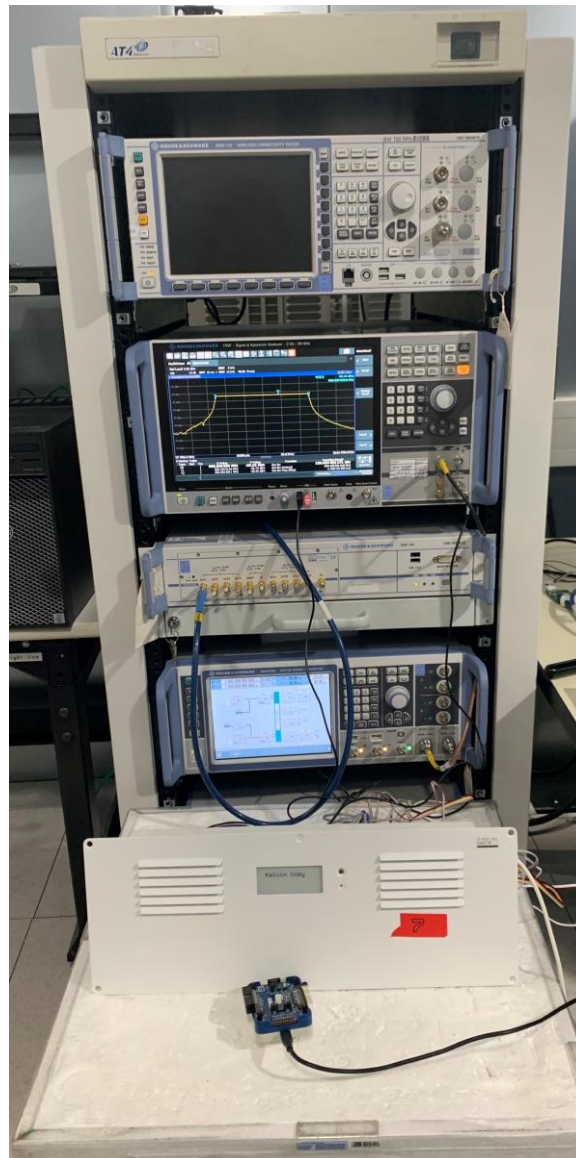
7. Conducted test setup
