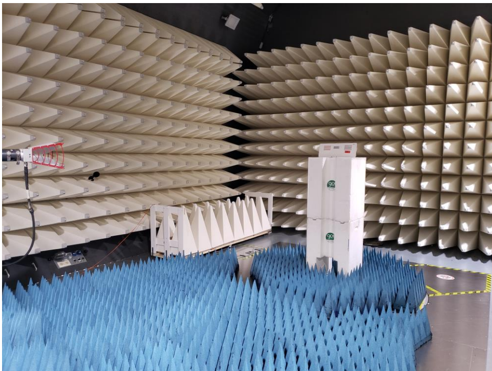
6. Radiated Emission test setup High Range
