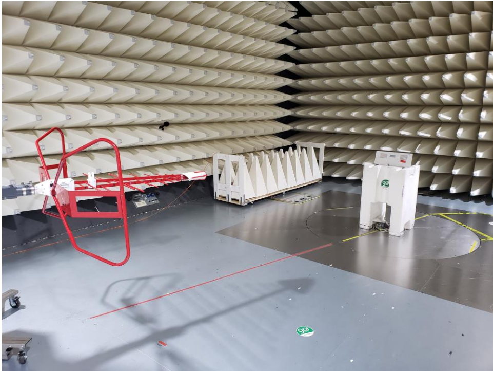
5. Radiated Emission test setup Low Range
