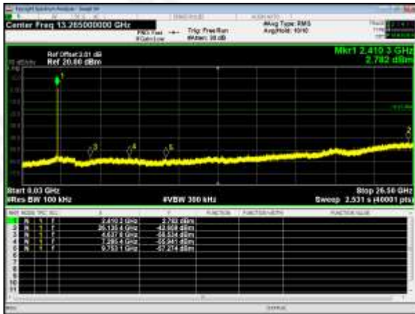
802.11b-Lowest channel
