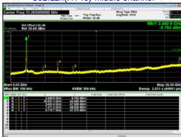
802.11n(HT40)-Middle channel
