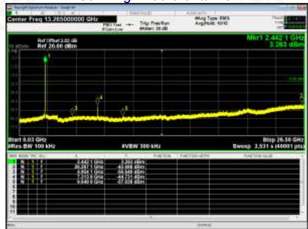
802.11g-Middle channel
