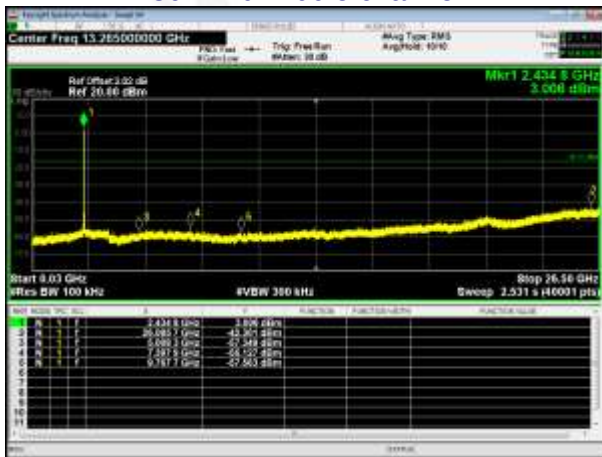
802.11b-Middle channel
