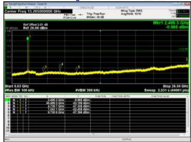
802.11g-Lowest channel
