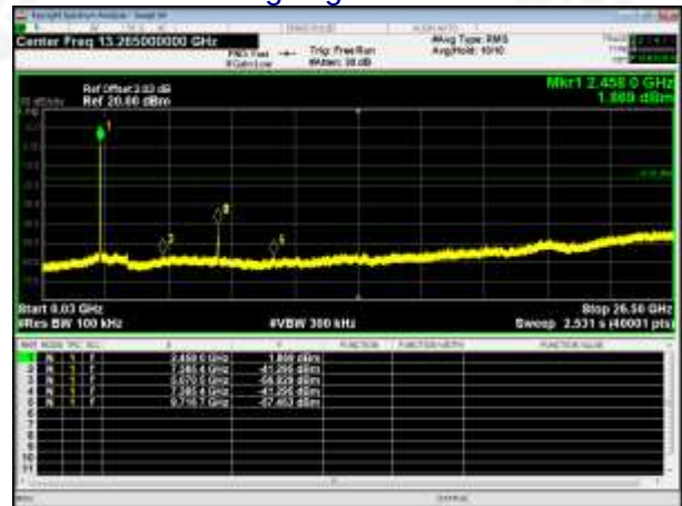
802.11g-Highest channel
