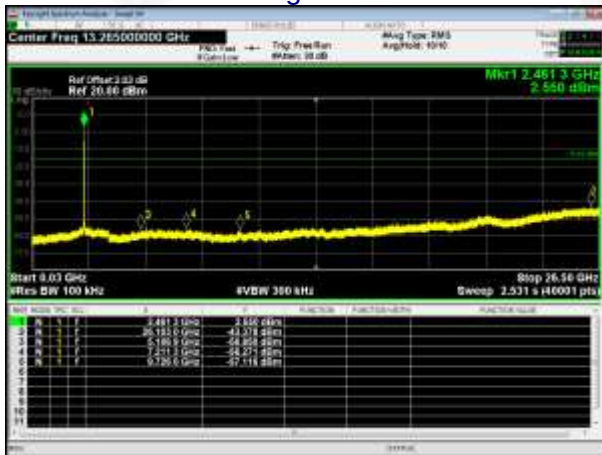
802.11b-Highest channel
