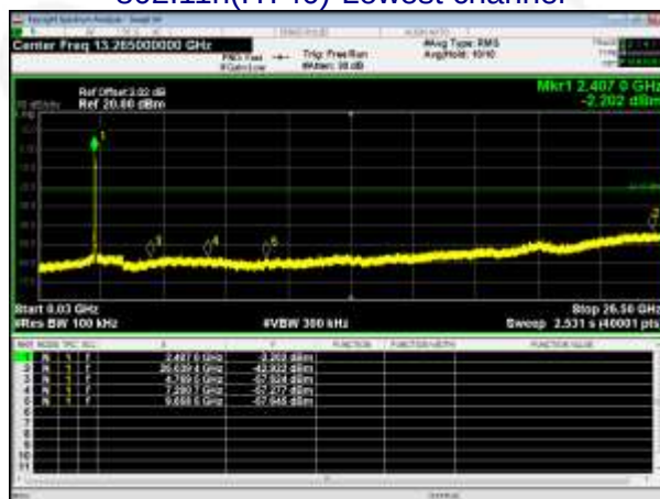
802.11n(HT40)-Lowest channel
