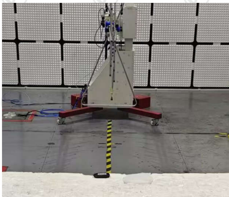
Radiated emission Test Setup-2 (30MHz~1GHz)Close up
