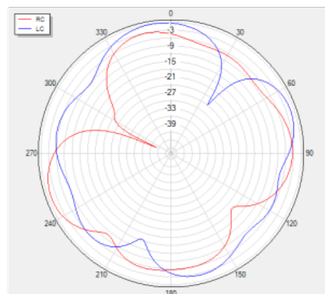
Theta=90 freq=2480MHz
