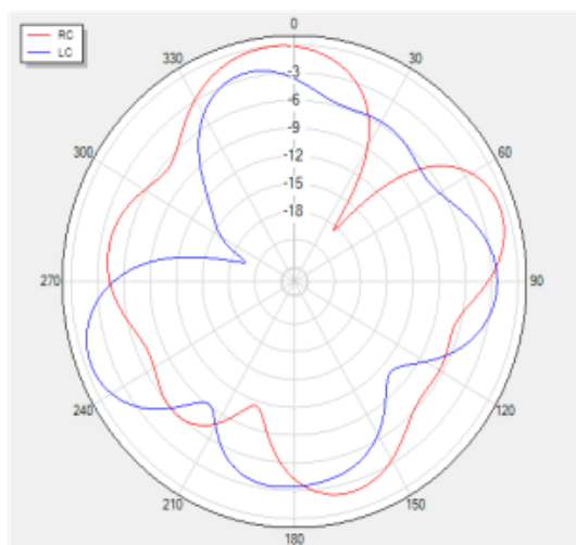
Theta=90 freq=2450MHz
