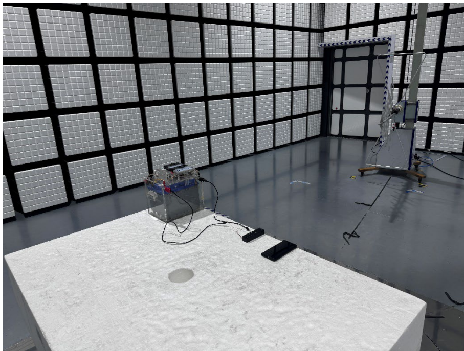
Description: Back view of Radiated Emission Test Setup (Below 1GHz) Mode 2
