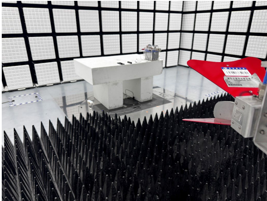
Description: Back view of Radiated Emission Test Setup (Above 1GHz) Mode 2
