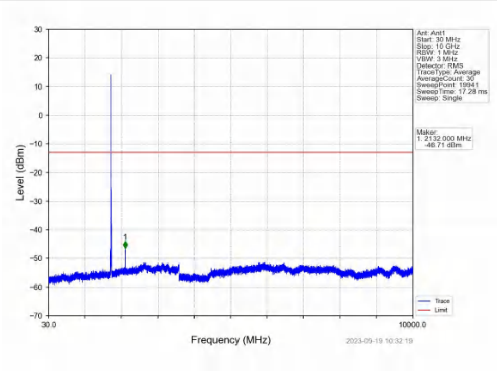
Band4_10MHz_QPSK_MCH_1732.5MHz_RB_1_0_NTNV
