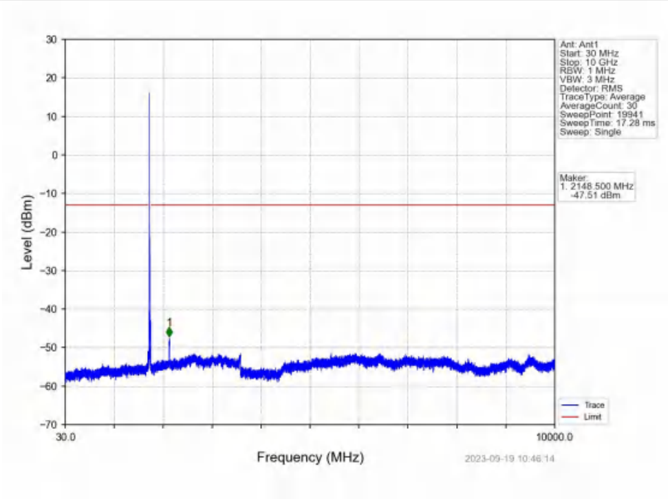
Band4_15MHz_16QAM_HCH_1747.5MHz_RB_1_0_NTNV
