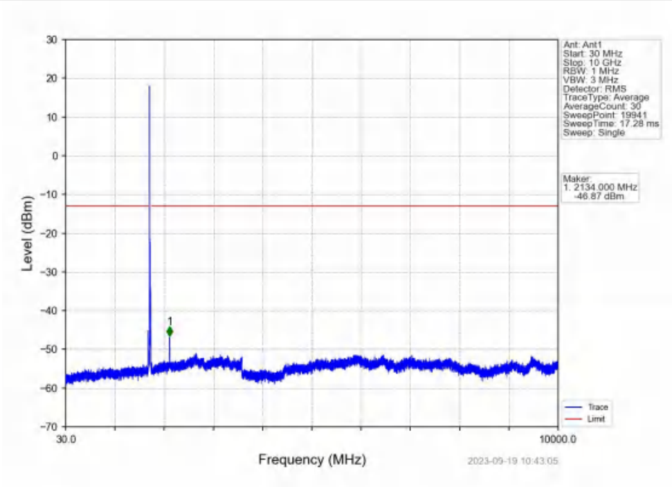
Band4_15MHz_16QAM_MCH_1732.5MHz_RB_1_0_NTNV
