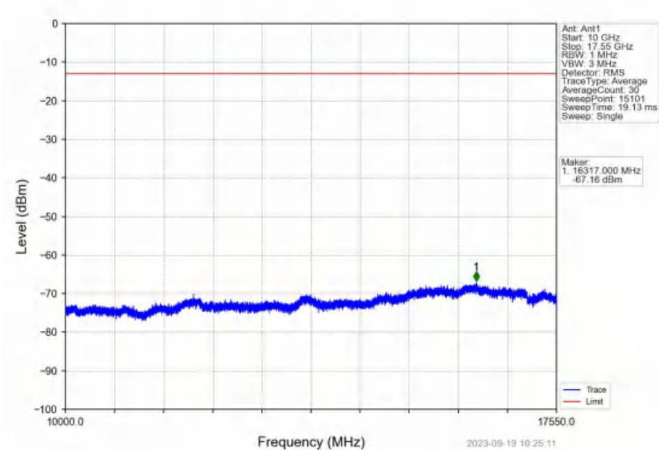
Band4_5MHz_16QAM_LCH_1712.5MHz_RB_1_0_NTNV
