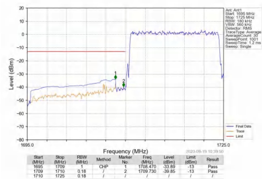
Band4_15MHz_QPSK_LCH_1717.5MHz_RB_75_0_NTNV
