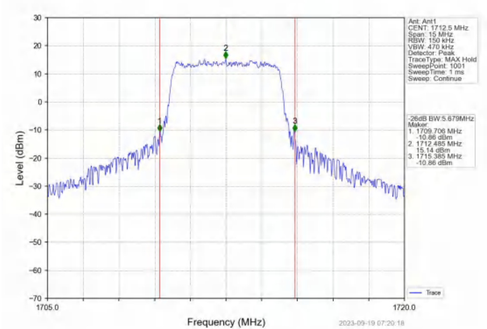
Band4_5MHz_16QAM_LCH_1712.5MHz_RB_25_0_NTNV
