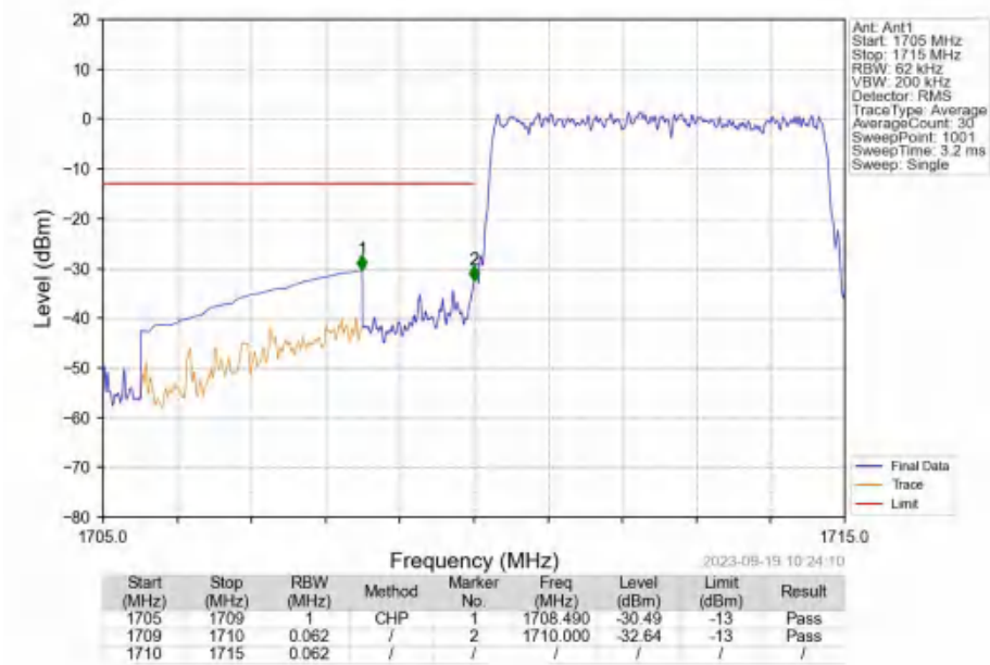
Band4_5MHz_QPSK_LCH_1712.5MHz_RB_25_0_NTNV
