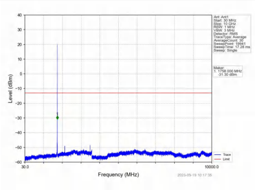
Band4_1.4MHz_QPSK_HCH_1754.3MHz_RB_1_0_NTNV
