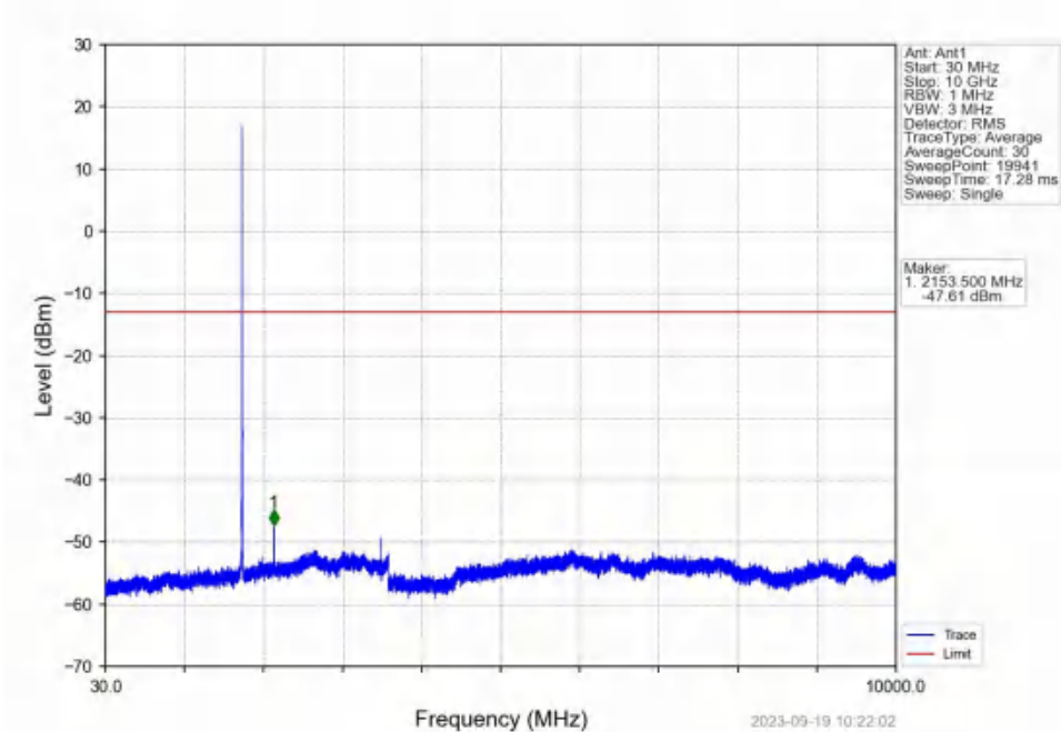
Band4_3MHz_16QAM_HCH_1753.5MHz_RB_1_0_NTNV
