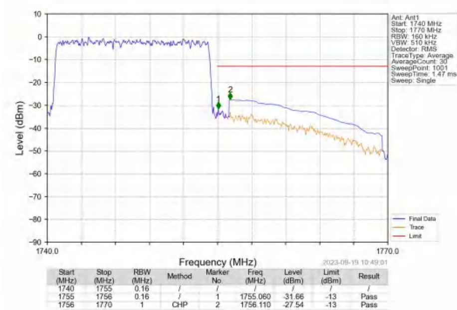
Band4_15MHz_16QAM_HCH_1747.5MHz_RB_75_0_NTNV
