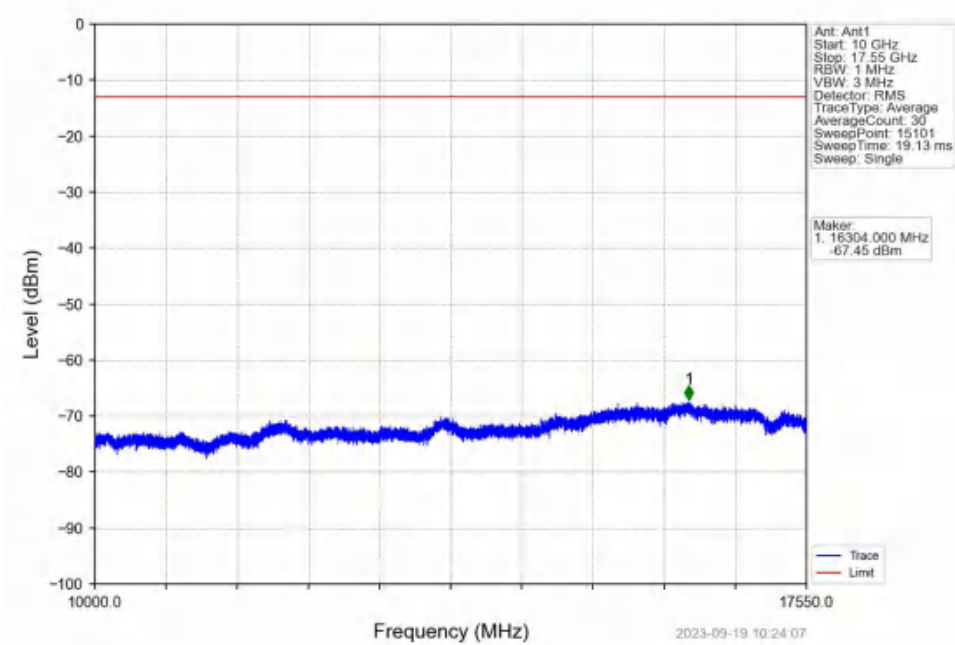
Band4_5MHz_QPSK_LCH_1712.5MHz_RB_25_0_NTNV
