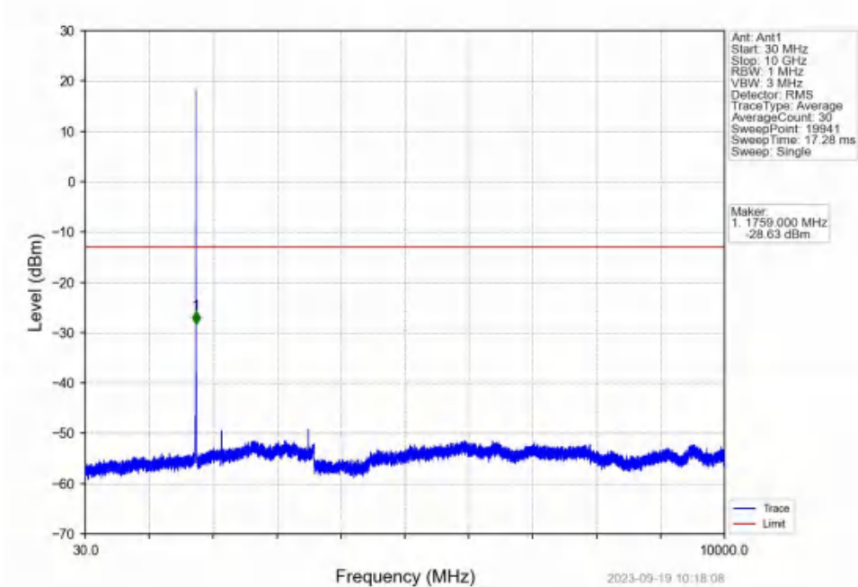
Band4_1.4MHz_16QAM_HCH_1754.3MHz_RB_1_0_NTNV
