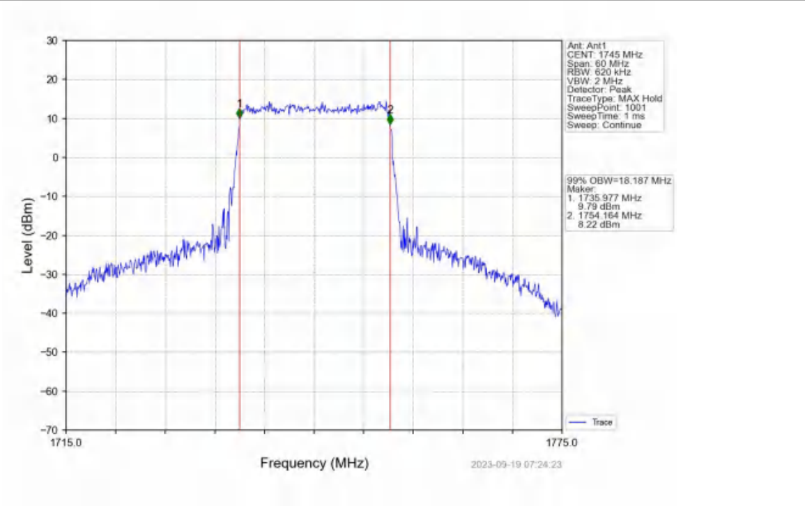
Band4_20MHz_16QAM_HCH_1745MHz_RB_100_0_NTNV
