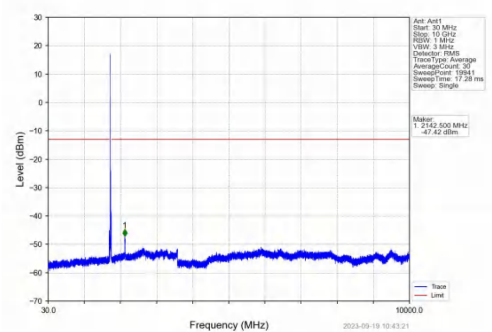
Band4_15MHz_QPSK_HCH_1747.5MHz_RB_1_0_NTNV
