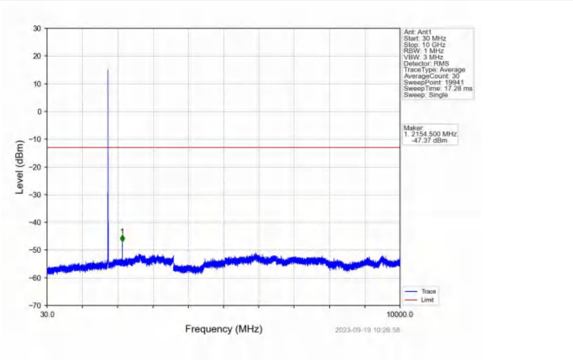
Band4_5MHz_16QAM_HCH_1752.5MHz_RB_1_0_NTNV
