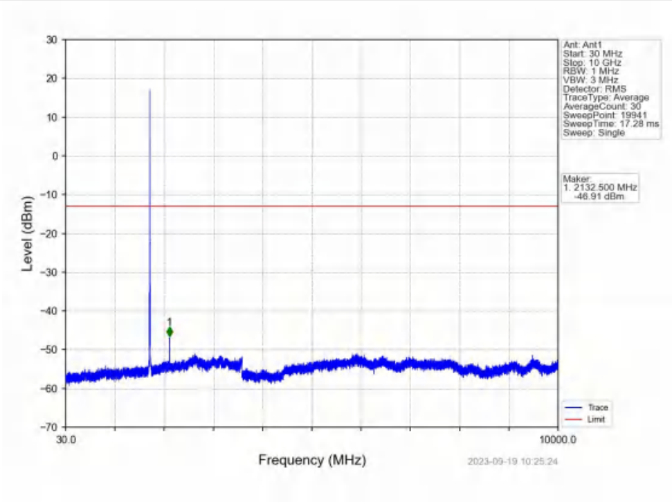
Band4_5MHz_QPSK_MCH_1732.5MHz_RB_1_0_NTNV
