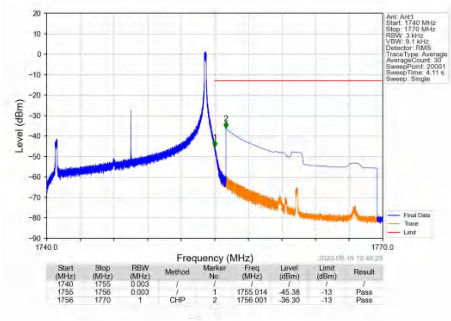
Band4_15MHz_16QAM_HCH_1747.5MHz_RB_1_74_NTNV
