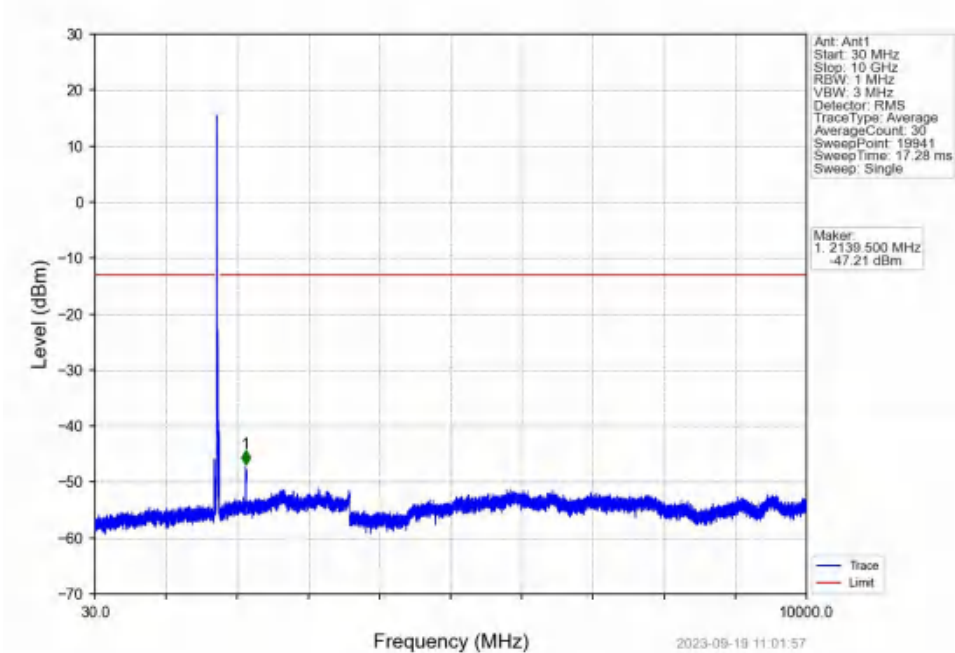
Band4_20MHz_16QAM_HCH_1745MHz_RB_1_0_NTNV
