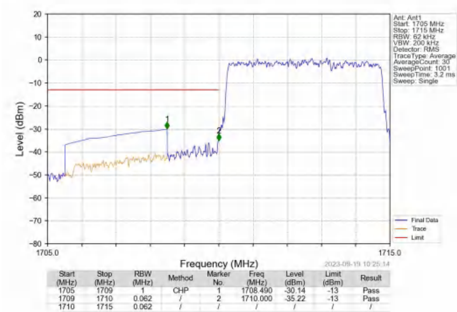
Band4_5MHz_16QAM_LCH_1712.5MHz_RB_25_0_NTNV
