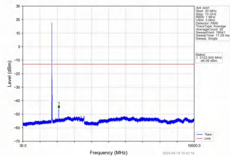
Band4_15MHz_16QAM_LCH_1717.5MHz_RB_1_0_NTNV
