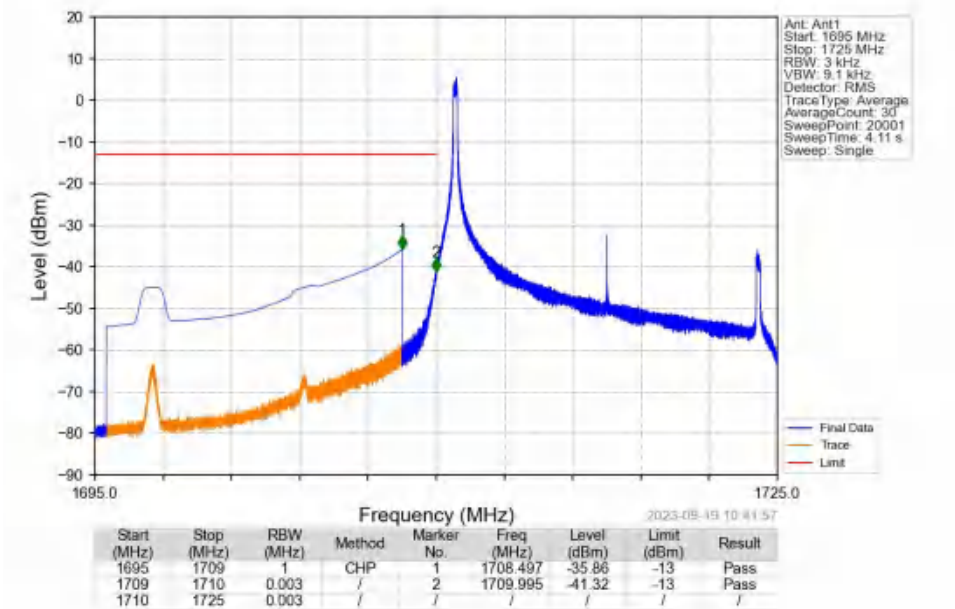
Band4_15MHz_16QAM_LCH_1717.5MHz_RB_1_0_NTNV
