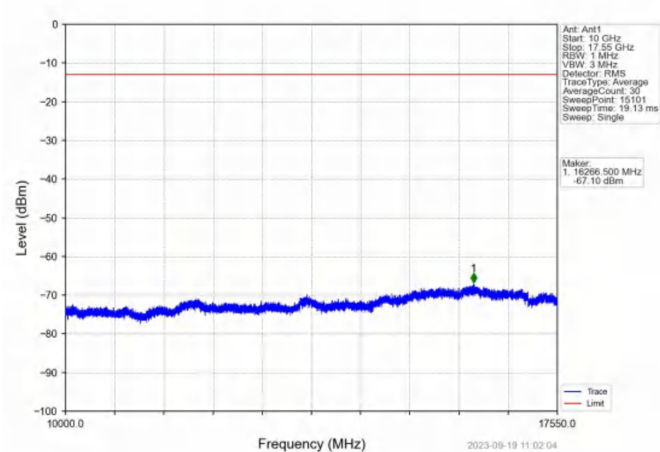
Band4_20MHz_16QAM_HCH_1745MHz_RB_1_0_NTNV
