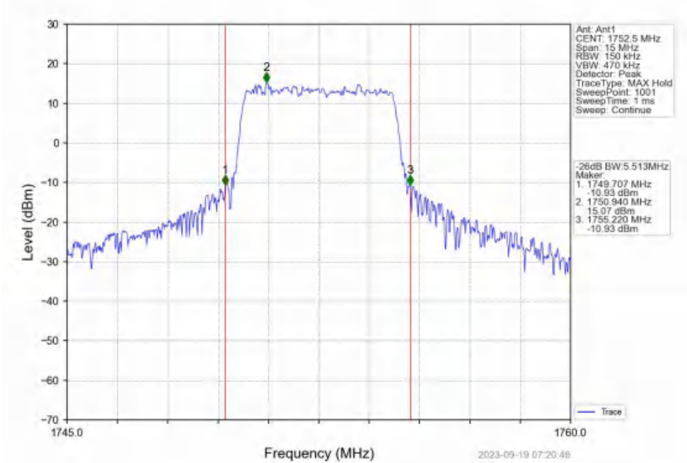
Band4_5MHz_QPSK_HCH_1752.5MHz_RB_25_0_NTNV
