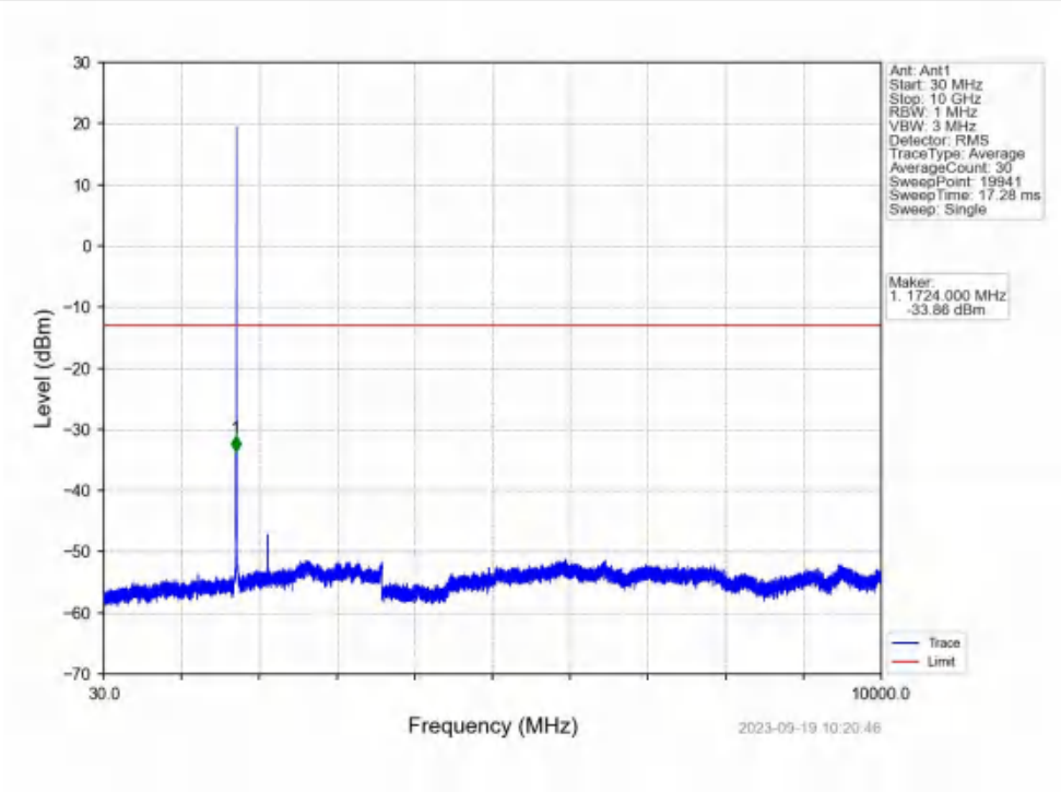
Band4_3MHz_QPSK_MCH_1732.5MHz_RB_1_0_NTNV
