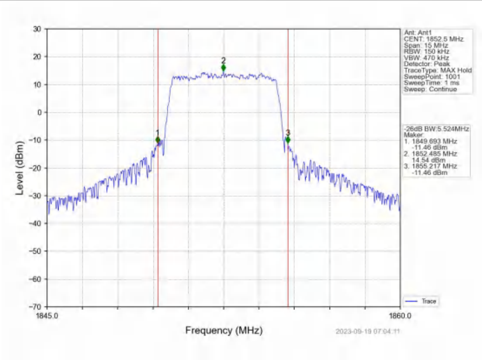
Band2_5MHz_16QAM_LCH_1852.5MHz_RB_25_0_NTNV
