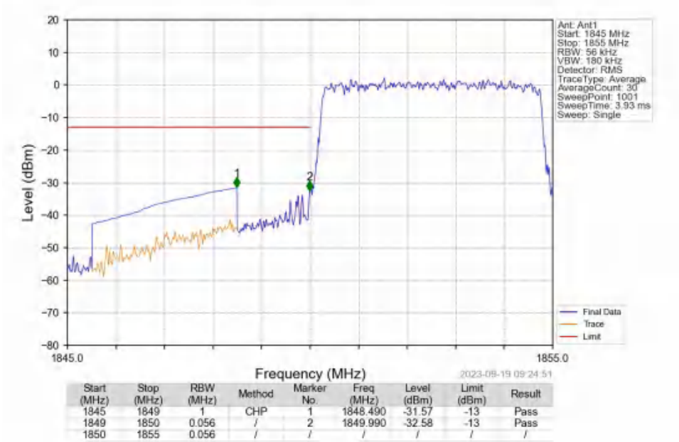
Band2_5MHz_16QAM_LCH_1852.5MHz_RB_25_0_NTNV
