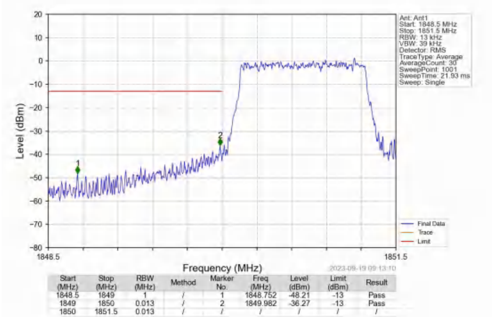
Band2_1.4MHz_QPSK_LCH_1850.7MHz_RB_6_0_NTNV
