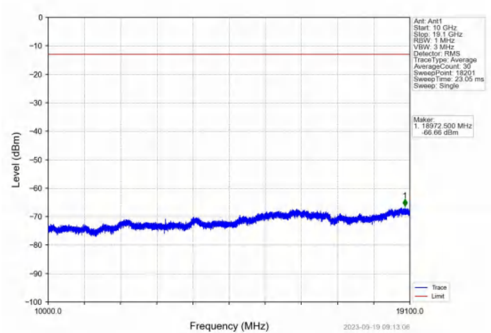
Band2_1.4MHz_QPSK_LCH_1850.7MHz_RB_1_0_NTNV
