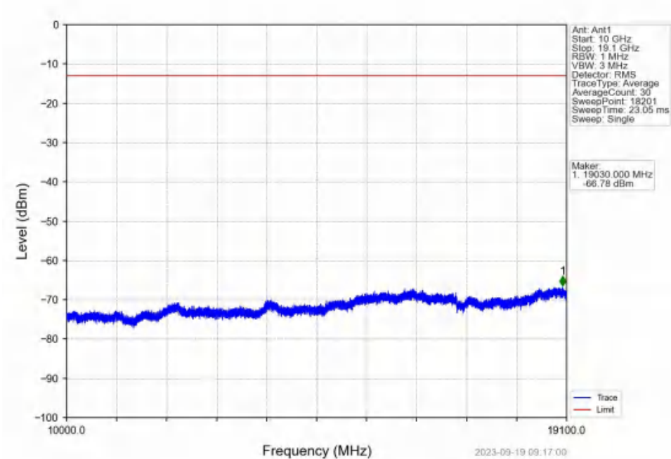
Band2_1.4MHz_16QAM_MCH_1880MHz_RB_1_0_NTNV
