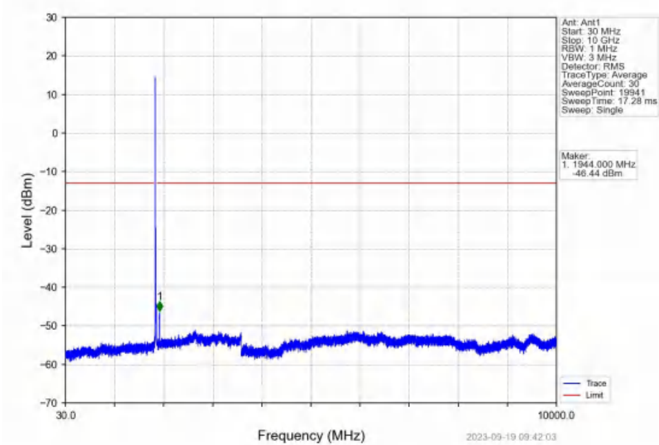
Band2_15MHz_16QAM_LCH_1857.5MHz_RB_1_0_NTNV
