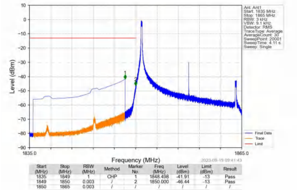
Band2_15MHz_16QAM_LCH_1857.5MHz_RB_1_0_NTNV
