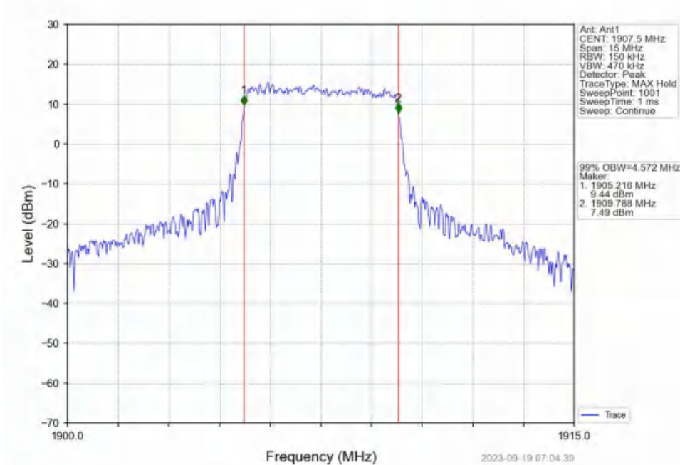
Band2_5MHz_QPSK_HCH_1907.5MHz_RB_25_0_NTNV
