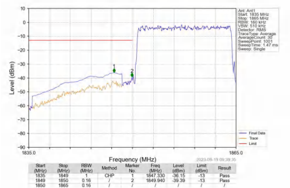
Band2_15MHz_QPSK_LCH_1857.5MHz_RB_75_0_NTNV
