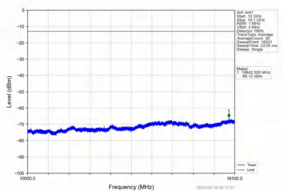
Band2_1.4MHz_16QAM_HCH_1909.3MHz_RB_1_0_NTNV
