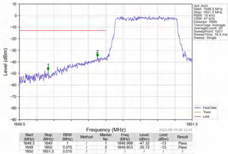
Band2 1.4MHz 16QAM LCH 1850.7MHz RB 6 0 NTNV
