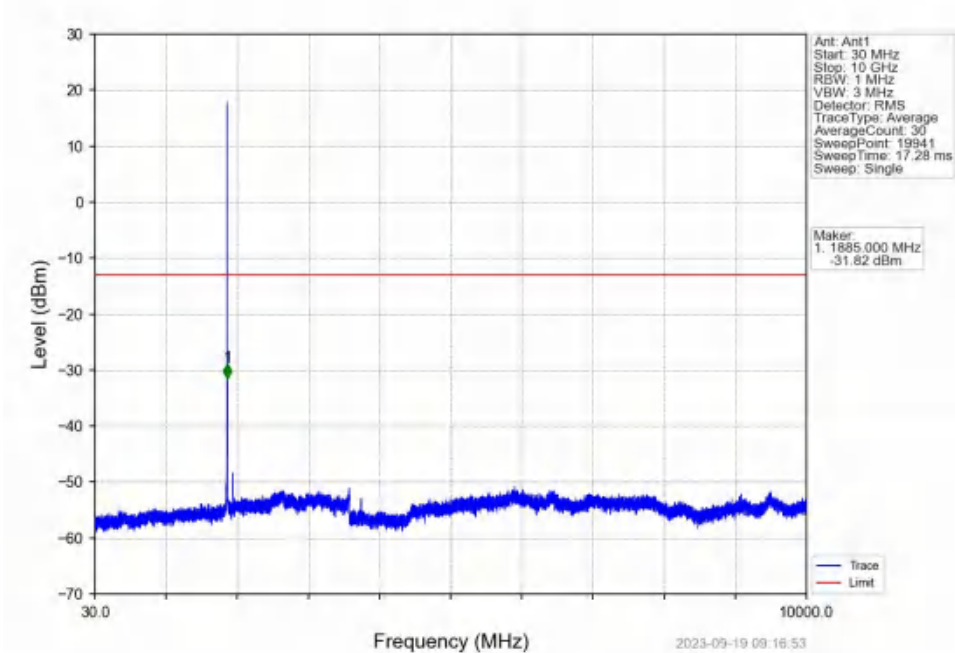
Band2_1.4MHz_16QAM_MCH_1880MHz_RB_1_0_NTNV
