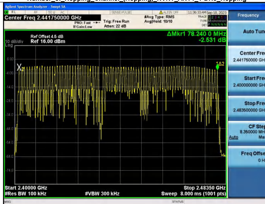
Number_of_Hopping_Channel (Hopping) NVNT ANT1 1-DH5 Hopping
