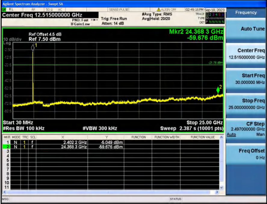
2_Spurious_Emissions_NVNT_ANT1_2-DH5_2402
