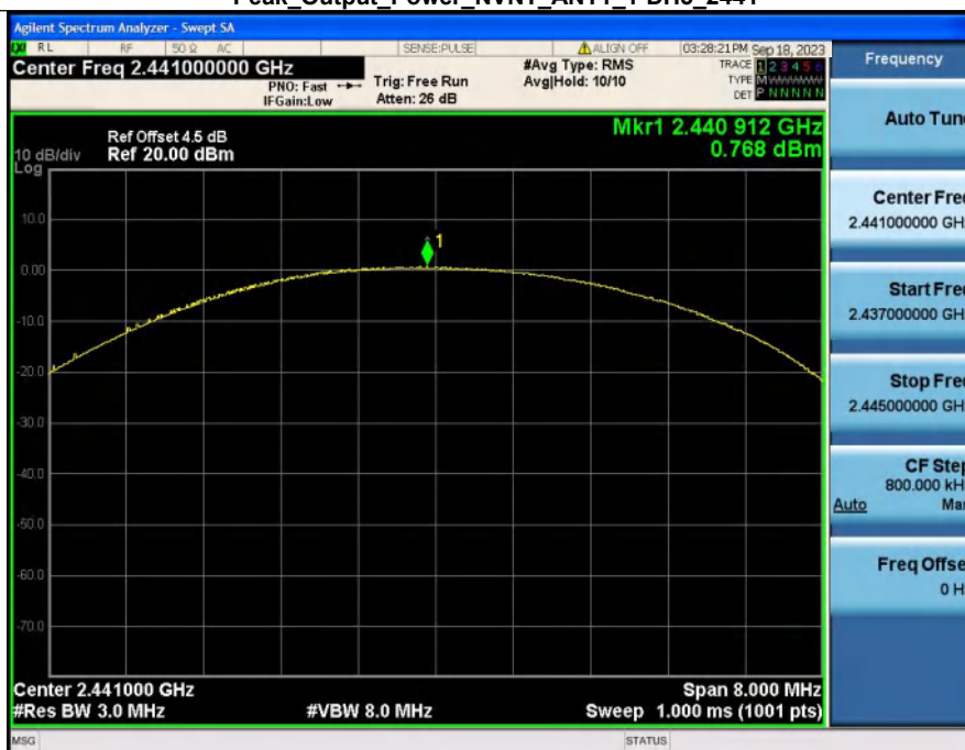
Peak_Output_Power_NVNT_ANT1_1-DH5_2441
