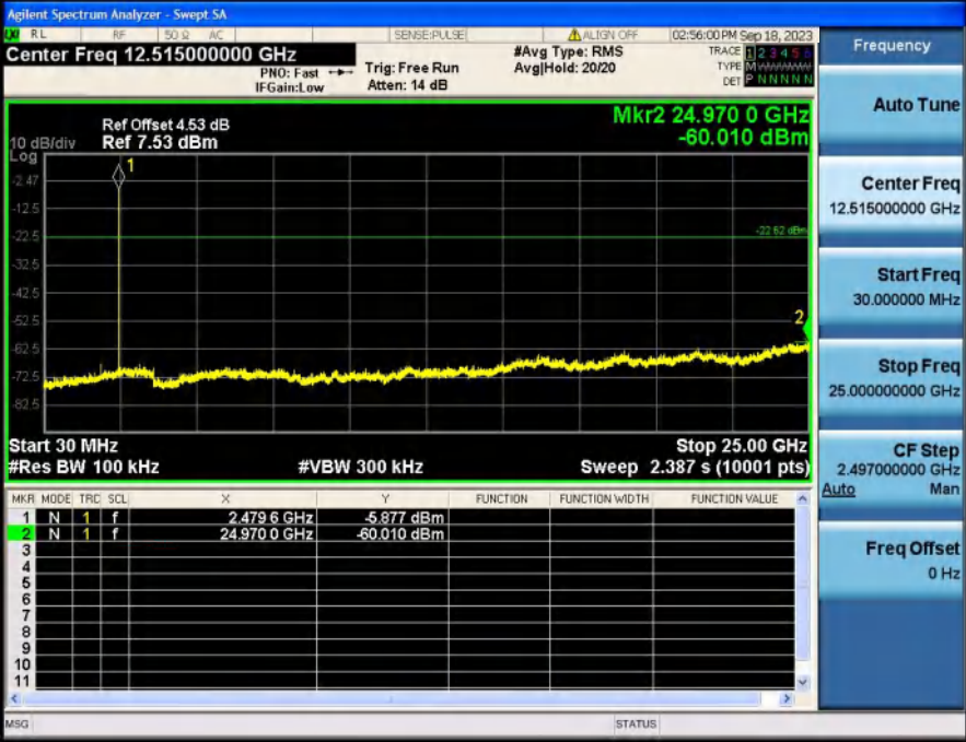
2_Spurious_Emissions_NVNT_ANT1_2-DH5_2480
