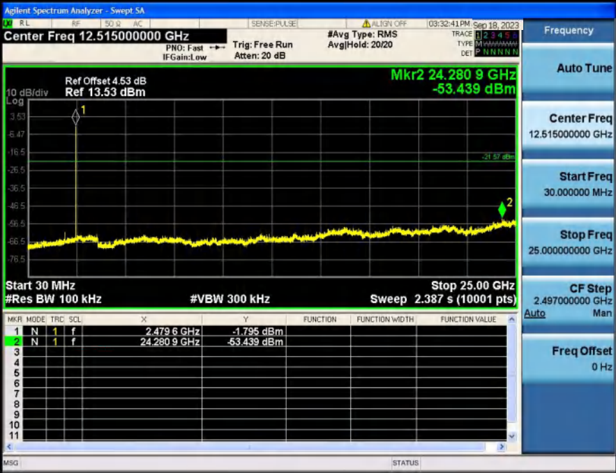
2_Spurious_Emissions_NVNT_ANT1_1-DH5_2480
