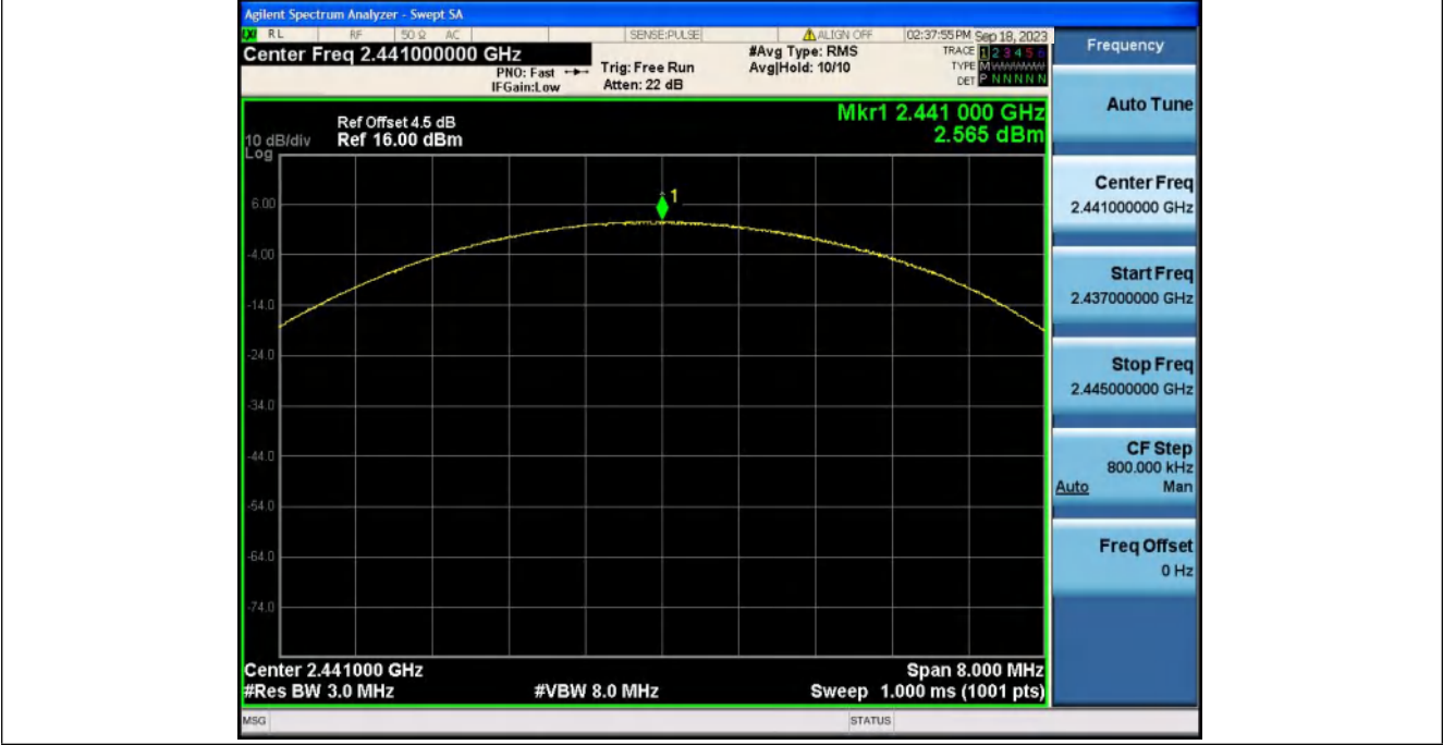
Peak_Output_Power_NVNT_ANT1_3-DH5_2441
