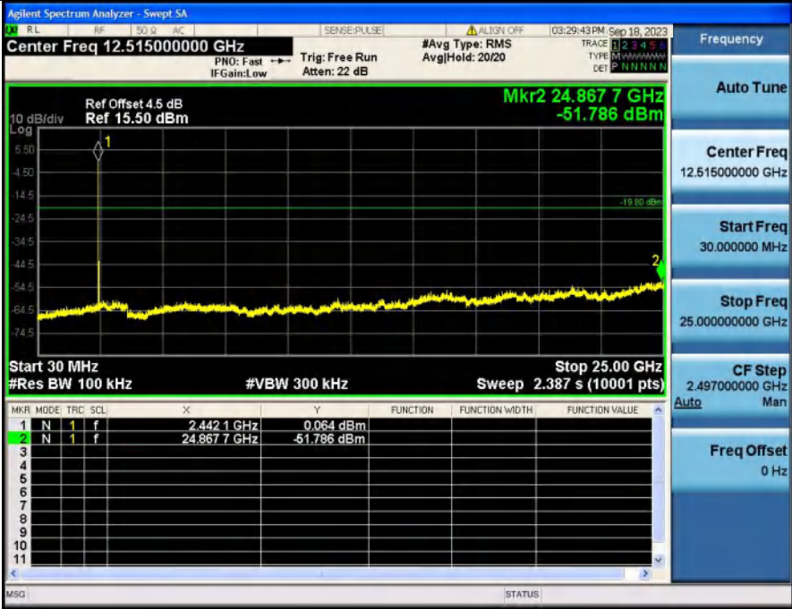
2_Spurious_Emissions_NVNT_ANT1_1-DH5_2441
