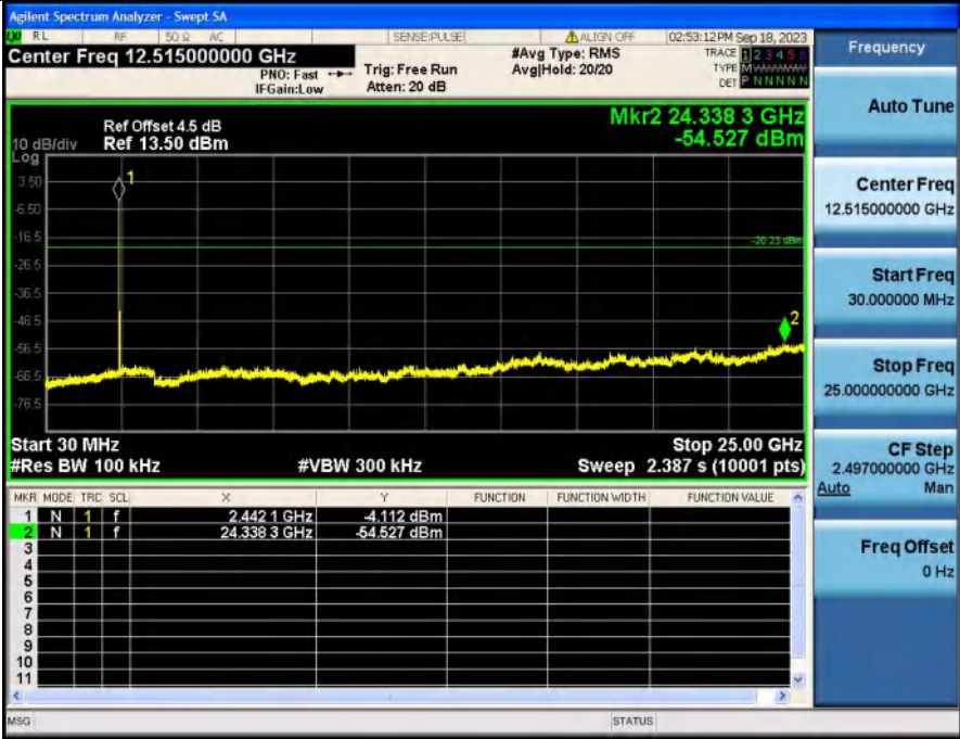
2_Spurious_Emissions_NVNT_ANT1_2-DH5_2441
