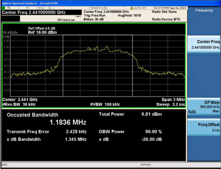
99%_Occupied_Bandwidth_NVNT_ANT1_3-DH5_2441
