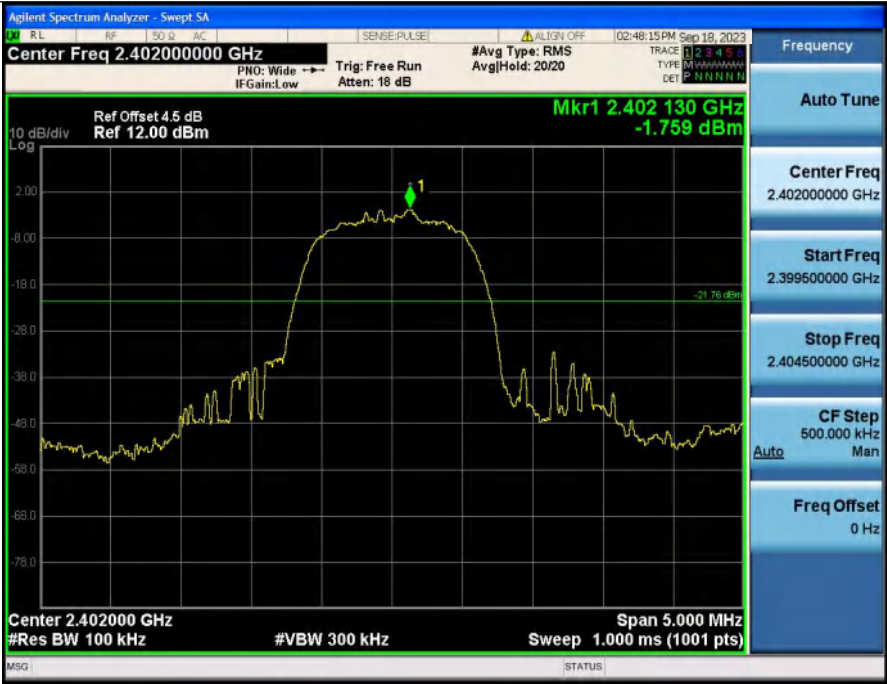
2_Spurious_Emissions_NVNT_ANT1_2-DH5_2402
