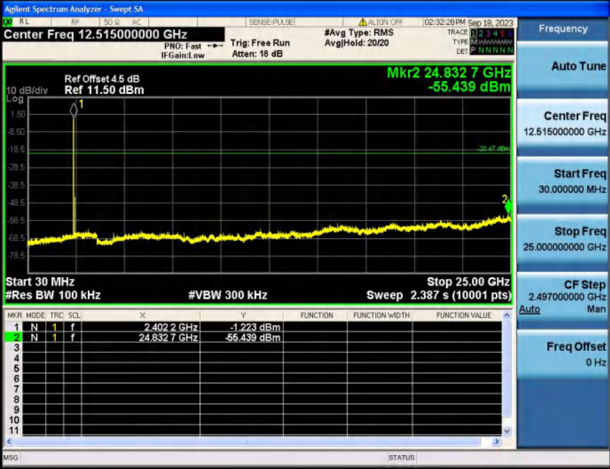
2_Spurious_Emissions_NVNT_ANT1_3-DH5_2402
