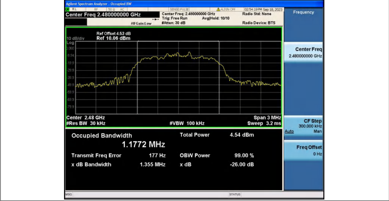
99%_Occupied_Bandwidth_NVNT_ANT1_2-DH5_2480
