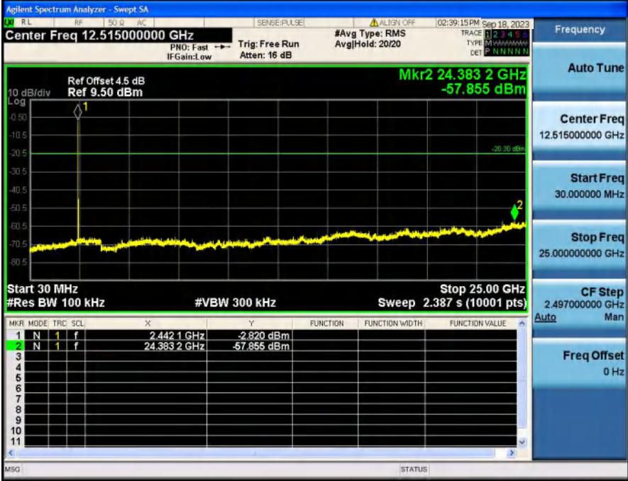
2_Spurious_Emissions_NVNT_ANT1_3-DH5_2441
