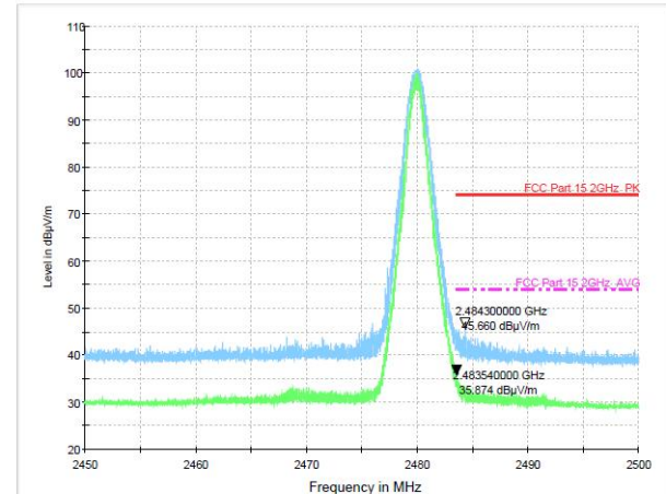
Test Mode: 8DPSK-High
