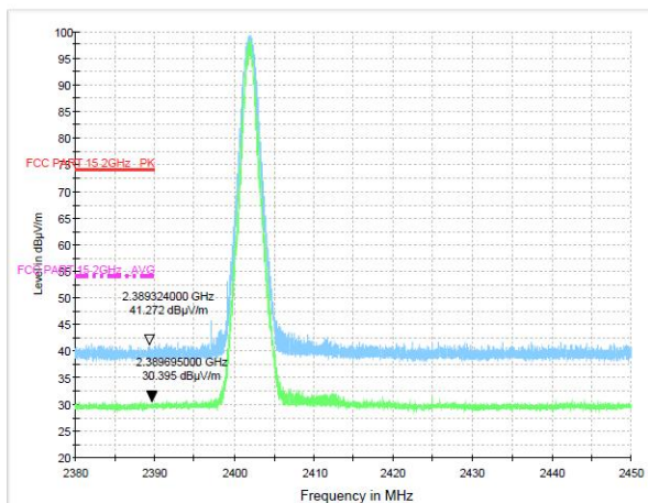
Test Mode: 8DPSK-Low
