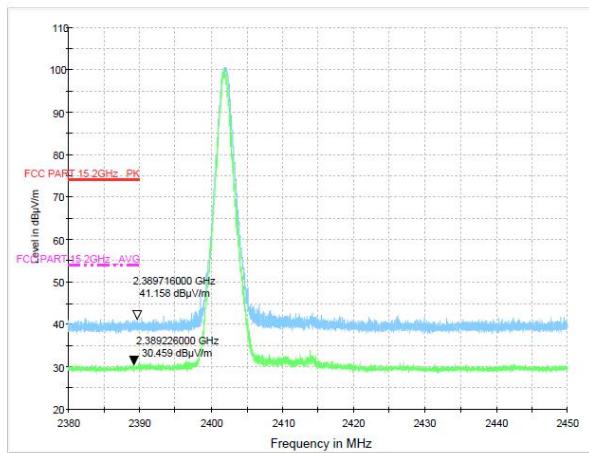
Test Mode: \pi/4 DQPSK-Low
