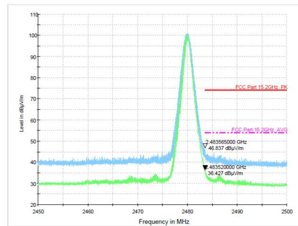
Test Mode: \pi/4 DQPSK-High
