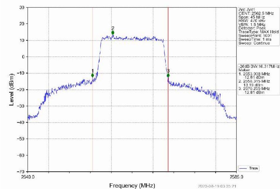
Band7_15MHz_16QAM_HCH_2562.5MHz_RB_75_0_NTNV
