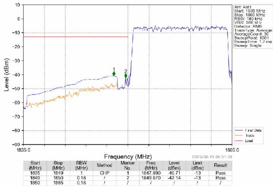
Band2_15MHz_16QAM_LCH_1857.5MHz_RB_75_0_NTNV
