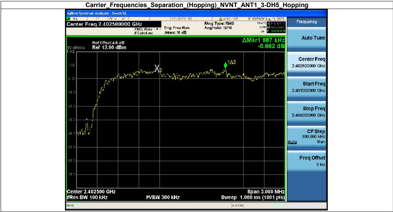
Carrier_Frequencies_Separation_(Hopping)_NVNT_ANT1_3-DH5_Hopping
